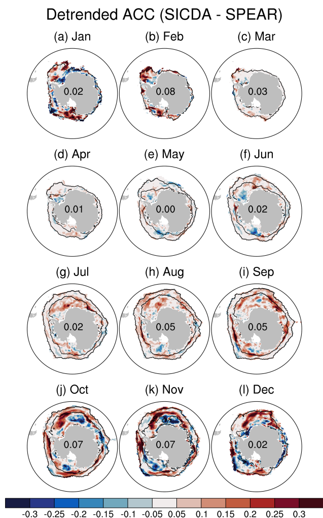
Figure 8. Difference in the 45-forecast-day mean of the detrended SIC ACC between the two reforecast experiments (SICDA – SPEAR). The black lines on each map represent the observed 10 % SIC interannual variability zone. The numbers on each map are the area-weighted average of the ACC difference within the SIC variability zone.
