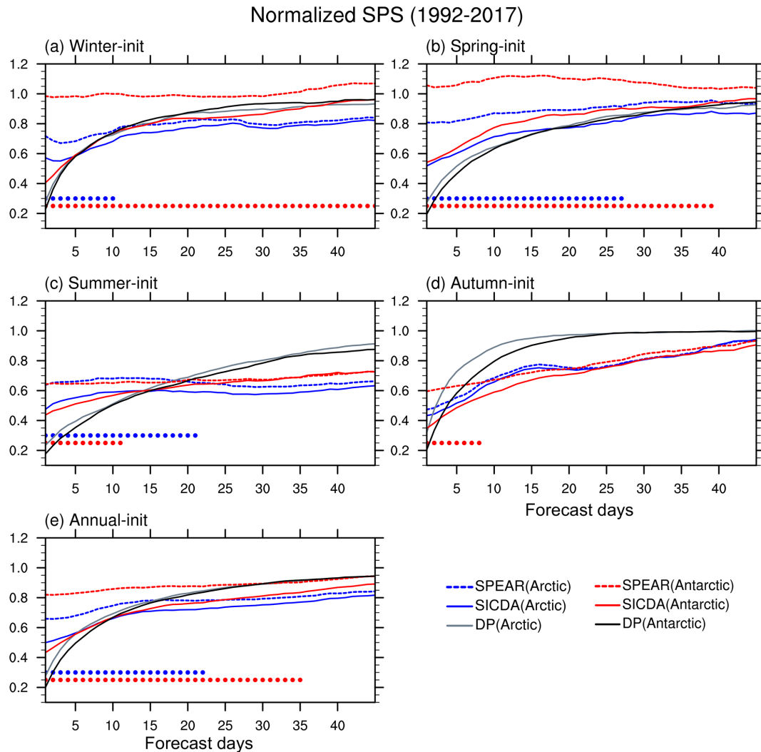
Figure 10. Normalized SPS calculated over the Antarctic as a function of forecast days for SPEAR (red dashed lines), SICDA (red solid lines) and DP (black lines), and over the Arctic for SPEAR (blue dashed lines), SICDA (blue solid lines) and DP (gray lines). The SPS values are normalized by the SPS values of the trend climatology forecast for each hemisphere. The normalized SPS values are calculated for each initialization month and then averaged over the (a) winter months, (b) spring months, (c) summer months, (d) autumn months, and (e) all 12 months. Each red filled circle on the bottom indicates that the SPS value from SICDA is lower than that of SPEAR at the 95 % significant level. The blue filled circles are for the Arctic.
