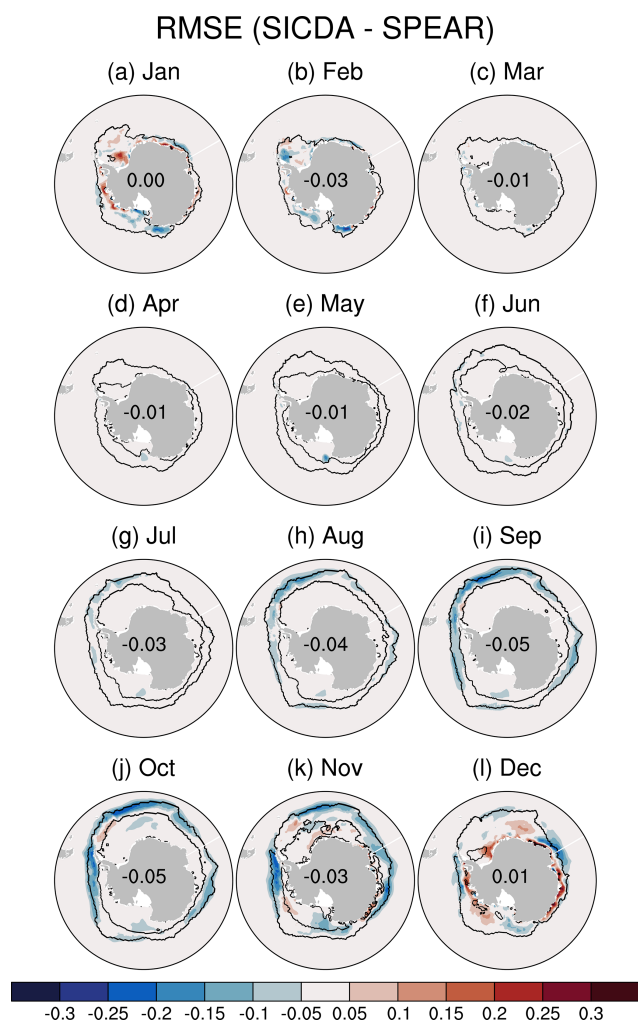
Figure 12. 45-forecast-day mean of the SIC RMSE difference between the two reforecast experiments (SICDA – SPEAR). The black lines on each map represent the 10 % SIC interannual variability zone. The numbers on each map are the area-weighted average of the RMSE difference within the 10 % SIC variability zone.
