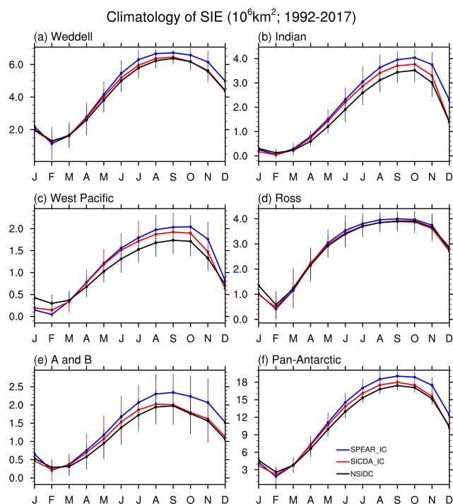
Figure 2. 26-year (1992–2017) mean seasonal cycle of regional and pan-Antarctic SIE for SPEAR_IC (blue), SICDA_IC (red), and the NSIDC observations (black). Each error bar represents two standard deviations of regional SIE calculated over the years.
