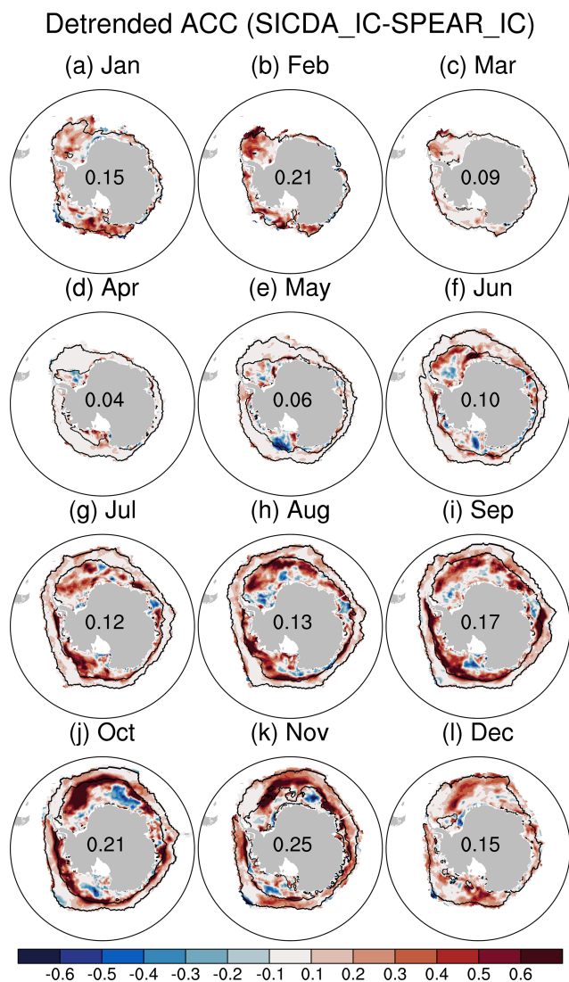
Figure 4. Difference in detrended SIC Anomaly Correlation Coefficient (ACC) between the two ICs (SICDA_IC – SPEAR_IC) for each month. The black lines on each map represent the observed 10 % SIC variability zone. The numbers on each map are the area-weighted average of the detrended ACC difference within the 10 % SIC variability zone.
