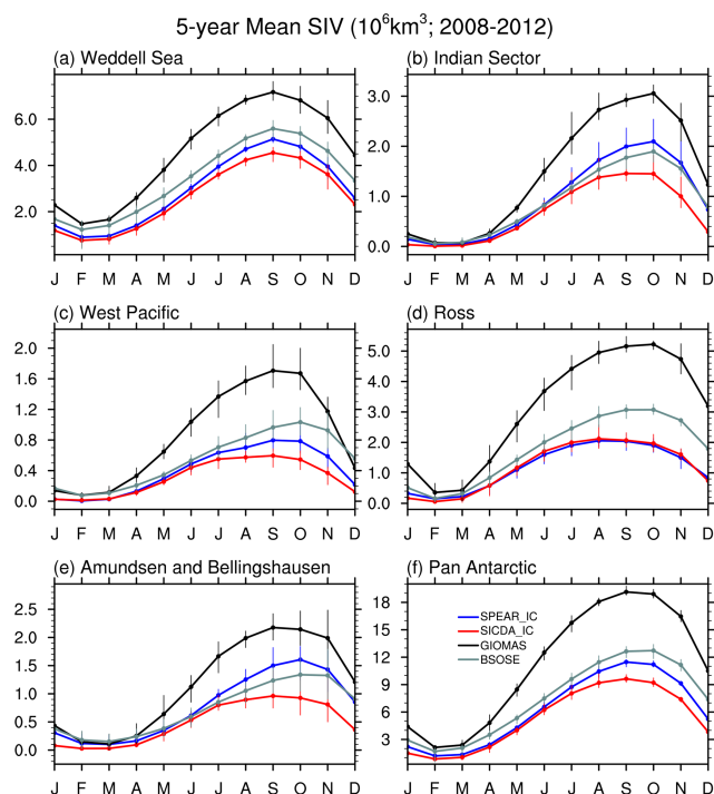
Figure 6. 5-year mean seasonal cycle of the regional and pan-Antarctic SIV from SPEAR_IC (blue), SICDA_IC (red), GIOMAS (black), and BSOSE (gray). The values are calculated over their overlapping years, 2008–2012. Each error bar represents the range of values across the years.
