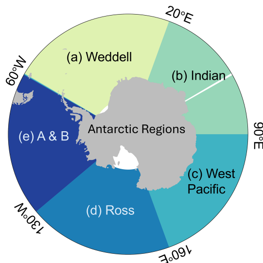
Figure 1. The Antarctic regions defined in this study. The longitude boundaries of the regions are: (a) 60° W–20° E for Weddell, (b) 20–90° E for Indian, (c) 90–160° E for West Pacific, (d) 160° E to 130° W for Ross, and (e) 130–60° W for Amundsen and Bellinghausen (A and B hereafter).
