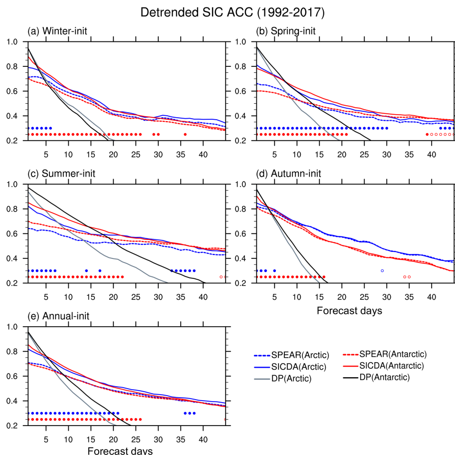
Figure 9. Detrended SIC ACC averaged over the Antarctic ice variability zone as a function of forecast days for SPEAR (red dashed lines), SICDA (red solid lines), and DP (black lines), and over the Arctic ice variability zone for SPEAR (blue dashed lines), SICDA (blue solid lines), and DP (gray lines). The Detrended ACC values are calculated for each initialization month and then averaged over the (a) winter months, (b) spring months, (c) summer months, (d) autumn months, and (e) all 12 months. Each red filled circle on the bottom indicates that the detrended ACC of SICDA is significantly higher than that of SPEAR, and red open circle the detrended SIC ACC of SICDA is 95 % significantly worse than that of SPEAR for the corresponding forecast day in the Antarctic. The blue filled circles and open circles are for the Arctic, respectively.
