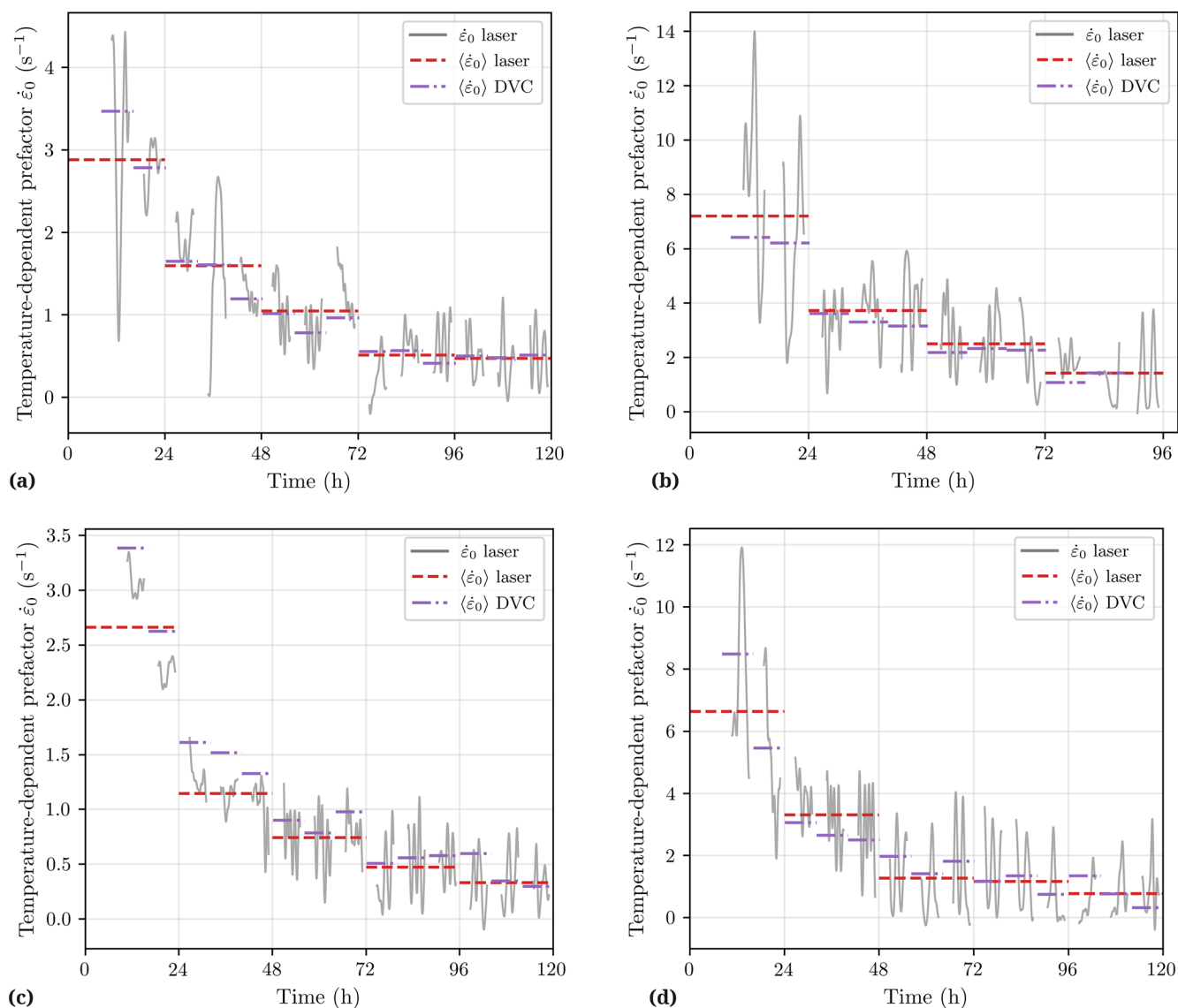
Figure A4. Temporal evolution of the strain rate prefactor \dot{\epsilon}_0 , computed from laser displacement measurements and DVC. (a) Sample 2, (b) Sample 3, (c) Sample 4, (d) Sample 5.
