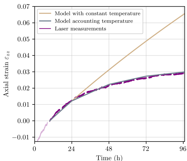
Figure 7. Strain versus time measured by the laser and predicted with the model Eq. (4) considering the measured temperature and a constant temperature equal to the initial temperature. The offset of the temperature prefactor is calibrated on the first temperature step. The first 8 h (grey area) are excluded from the analysis.
