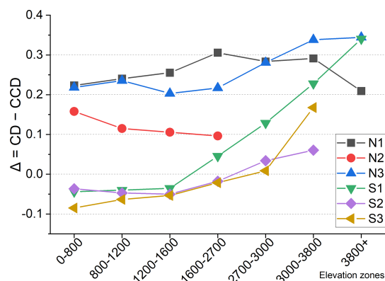
Figure 8. Elevation-dependent differences between coupling degree (CD) and coupling coordination degree (CCD) across the six sub-regions ( \Delta = \text{CD} - \text{CCD} ).
