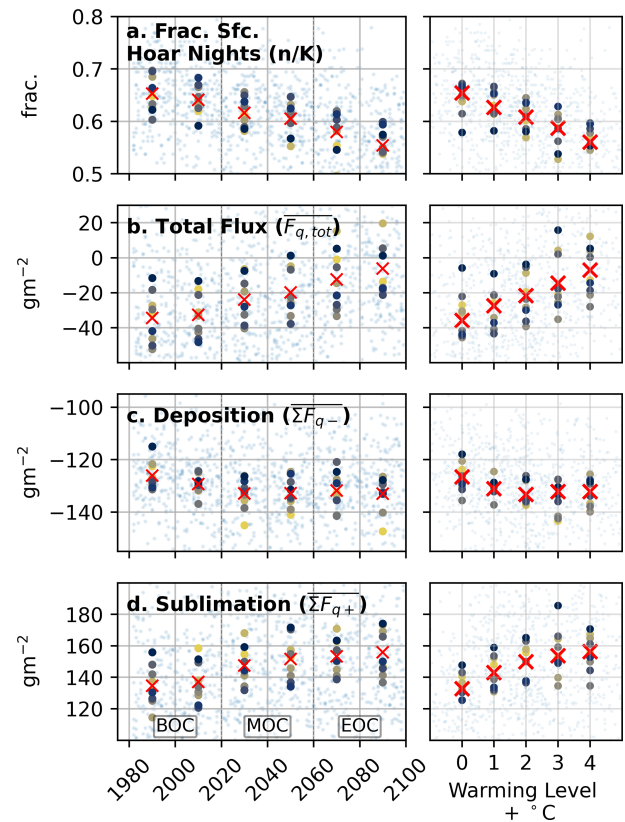
Figure 13. The same as Fig. 12, but for (a) The fraction of winter nights where the nightly cumulative \Sigma F_q is less than zero (i.e., surface hoar) per year, (b) the average mass of nightly total water vapor flux ( -F_{q,tot} ), (c) the average mass of nightly deposition events ( \Sigma F_{q,-} ), and (d) the average mass of nightly sublimation events ( \Sigma F_{q,+} ).
