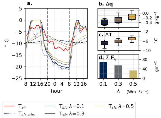
Figure 10. Sensitivity of surface hoar to prescribed values of snow thermal conductivity over a 36 h period characteristic of low ( \lambda = 0.1 ), medium ( \lambda = 0.3 ) and high-density ( \lambda = 0.5 ) snow: (a) Evolution of modeled T_{\text{sfc}} for varying \lambda values, with T_{\text{air}} (solid red line) and observed T_{\text{sfc}} (dotted line) included for comparison. Boxplots show (b) \Delta q , (c) \Delta T , and (d) overnight \Sigma F_q (between 08:00 pm to 08:00 am, depicted by dashed gray lines in a). The line colors in (a) correspond with the bar colors in (b)–(d).
