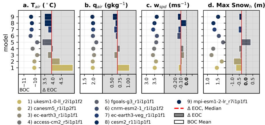
Figure 11. Effects of warming in the ERW across the 9 downscaled GCMs on (a) T_{air} , (b) q_{air} , (c) w_{spd} , and (d) maximum annual \text{Snow}_h . Left columns of each subplot depict the baseline beginning-of-century period winter nighttime average for each variable. Right columns depict the change at the EOC relative to the BOC. Red-lines depict the median change across all models for each variable.
