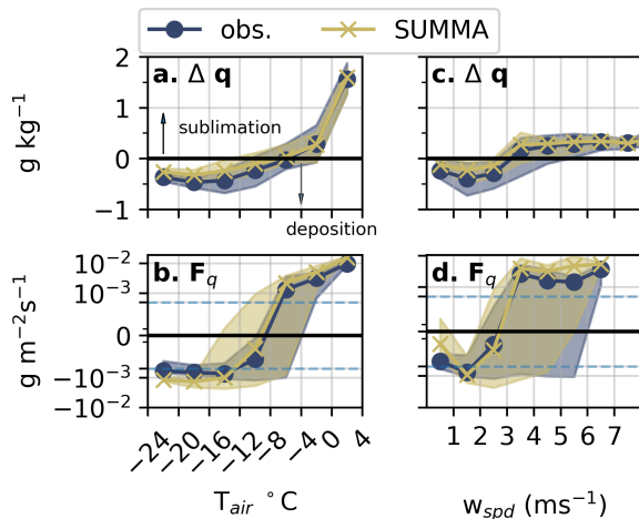
Figure 9. The sensitivity of overnight 30 min \Delta q and F_q to T_{\text{air}} (a, b) and w_{\text{spd}} (c, d) from both observations and SUMMA output expressed as bin-averages. Shaded regions depict the 25th and 75th percentile ranges within each bin. Note that the y-axes for (b) and (d) use a symmetric logarithmic scale, with a linear region between the blue dashed lines.
