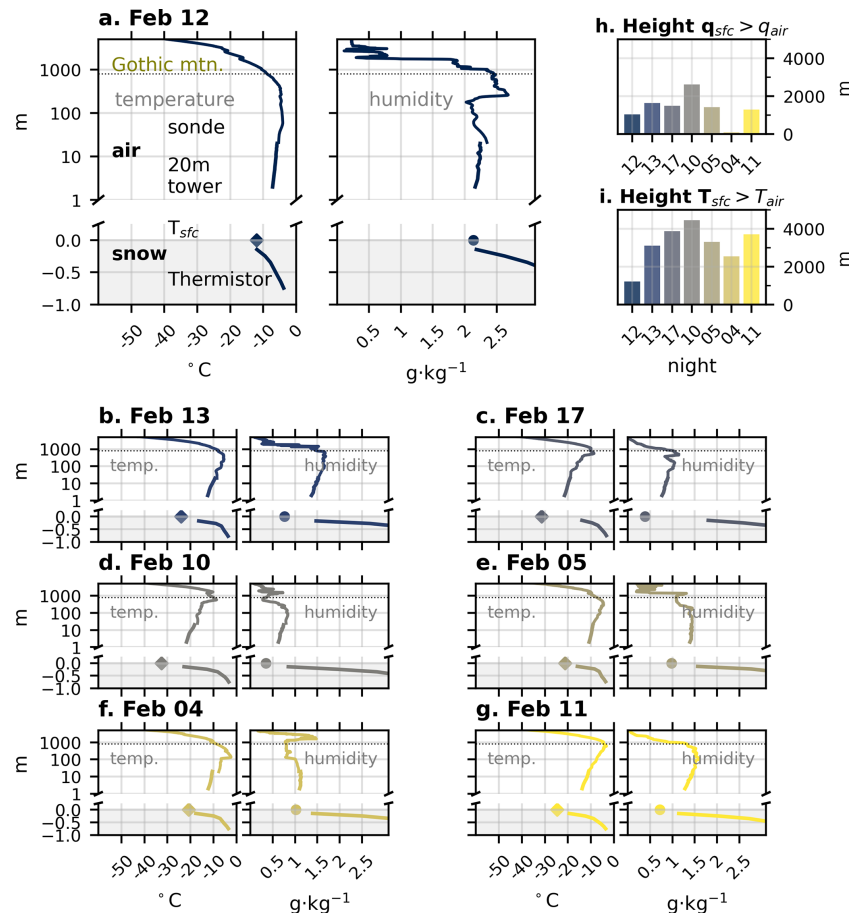
Figure 4. (a–g) 05:00 a.m. local time profiles of T_{\text{air}} and q_{\text{air}} throughout the snow–atmosphere continuum as measured by SOS towers, balloon sondes, down-looking radiometers ( T_{\text{sfc}} ), and buried snow thermistor arrays. Note the log scale y-axis. Units are heights in meters with respect to the snow surface height, defined as 0. (h, i) Barplots on the top-right depict the lowest atmospheric height level at which T_{\text{sfc}} and q_{\text{sfc}} exceeds the respective value in the atmosphere for each night. The panels are ordered by the size of the surface hoar event in the same order as (Fig. 8).
