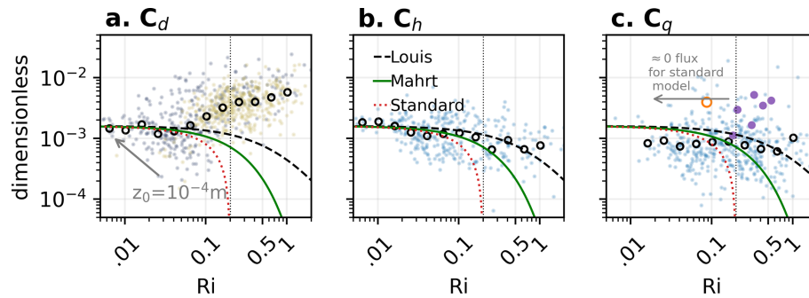
Figure 6. Relationship between Ri and the bulk transfer coefficients for (a) momentum (b) heat, and (c) moisture computed from EC fluxes and bulk gradients using Eqs. (2)–(4). Blue circles in (a)–(c) are 30 min values for all time periods considered and black open circles are bin-averages. Yellow circles in (a) denote clear-sky conditions. Purple and orange circles are estimated from Stössel box observations and digitized data from H97 respectively in (c). The solid, dashed, and dotted lines correspond to theoretical stability correction curves using the Mahrt, Louis, and standard parameterizations implemented in the SUMMA model and z_0 = 2 \times 10^{-4} .
