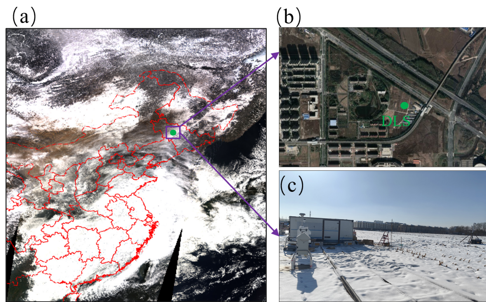
Figure 1. Sampling site (DLS) information: (a) Satellite-derived snow cover image (data source: National Snow and Ice Data Center, https://nsidc.org/data , last access: 17 September 2026). (b) Traffic conditions around the sampling site at the Northeast Institute of Geography and Agroecology, Chinese Academy of Sciences (NIGA), Jilin Province, China (Imagery © 2026 Airbus, Map data © 2026 Google, https://earth.google.com/ , last access: 17 September 2026). (c) The observation station surrounded by snow-covered farmland.
