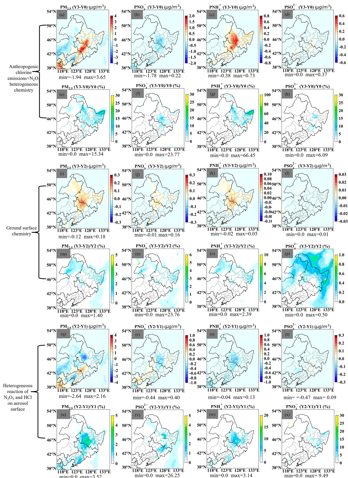
Figure 7. The quantitative contribution of different pathways of chlorine chemistry on \text{PM}_{2.5} , and its chemical components.
