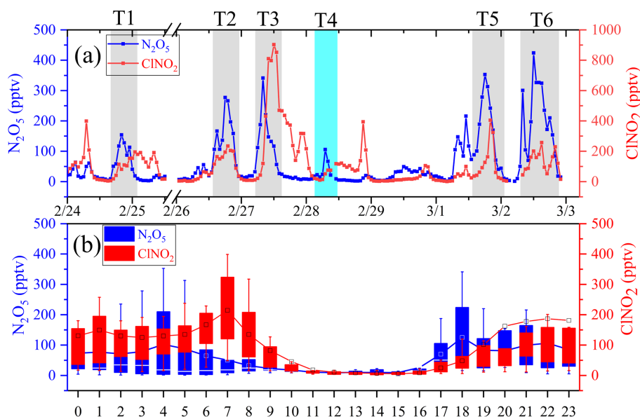
Figure 2. Field observations of \text{N}_2\text{O}_5 and \text{ClNO}_2 at the DLS station from 23 February to 3 March 2024. (a) Time series. The gray shaded periods (T1, T2, T3, T5, and T6) represent episodes with concurrent elevated \text{N}_2\text{O}_5 and \text{ClNO}_2 peaks, while the cyan shaded period (T4) indicates an episode where no such concurrent peak was observed. The data gap between 14:00 (UTC+8) on 25 February and 10:00 (UTC+8) on 26 February is due to instrument maintenance, during which no measurements were available. (b) Diurnal variation.
