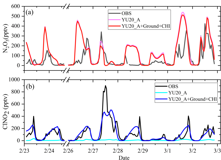
Figure 3. Comparison of simulated and observed values for YU20_A (Y0) and YU20_A_G_ChI (Y3) the DLS station in Northeast China: (a) \text{N}_2\text{O}_5 , (b) \text{ClNO}_2 .
