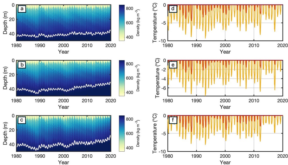
Figure 5. Modeled profiles of density (a–c) and modeled firn temperature (d–f) from 1980 to 2019 from the Kuipers Munneke et al. (2015) firn-densification model at the MLD site (a, d); MG3 site (b, e); and NWB1 site (c, f). Temperatures are shown at 3 m depth (light orange), 5 m depth (dark orange), and 8 m depth (red) in (d)–(f). The temperature at 8 m depth was always at 0 °C over this interval, see Fig. A5. Bubble close-off depth (approximately 830 kg m −3 ) is delineated by the white line on (a)–(c).
