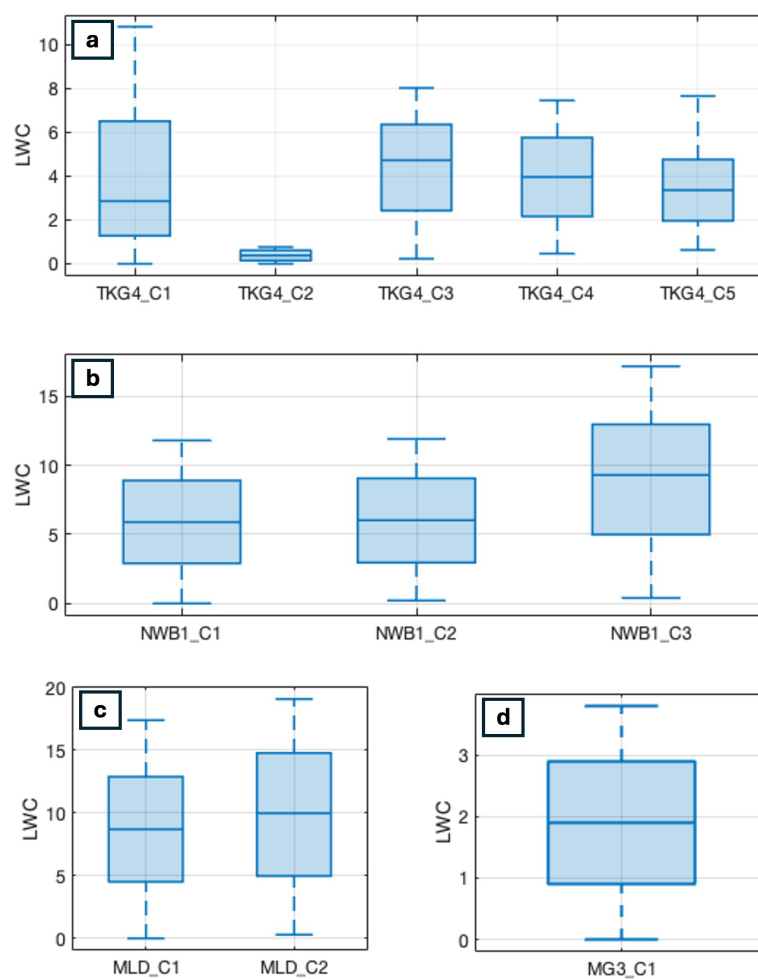
Figure A4. Box plots of repeated measurements of liquid water content (LWC) of the full cores at all the four sites: (a) TKG4, (b) NWB1, (c) MLD, and (d) MG3.
