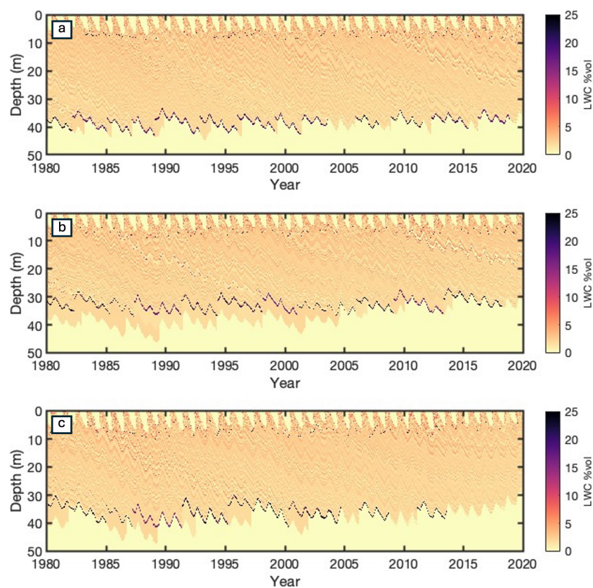
Figure A6. Modeled liquid-water content (LWC) profile evolution for the three sites: (a) MLD, (b) MG3, and (c) NWB1.
