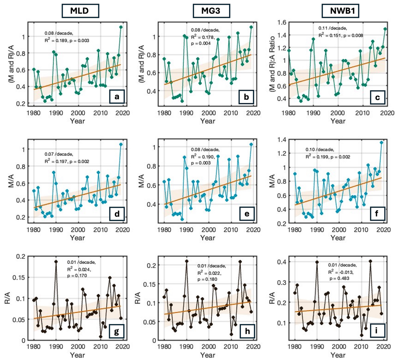
Figure A3. Comparison between climate variables from the Ing et al. (2025) product for the three accumulation-zone sites (MLD, MG3, NWB1). Ratio between the sum of cumulative annual melt and rain to the cumulative annual snow accumulation (a–c); ratio between melt and accumulation (d–f); and ratio between rain and accumulation (g–i).
