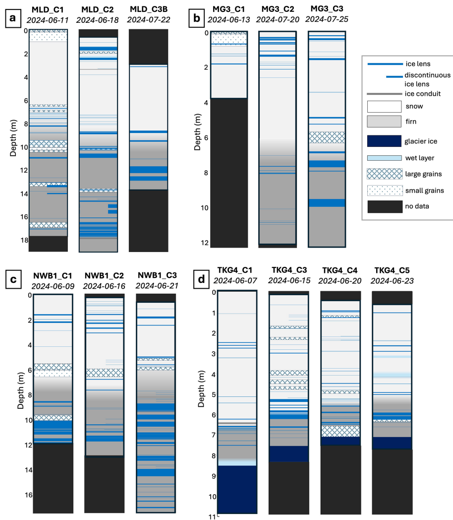
Figure 3. Stratigraphy of the repeat firn cores at sites (a) MLD, (b) MG3, (c) NWB1, and (d) TKG4. All surfaces are corrected for ablation, except MG3, where no ablation measurements exist. Repeat cores were taken within 1–3 m of each other. Stratigraphic differences suggest high local variability in the snow and firn structure even in high-melt environments like the Juneau Icefield. Large volumes of liquid water were found at the base of the TKG4_C1 core. Note that there is no TKG4_C2 core, due drill malfunction.
