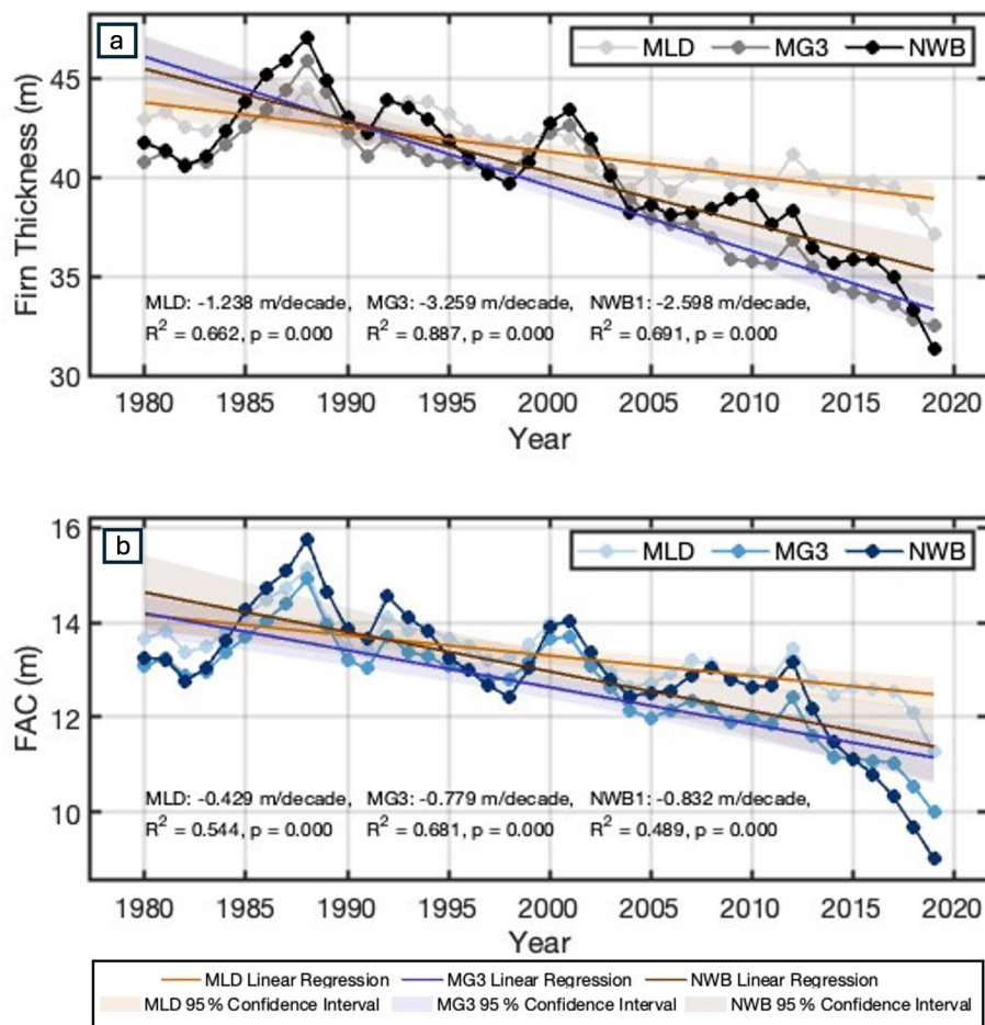
Figure 6. Modeled (a) mean annual firn thickness and (b) mean annual firn-air content (FAC) from the Kuipers Munneke et al. (2015) firn-densification model at accumulation-zone sites MLD, MG3, and NWB1 from 1980 to 2019.
