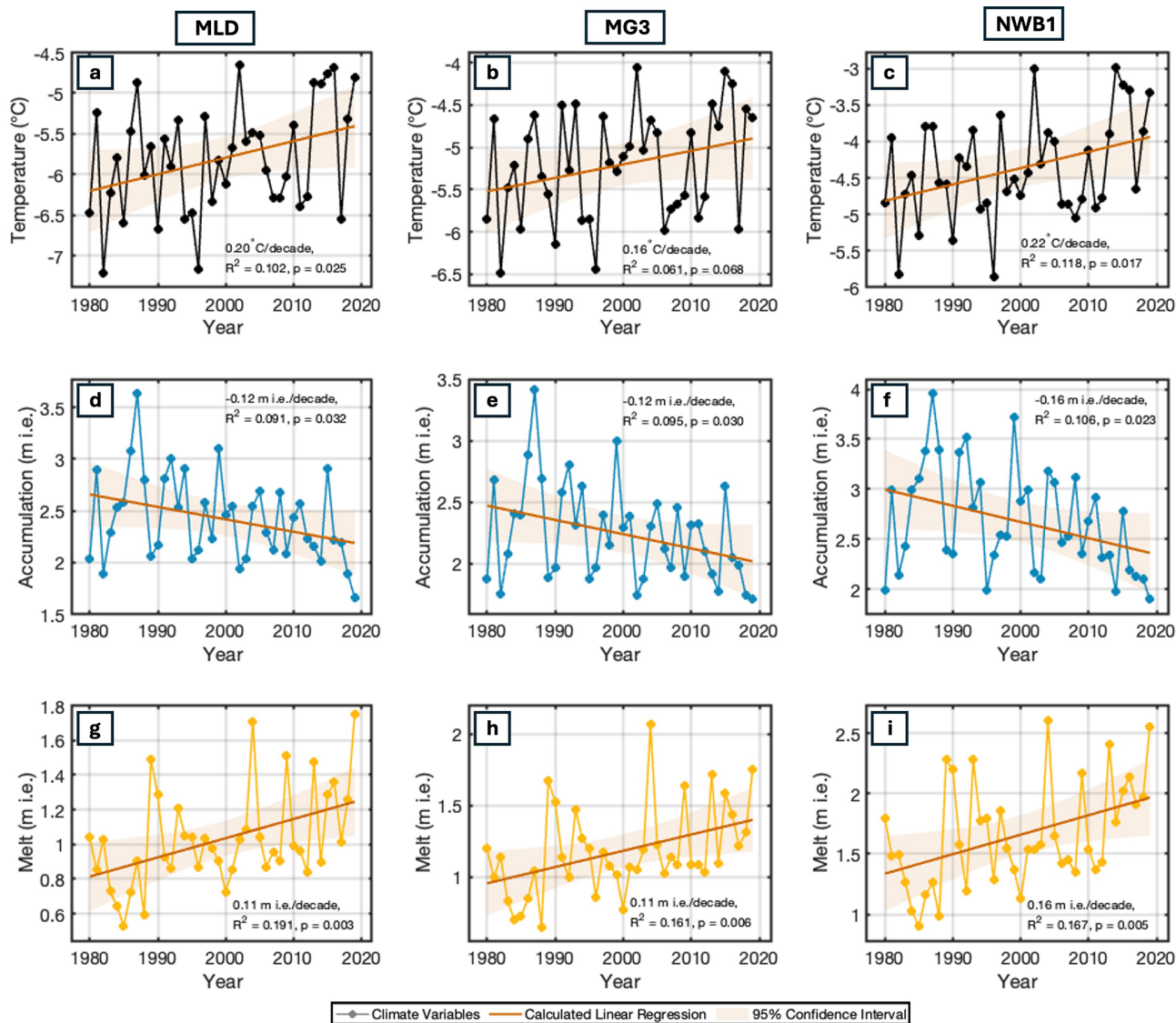
Figure 2. Mean annual climate at each site in the accumulation zone (MLD, MG3, NWB1) derived from the product by Ing et al. (2025): mean annual temperature (a–c), cumulative annual snow accumulation (d–f), and cumulative annual surface melt (g–i).
