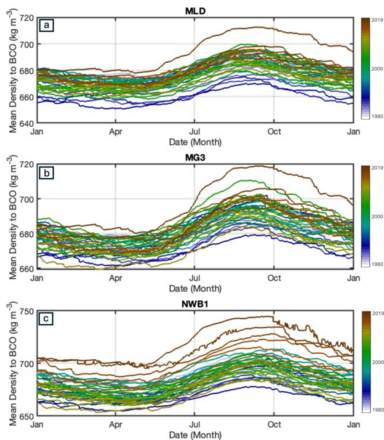
Figure A9. Modeled daily mean density (dry + liquid) from 1980–2019 for the three sites: (a) MLD, (b) MG3, and (c) NWB1.
