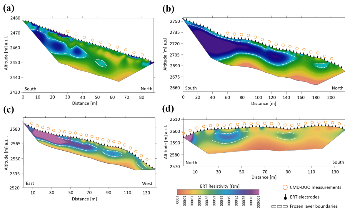
Figure 2. Inverted resistivity models obtained from ERT measurements at (a) the active rock glacier at Flüela Pass, (b) the active rock glacier at Stelvio Pass, (c) Le Rese di Scorluzzo inactive rock glacier, and (d) the Le Rese di Scorluzzo inactive protalus rampart at Stelvio Pass. The positions of the ERT electrodes (black point marker with stem) along the transects and the measurement points acquired with the CMD-DUO FDEM system (orange circle) are shown. The white dashed lines indicate the interpreted boundary of the inferred frozen layer.
