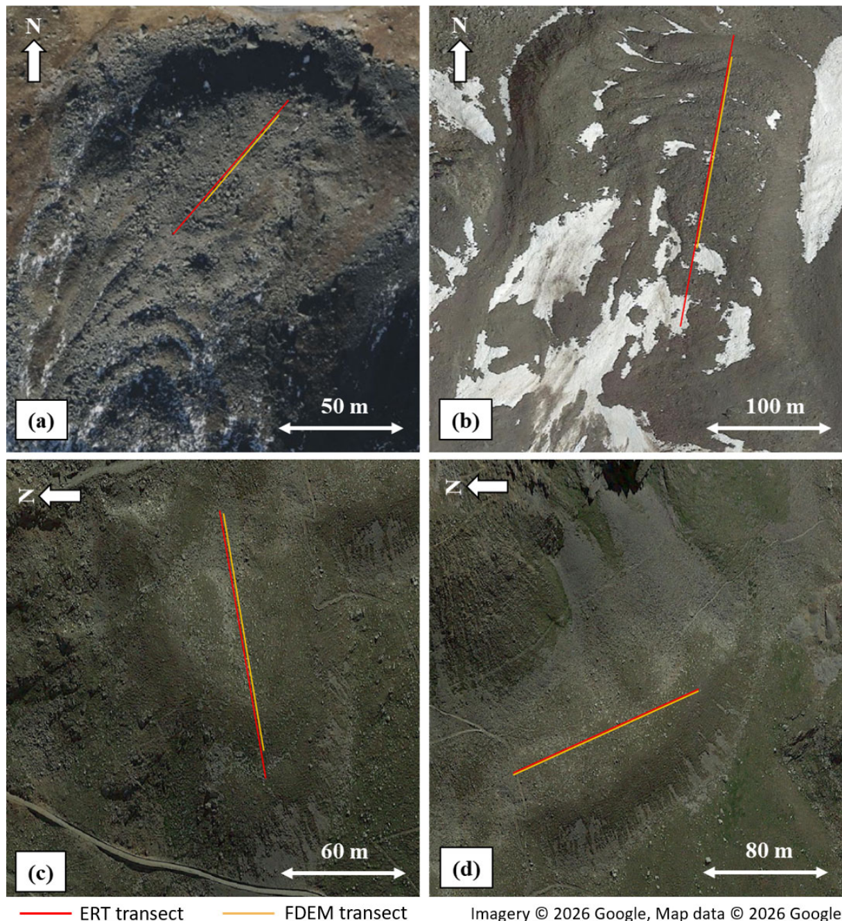
Figure 1. Satellite images of the study sites showing the ERT (red lines) and FDEM (orange lines) survey profiles. (a) Active rock glacier at Flüela Pass (Switzerland; 46.746° N, 9.951° E). (b) Active rock glacier at Stelvio Pass (Italy; 46.527° N, 10.441° E). (c) Le Rese di Scorluzzo inactive rock glacier at Stelvio Pass (Italy; 46.531° N, 10.420° E). (d) Le Rese di Scorluzzo inactive protalus rampart at Stelvio Pass (Italy; 46.530° N, 10.421° E). Background imagery: Imagery © 2026 Google, Map data © 2026 Google (accessed via QuickMapServices in QGIS).
