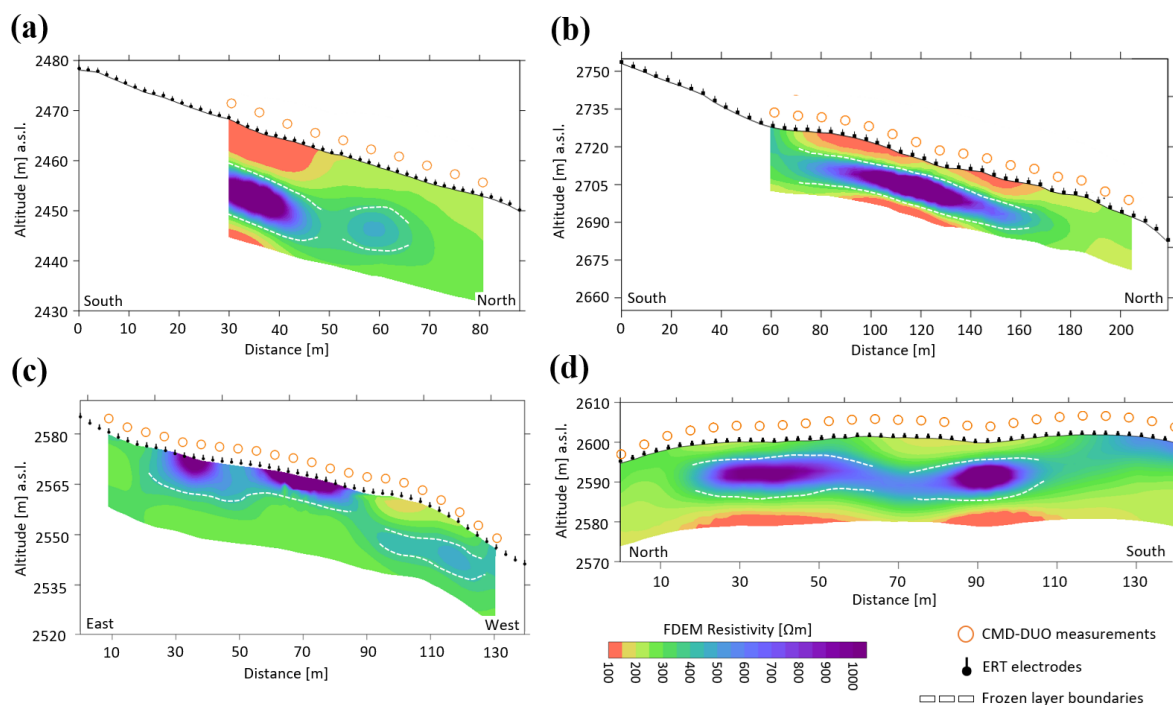
Figure 3. Pseudo-2D inverted resistivity models obtained from FDEM data acquired with the CMD-DUO in HCP configuration at the sites of (a) active rock glacier at Flüela Pass (RMSPE: 7.88 %), (b) active rock glacier at Stelvio Pass (RMSPE: 7.36 %), (c) Le Rese di Scorluzzo inactive rock glacier (RMSPE: 4.03 %), and (d) the Le Rese di Scorluzzo inactive protalus rampart at Stelvio Pass (RMSPE: 6.18 %). The positions of the FDEM measurement points are marked with orange circles, and the white dashed lines indicate the inferred boundary of the frozen layer.
