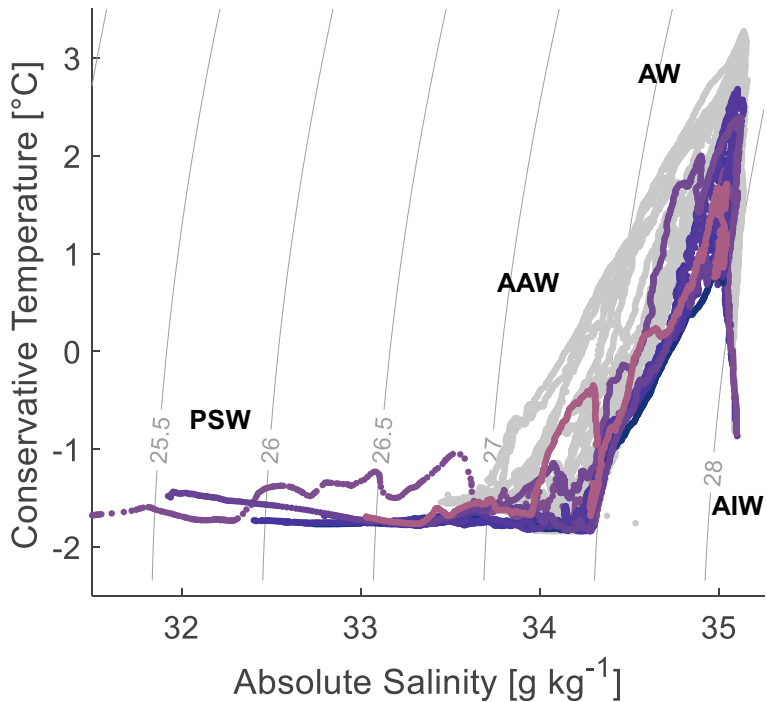
East Greenland Current
