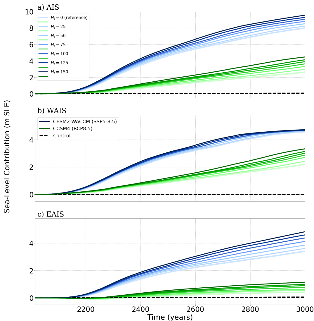
Figure 3. SLC relative to 2015 (m SLE) for the different values of H_t (in m) used. In (a) for the whole AIS, in (b) for the WAIS, and in (c) for the EAIS. Dashed lines represent the control simulations corresponding to the different values of H_t , overlapping as variations are very small during the simulation period.
