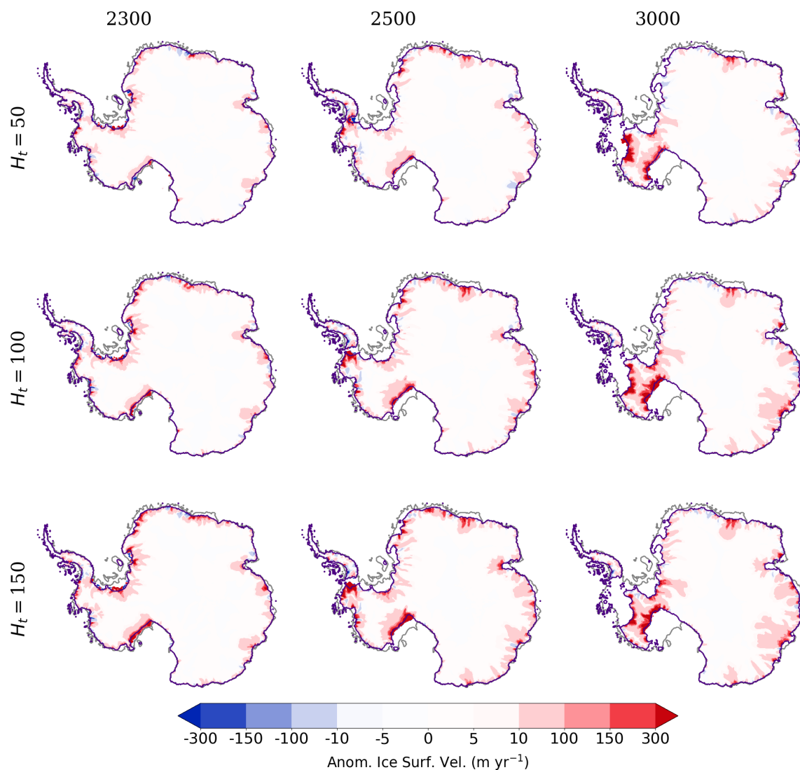
Figure 7. Same as Fig. 6 but for the experiments with CCSM4 (RCP8.5).
