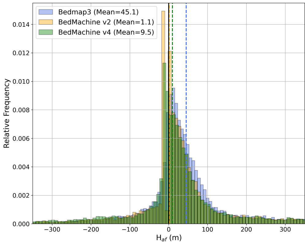
Figure 8. Histograms of H_{af} (m) for three different topography datasets (Bedmap3, BedMachine v2, and BedMachine v4), using all the GZs regions in Fig. 2. Dashed lines indicate the average value for each topography dataset.
