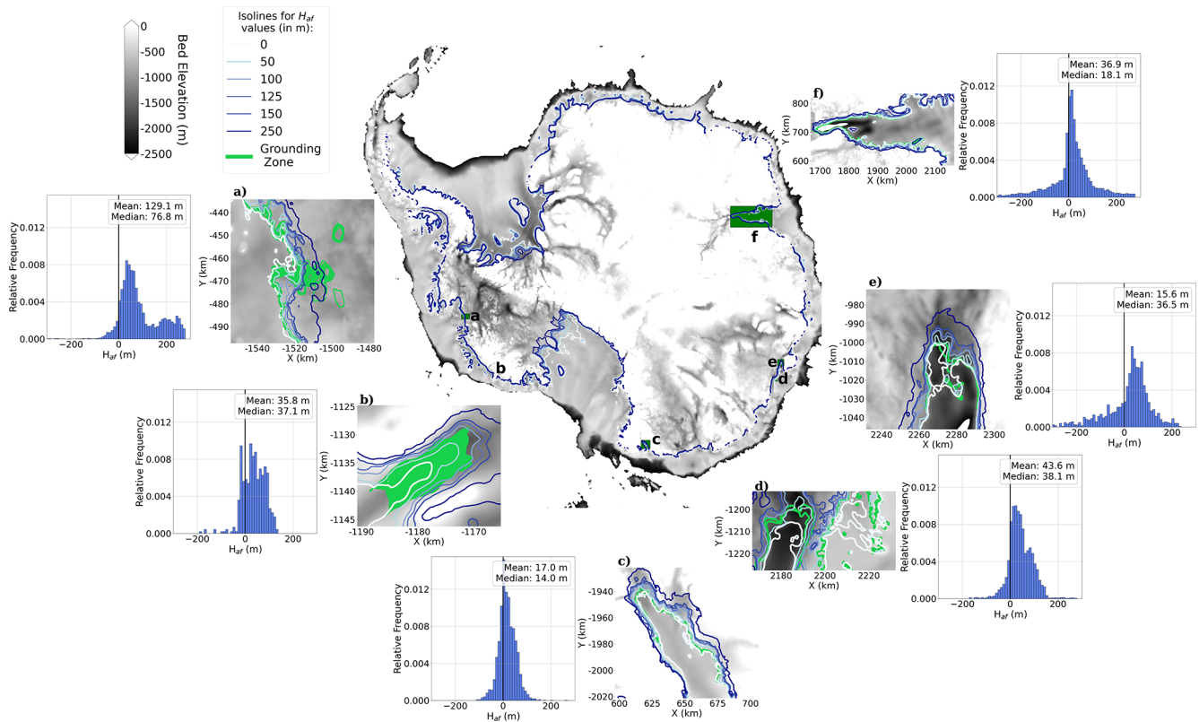
Figure 2. Observational estimates of the GZ for different regions compared with isolines of thickness above flotation. Rectangles with letters (a–f) delimit the extension of the different regions of the insets, for which the observational GZ obtained through DInSAR from different studies is shown in green: (a) Thwaites Glacier (Rignot et al., 2024), (b) Berry Glacier (Chen et al., 2025), (c) Rennick Glacier (Ross et al., 2025), (d) Moscow University Glacier (Ross et al., 2025), (e) Totten Glacier (Ross et al., 2025) and (f) Amery Ice Shelf (Zhu et al., 2025). The isolines of thickness above flotation, H_{af} , are calculated from the Bedmap3 dataset (Pritchard et al., 2025) with a resolution of 500 m. Grayscale shading shows the bedrock topography. Next to each panel, histograms of the H_{af} (m) values are shown corresponding to the data points contained within the GZ. Mean and median values are indicated in each panel.
