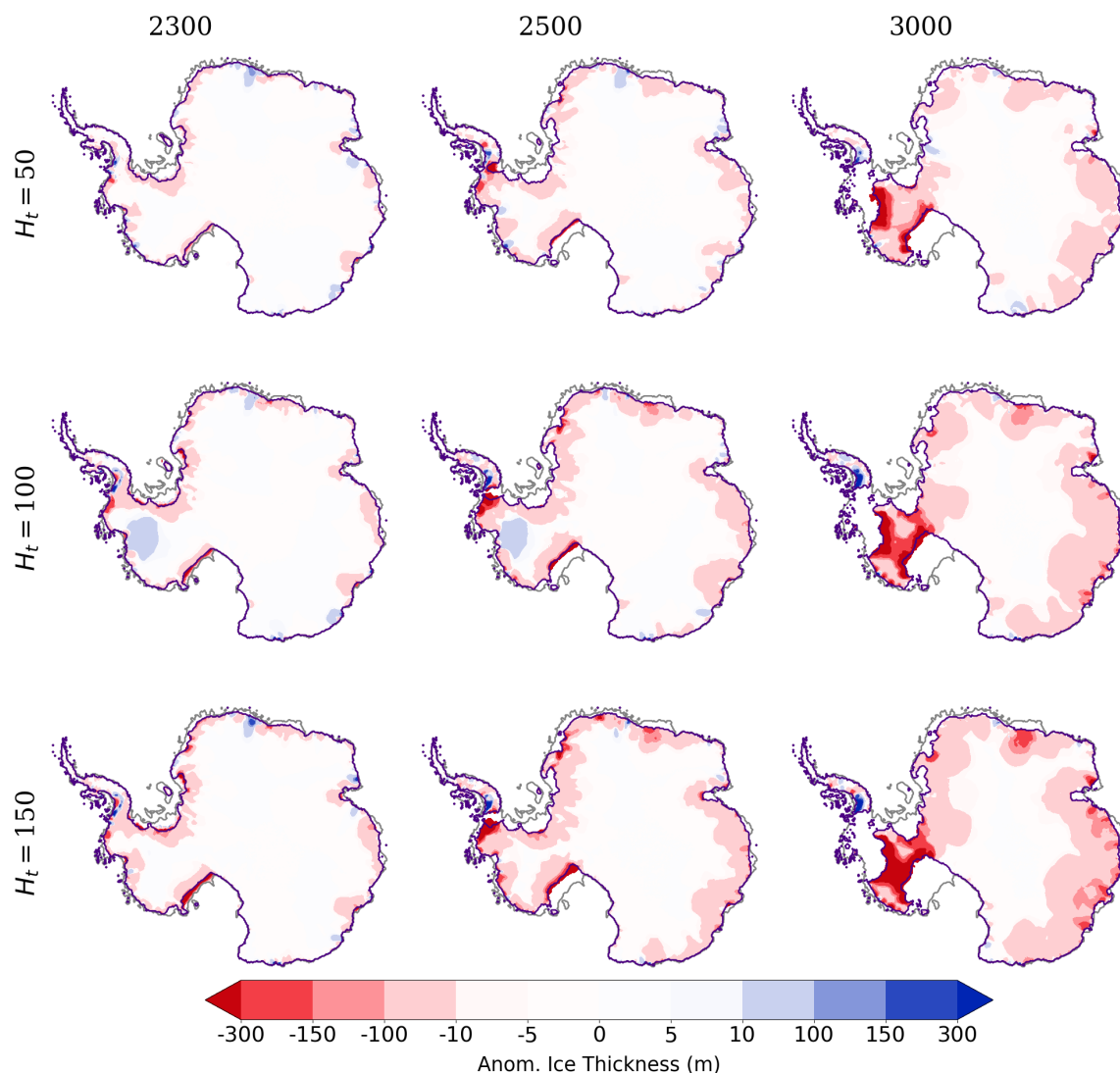
Figure 5. Same as Fig. 4 but for the experiments with CCSM4 (RCP8.5).
