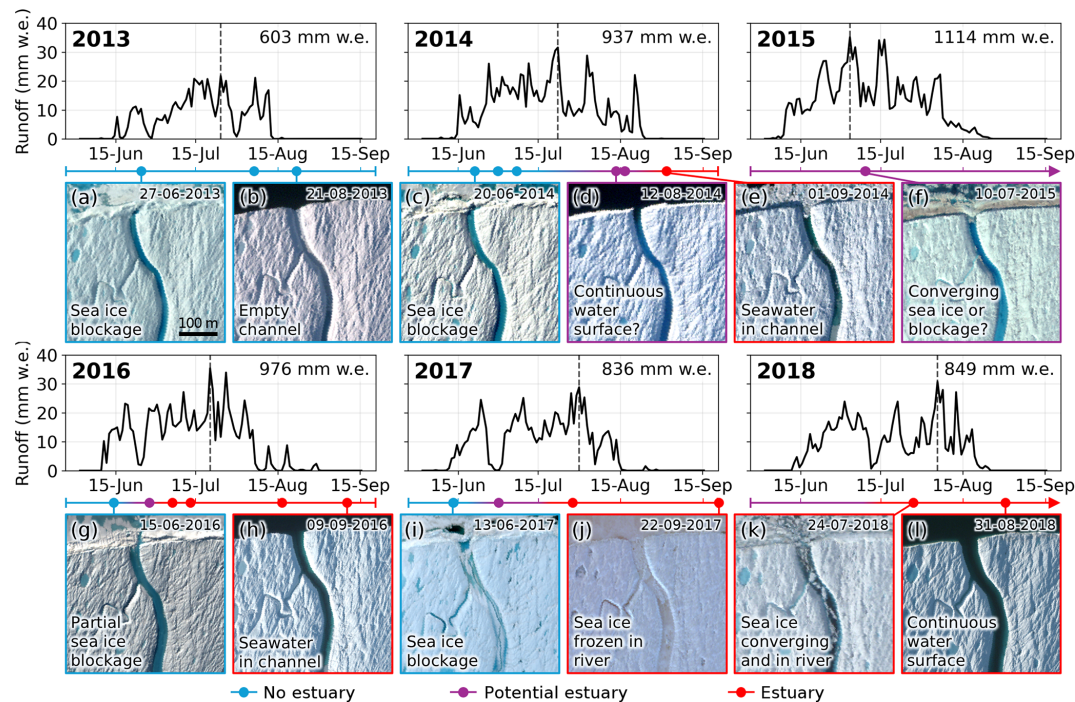
Figure 8. Timeline of Petermann Ice Shelf estuary formation showing surface runoff and WorldView imagery from 2013 to 2018 (© Vantor 2025). Summer (1 June to 15 September) runoff over Petermann Ice Shelf from MAR is shown in black with a dashed line indicating peak runoff. A corresponding timeline coloured by likelihood of estuary presence (blue for no estuary, purple for ambiguous, and red for estuary) is shown below each of the runoff plots with coloured circles on the timeline representing availability of cloud-free WorldView-2/3 images; 12 example images (a–l; all at the same spatial scale) are shown below their respective coloured circles on the timeline and are labelled with relevant estuary formation criteria information. Gradients between two solid colours on the timeline indicate that a change in estuary likelihood occurred between two dates, but that the exact timing cannot be determined. At the end of each melt season, it is assumed that the conditions from the last cloud free image persist until refreezing. Additional images used to develop the timeline but not shown here can be found in Fig. S9.
