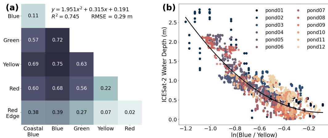
Figure 4. Dual channel depth equation calibration using OBRA: (a) heatmap showing R^2 for all 15 WorldView-2/3 band combinations with best fit equation and (b) scatterplot of ICESat-2 derived depths plotted against reflectance in the optimal band combination, blue and yellow, with the best fit line.
