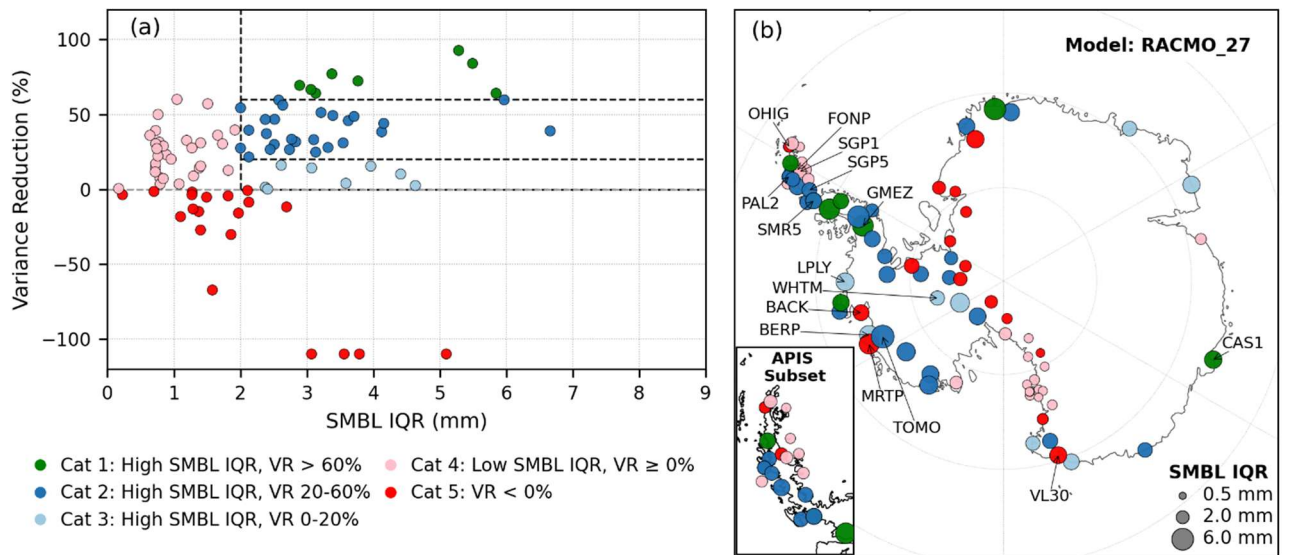
Figure S4: (a) Variance reduction at GPS stations as a function of SMBL IQR, for RACMO_27 model. Colours reflect categorisation into five categories based on SMBL IQR and variance reduction of the model. (b) GPS sites with colours reflecting the same categories as in a) and symbol sizes reflecting SMBL IQR. GPS site names discussed in the text are annotated.
