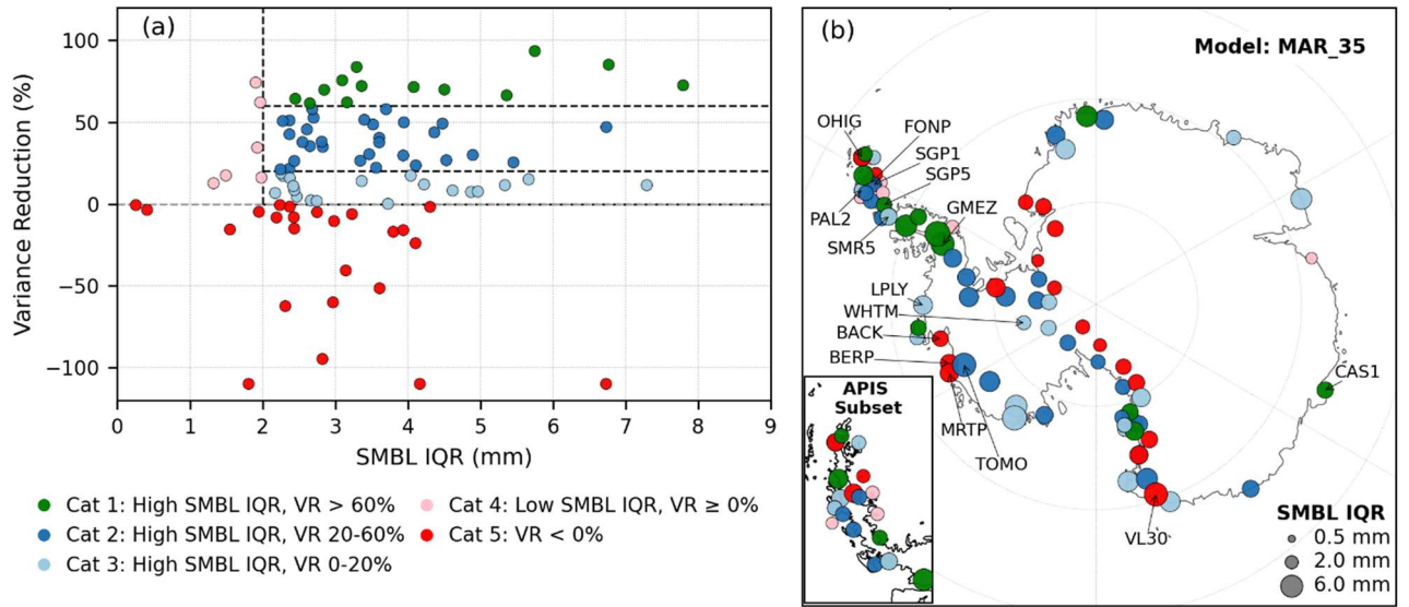
Figure S5: (a) Variance reduction at GPS stations as a function of SMBL IQR, for MAR_35 model. Colours reflect categorisation into five categories based on SMBL IQR and variance reduction of the model. (b) GPS sites with colours reflecting the same categories as in a) and symbol sizes reflecting SMBL IQR. GPS site names discussed in the text are annotated.
