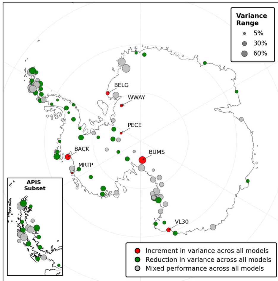
Figure S13: Range of variance change at GPS stations across the seven SMB models. Circle colour indicates the consistency of each station's response across the SMB models: red denotes stations where application of SMB loading increases variance across all the models, green denotes stations where application of SMB loading reduces variance across all the models, and gray denotes stations where the response varies across models. Circle size indicates the range of variance change across models.
