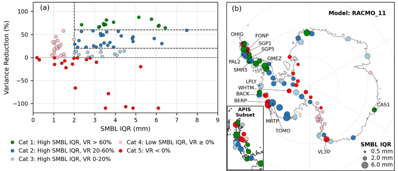
Figure S3: (a) Variance reduction at GPS stations as a function of SMBL IQR, for RACMO_11 model. Colours reflect categorisation into five categories based on SMBL IQR and variance reduction of the model. (b) GPS sites with colours reflecting the same categories as in a) and symbol sizes reflecting SMBL IQR. GPS site names discussed in the text are annotated.
