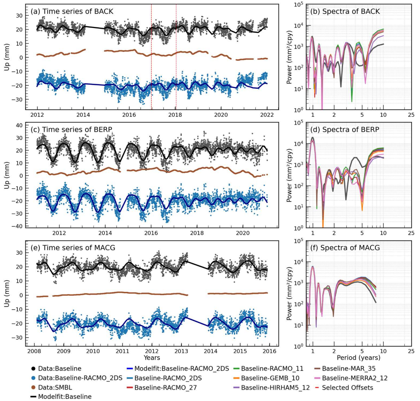
Figure S2: (Left Panels) Detrended vertical GPS time series for the stations BACK (a), BERP (c) and MACG (e). Gray dots correspond to detrended REGAIN vertical time series corrected for NTOL (REGAIN-NTOL; baseline) and vertically offset by +20 mm for visual clarity. Brown dots represent detrended SMBL time series from RACMO_2DS model and the blue dots correspond to the resulting time series after applying the SMBL correction (REGAIN-NTOL-SMBL), vertically offset by -20 mm. Solid blue and black lines show the linear models estimated before (offset by +20 mm) and after (offset by -20 mm) SMBL correction, respectively. Red dashed lines mark the dates of identified offsets. The time series in panels (a), (c) and (e) span different observation periods. (Right Panels) Lomb-Scargle spectra for stations BACK (b) and BERP (d) and MACG (f).
