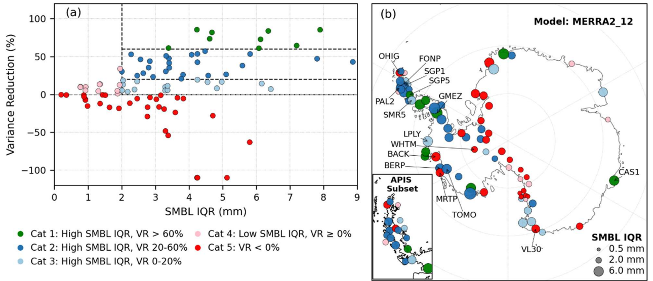
Figure S7: (a) Variance reduction at GPS stations as a function of SMBL IQR, for MERRA2_12 model. Colours reflect categorisation into five categories based on SMBL IQR and variance reduction of the model. (b) GPS sites with colours reflecting the same categories as in a) and symbol sizes reflecting SMBL IQR. GPS site names discussed in the text are annotated.
