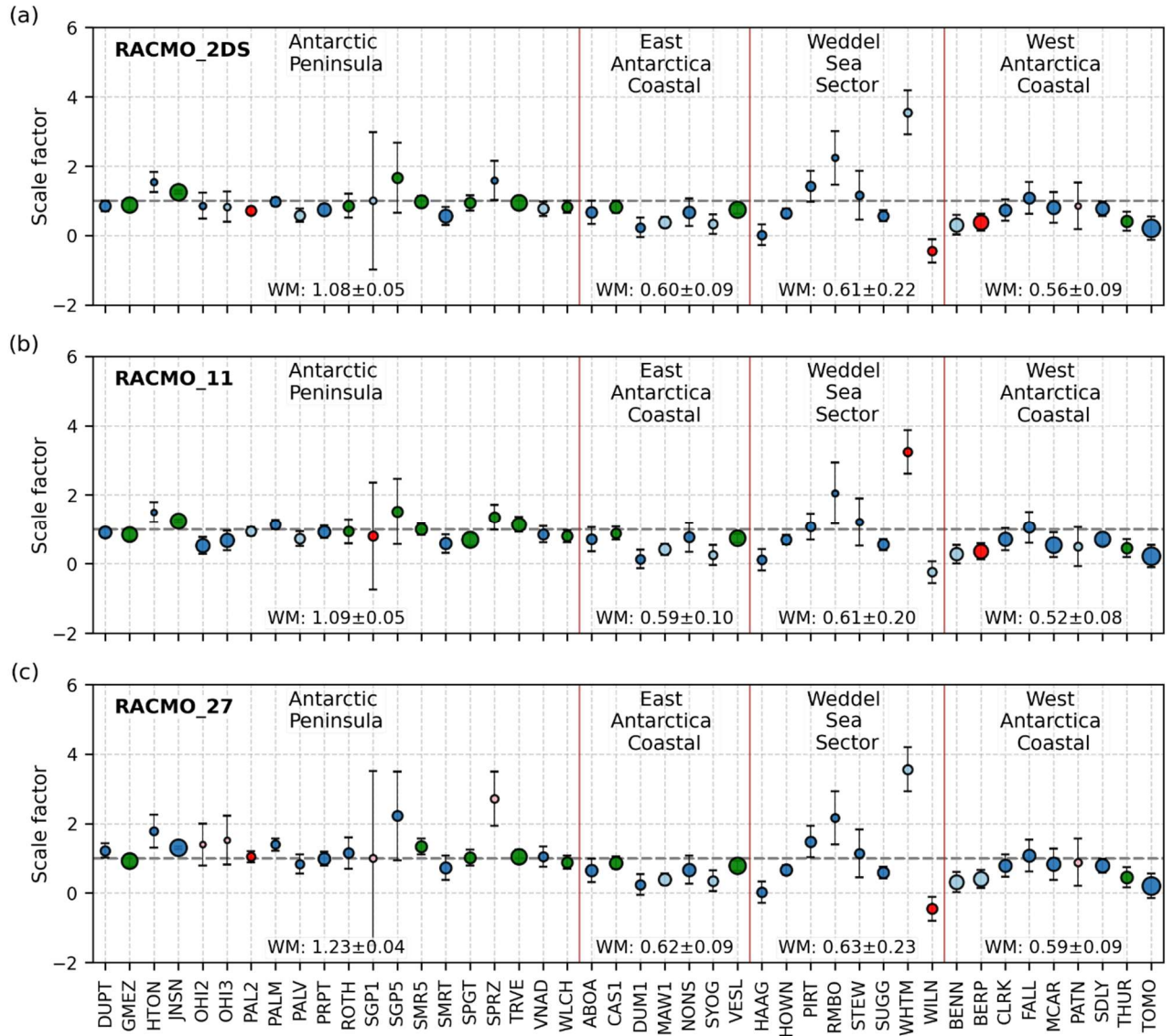
Figure S9: Scale factors and associated uncertainty for (a) RACMO_2DS (b) RACMO_11 and (c) RACMO_27 models grouped by geographical region. The size of the markers indicates the respective SMBL IQR and the colours indicates the categories of the sites as in Figure 5. Error bars indicate a 1-sigma uncertainty. The horizontal dashed line marks a scale of 1.
