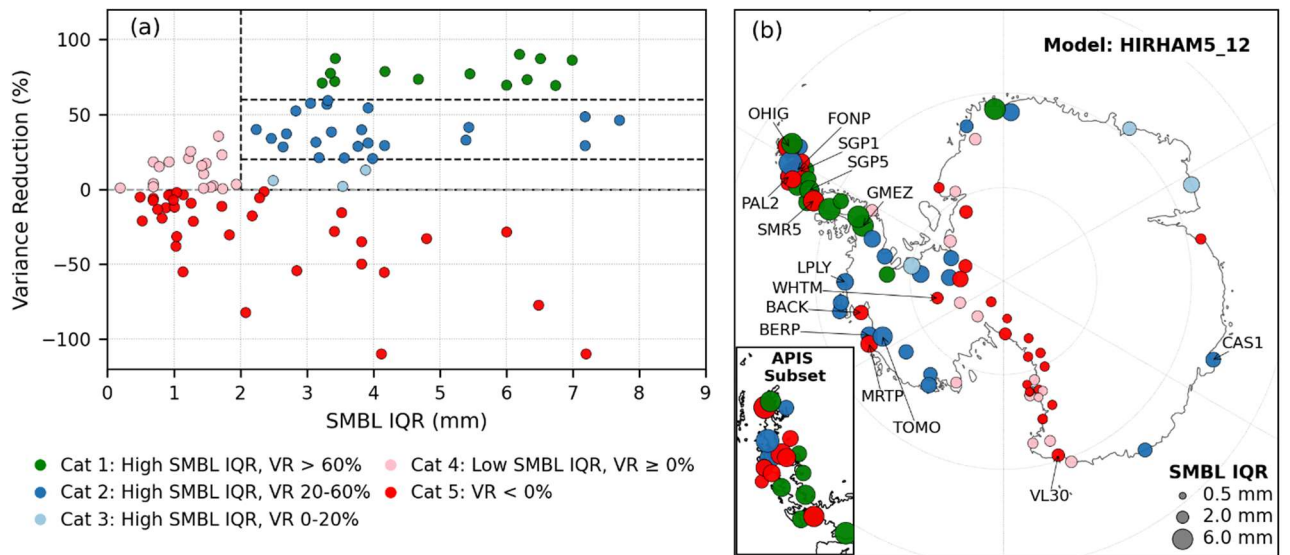
Figure S8: (a) Variance reduction at GPS stations as a function of SMBL IQR, for HIRHAM5_12 model. Colours reflect categorisation into five categories based on SMBL IQR and variance reduction of the model. (b) GPS sites with colours reflecting the same categories as in a) and symbol sizes reflecting SMBL IQR. GPS site names discussed in the text are annotated.
