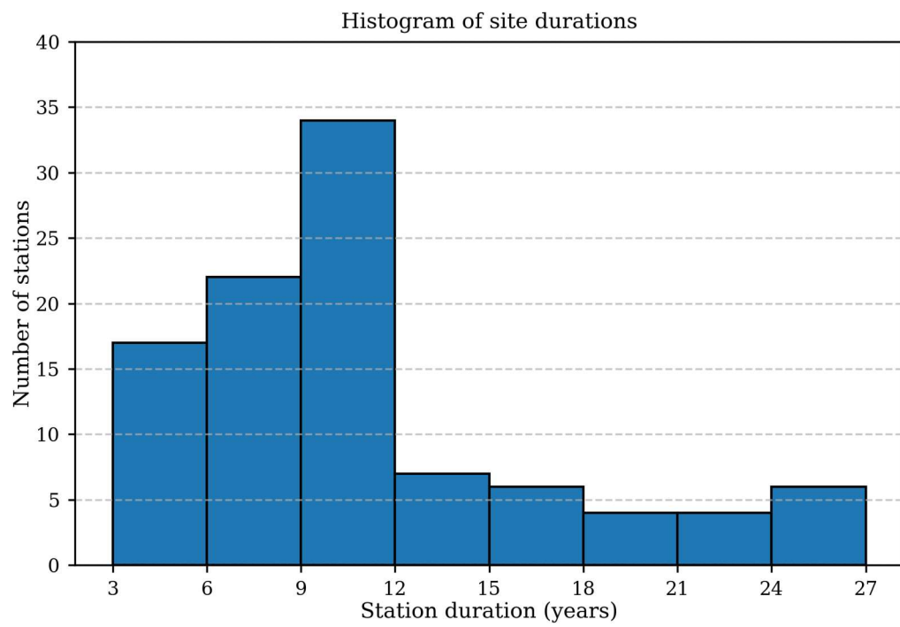
Figure S1: Histogram of site duration, considered for this study as shown with brown circles in Figure 2.
