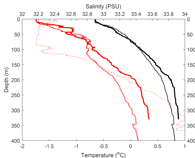
Figure 11. Vertical profiles down to 400 m depth of temperature (red) and salinity (black) in front of Tracy glacier in March 2022 (thick lines) and March 2023 (thin lines). Also shown is a March 2022 temperature profile at the mouth of the fjord at the edge of the landfast sea-ice (dotted).
