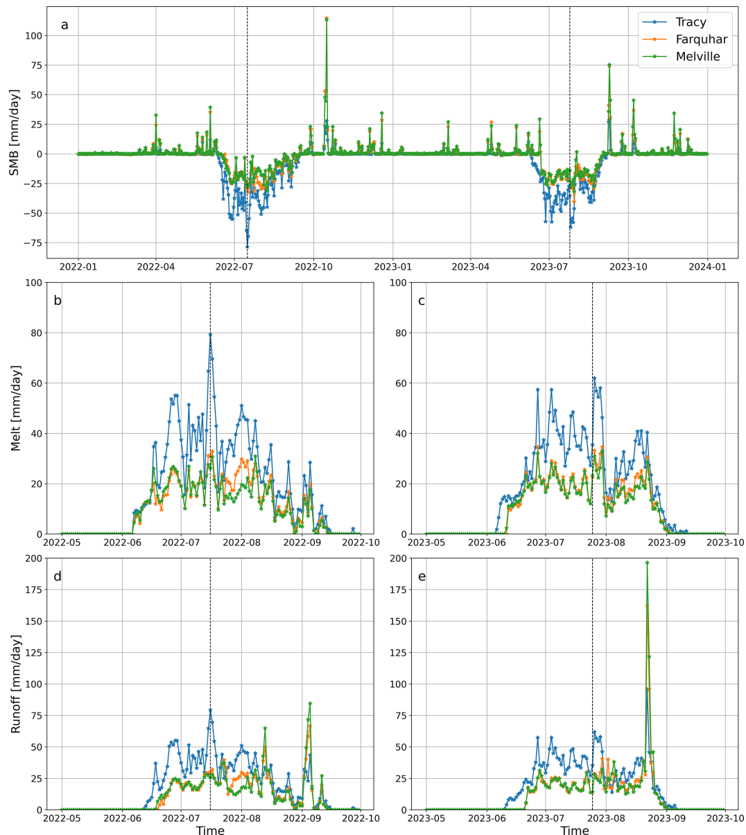
Figure 15. Daily SMB (a), surface melt 2022 (b) and 2023 (c), and surface runoff 2022 (d) and 2023 (e) for the three glaciers. All values are given in mm per day, from the model grid cell nearest the glaciers. The vertical black dashed lines show the date of the sea ice break-up in 2022 and 2023.
