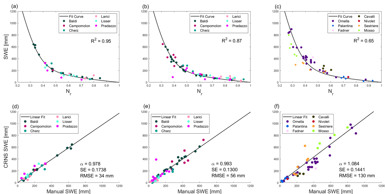
Figure 2. Normalised daily neutron count rate ( x -axis) against SWE direct measurements ( y -axis) for each site (coloured dots), and regression curve (black line) for the calibration dataset (a) and validation dataset divided between the six sites chosen for calibration (b) and the remaining seven sites (c). Manual SWE measurements plotted against SWE_{CRNS} ; coloured dots represent the calibration (d), validation in the same sites as calibration (e), and validation at different sites (f) dataset respectively; the black lines illustrate the linear regression fit performed for each dataset.
