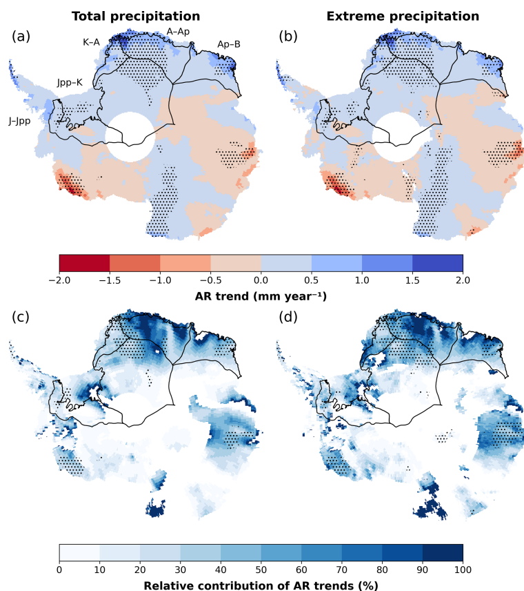
Figure 7. Annual trends in AR-associated (a) total and (b) extreme precipitation over Antarctica from 1980 to 2023 ( \text{mm yr}^{-1} ) from the AR detection dataset. Also shown are the relative contribution of the (c) AR-associated total precipitation trend to the ERA5-based total precipitation trend (%), and the (d) AR-associated extreme precipitation trend to the ERA5-based extreme precipitation trend (%). Stippling indicates regions where trends are statistically significant at the 90 % confidence level. Also shown in panel (a) are the locations of the A-Ap and K-A (Dronning Maud Land), Ap-B (Enderby Land), and J-Jpp (Filchner-Ronne) basins in East Antarctica, and the Jpp-K (Filchner-Ronne) basin in West Antarctica.
