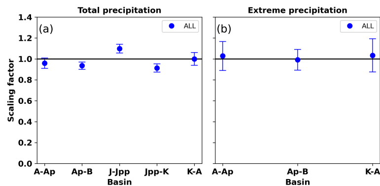
Figure 5. (a) One-signal estimates of basin-averaged scaling factors (solid blue circles) for annual total precipitation for drainage basins A-Ap, Ap-B, J-Jpp, Jpp-K and K-A from 1979 to 2023 based on regressing the CESM1 ALL ensemble against ERA5. (b) as (a) but for annual extreme precipitation for basins A-Ap, Ap-B and K-A. The error bars denote the 90 % confidence intervals and the horizontal line indicates a scaling factor of one. The A-Ap and K-A (Dronning Maud Land), Ap-B (Enderby Land), and J-Jpp (Filchner-Ronne) basins are in East Antarctica, and the Jpp-K (Filchner-Ronne) basin in West Antarctica.
