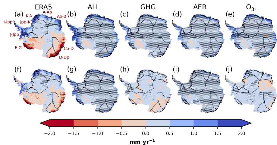
Figure 2. Annual linear trends in (a–e) total and (f–j) extreme precipitation over Antarctica from 1979 to 2023 ( \text{mm yr}^{-1} ) for (a, f) ERA5 and the CESM1 ensemble mean for (b, g) ALL, (c, h) GHG, (d, i) AER and (e, j) O 3 . Stippling indicates regions where trends are statistically significant at the 90 % confidence level. Also shown in panel (a) are the locations of the A-Ap and K-A (Dronning Maud Land), Ap-B (Enderby Land), Cp-D (Wilkes Land), D-Dp (Victoria Land), and Jpp-K (Filchner-Ronne) basins in East Antarctica, the F-G (Marie Byrd Land) and J-Jpp (Filchner-Ronne) basins in West Antarctica, and the I-Ipp basin in the Antarctic Peninsula.
