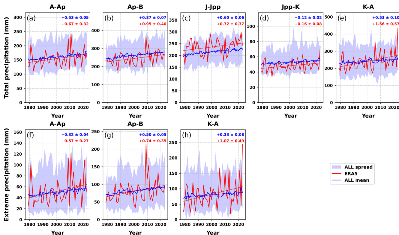
Figure 4. Times series of basin-averaged annual total precipitation (mm) for (a) A-Ap, (b) Ap-B, (c) J-Ipp, (d) Jpp-K, and (e) K-A, and annual extreme precipitation (mm) for (f) A-Ap, (g) Ap-B, and (h) K-A, from 1979 to 2023 from ERA5 (red) and the CESM1 ensemble mean for ALL (blue). Linear trends (statistically significant at 90 % confidence level) for ERA5 and ALL are represented by the red and blue lines, respectively. Blue shading represents the maximum and minimum ensemble spread of ALL. Each panel also shows the linear trend and the standard error ( \text{mm yr}^{-1} ). The A-Ap and K-A (Dronning Maud Land), Ap-B (Enderby Land), and J-Ipp (Filchner-Ronne) basins are in East Antarctica, and the Jpp-K (Filchner-Ronne) basin in West Antarctica.
