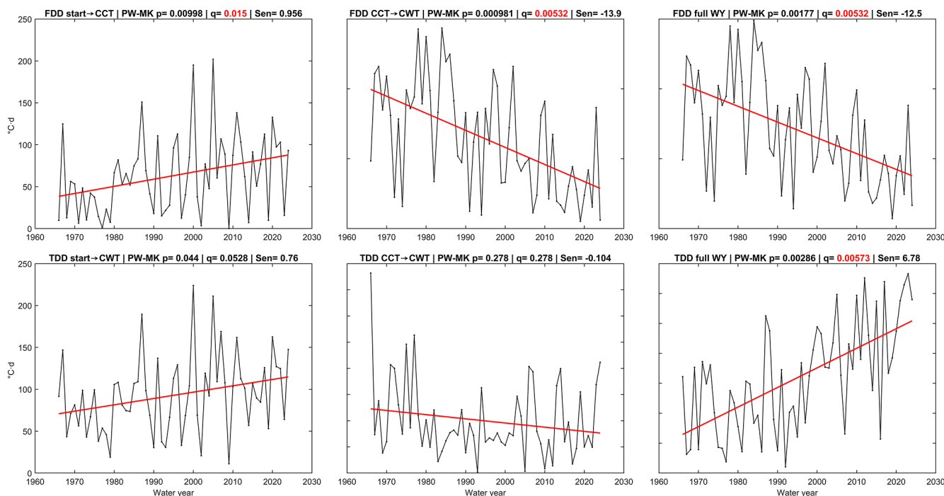
Figure 13. Long-term trends in freezing and thawing degree-day (FDD/TDD) linked to the ZCAT transition timings (WY1966–WY2024; n = 59 ). Panel titles report the PW-MK p -value, the Benjamini–Hochberg q -value (corrected within family), and Sen’s slope; the q -value is shown in red where the trend remains significant after correction ( q < 0.05 ).
