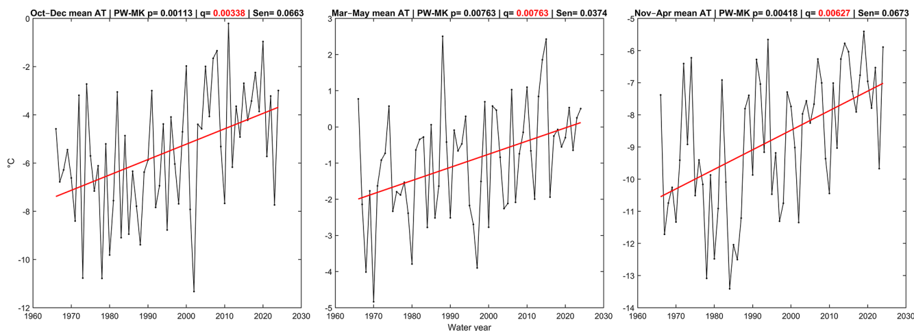
Figure 12. Long-term trends in seasonal air temperature (AT) (WY1966–WY2024; n = 59 ). Panel titles report the PW-MK p -value, the Benjamini–Hochberg q -value (corrected within family), and Sen’s slope; the q -value is shown in red where the trend remains significant after correction ( q < 0.05 ).
