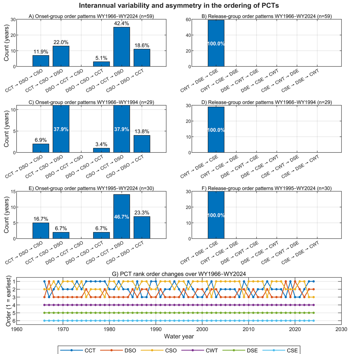
Figure 8. Interannual variability and asymmetry in the ordering of PCTs (WY1966–WY2024, n = 59 ). (A) Onset-group ordering frequencies, full record. (B) Release-group order-pattern frequencies, full record. (C) Onset-group order-pattern frequencies, early period (WY1966–WY1994, n = 29 ). (D) Release-group ordering frequencies, early period. (E) Onset-group ordering frequencies, late period (WY1995–WY2024, n = 30 ). (F) Release-group ordering frequencies, late period. (G) Year-to-year PCT rank order changes across the full record (rank 1 = earliest in that water year).
