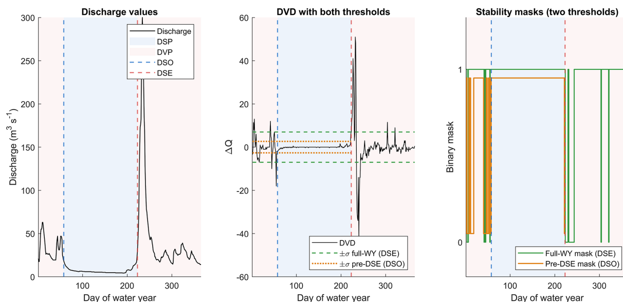
Figure 2. Detection of Discharge Stabilization Onset (DSO) and Discharge Stabilization End (DSE) by the Daily Value Difference (DVD) method, illustrated for WY1966. (Left) Daily discharge with DSO (blue dashed line) and DSE (red dashed line); the Discharge Stability Period (DSP) is shaded blue and the complementary Discharge Variability Period (DVP) pink. (Centre) Day-to-day discharge changes (DVD) with both variability thresholds: the full-water-year \pm\sigma band (green dashed), used to locate DSE as the end of the longest full-water-year stable run, and the stricter pre-DSE \pm\sigma band (orange dotted), used to locate DSO as the start of the longest stable run before DSE. (Right) The two corresponding binary stability masks: the full-water-year mask (green, for DSE) and the pre-DSE mask (orange, for DSO); a day is stable (mask = 1) when its DVD value lies within the relevant band, otherwise unstable (mask = 0). The pre-DSE mask in the third panel follows the same binary logic of Full-WY mask (0 and 1) but for better readability its height is manually reduced in this figure.
