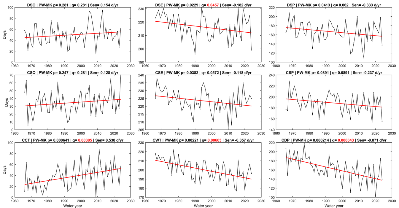
Figure 10. Long-term trends in Phase Change Timings (PCTs) and Intra-Variable Intervals (IVIs) (WY1966–WY2024; n = 59 ). Panel titles report the PW-MK p -value, the Benjamini–Hochberg q -value (corrected within family), and Sen’s slope; the q -value is shown in red where the trend remains significant after correction ( q < 0.05 ).
