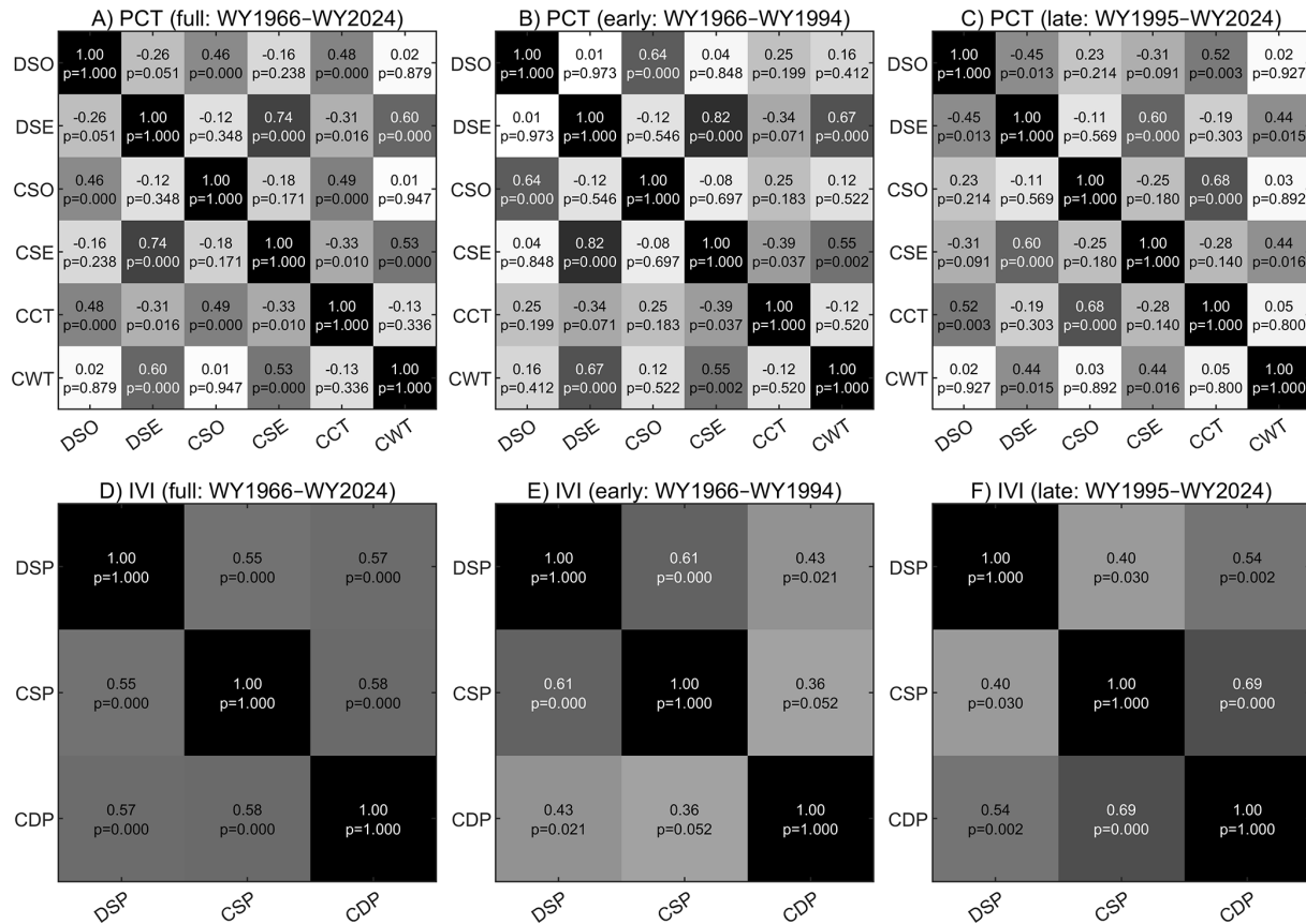
Figure 9. Spearman correlation matrices for PCTs (top row, panels A–C) and IVIs (bottom row, panels D–F) for the full record (WY1966–WY2024, n = 59 ), early period (WY1966–WY1994, n = 29 ), and late period (WY1995–WY2024, n = 30 ).
