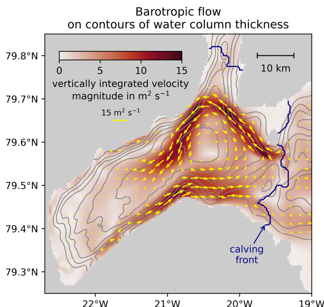
Figure 2. Intensity of the barotropic (i.e., vertically integrated) flow in the 79NG fjord shown in shades of red and the transport direction indicated by yellow arrows. Gray lines are the 100, 200, ..., 700 m isolines of the water column thickness, i.e., the depth of the seafloor minus the ice draft; the outermost contour corresponds to 100 m, the closed contour near the center to 700 m.
