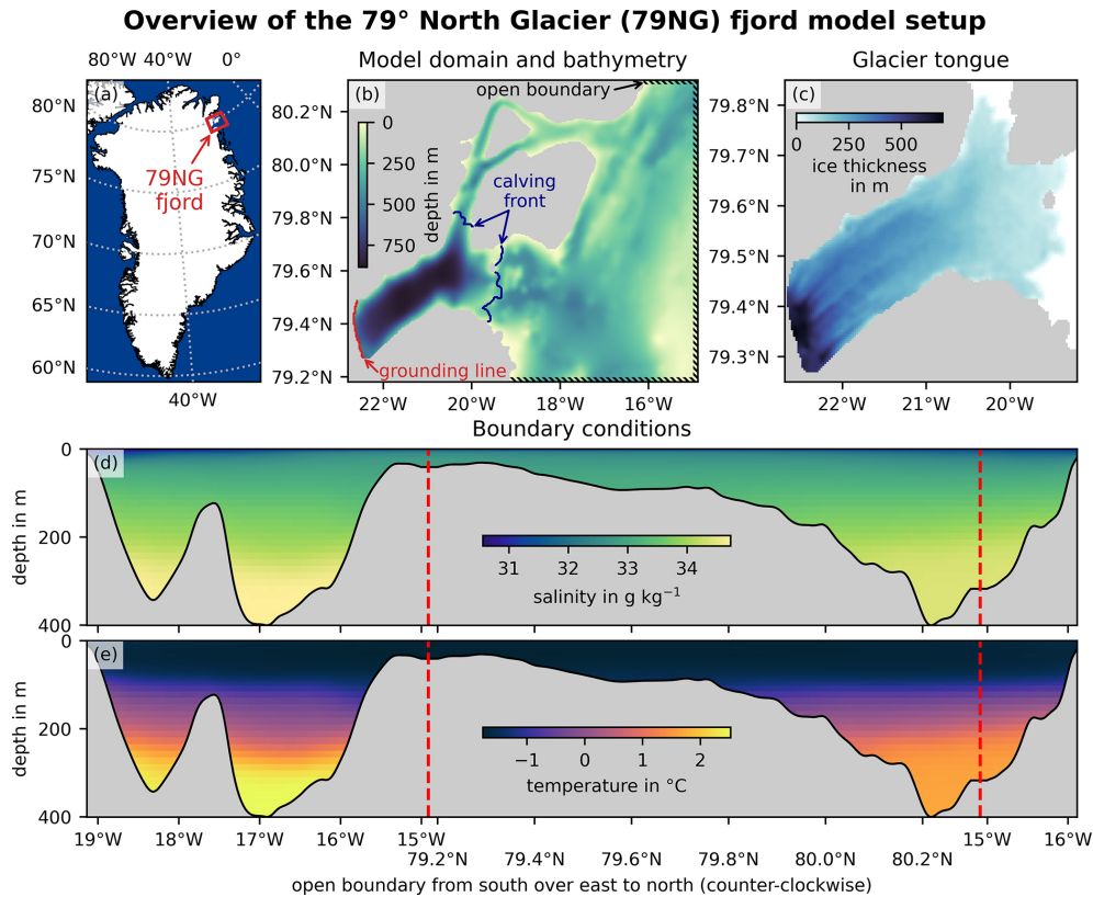
Figure 1. (a) Location of the 79NG fjord in Greenland. (b) Model domain and bathymetry; the northern branch of the fjord is Dijnphna Sound; subglacial discharge enters through the grounding line, which is the landward end of the floating glacier tongue; the calving front is its seaward end. (c) Thickness of the floating 79NG tongue. (d) Salinity and (e) temperature boundary conditions of the model; the open boundary (hatched area in panel b) is shown “unwinded” in counter-clockwise direction with the red dashed vertical lines marking the transitions between the southern, eastern and northern boundaries.
