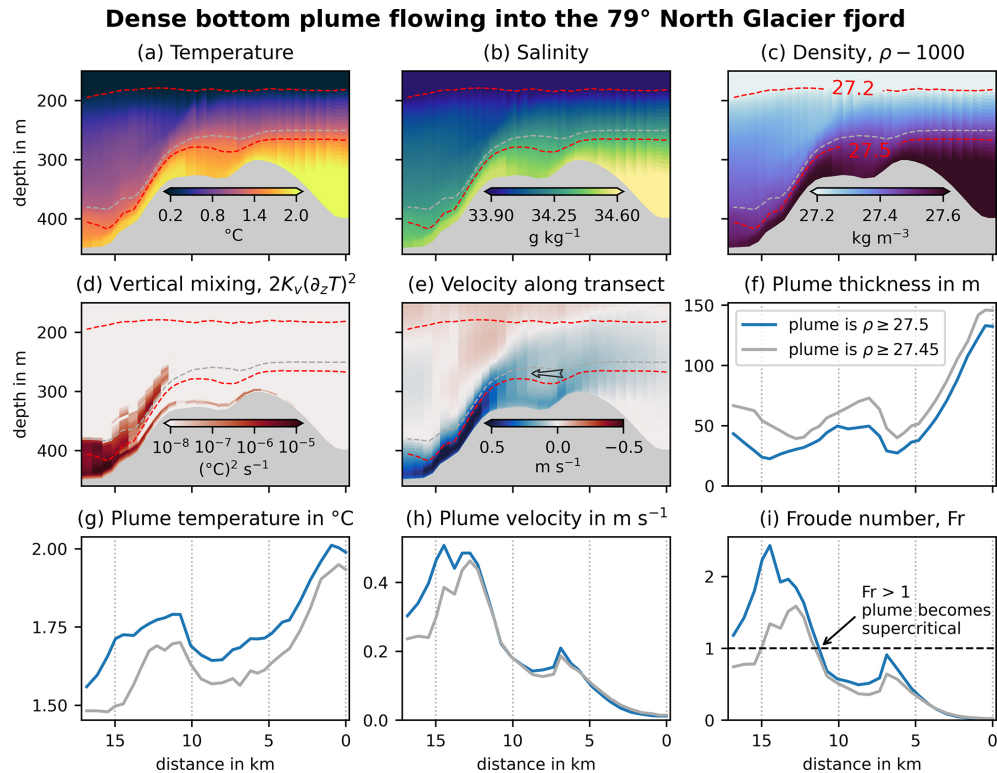
Figure 6. Properties of the inflow into the 79NG fjord along the transect marked in Fig. 5a. Panels (a)–(e) show vertical profiles of temperature (a), salinity (b), density anomaly (c), vertical turbulent mixing of temperature on a log scale (d), and flow velocity in the along-transect direction (e); red dashed lines mark the 27.2- and 27.5-isopycnals used to define the layers of ambient and plume water, see Sect. 2.4. Blue graphs in panels (f)–(i) show bulk properties of the plume: plume thickness (f), vertically averaged temperature (g), vertically averaged velocity (h), and Froude number (i). The sensitivity of the plume properties to the chosen plume interface is shown in gray, corresponding to the 27.45-isopycnal marked as gray dashed lines in panels (a)–(e). The x-axes of all panels show distance along the transect in the direction of the inflow, which is from right to left. Accordingly, positive velocities are also from right to left, as indicated by the arrow in (e). The sawtooth-like pattern visible in the first row is a visual artifact, because each grid cell is colored according to the value at the cell center, but model layers are tilted over sloping topography, resulting in visible differences between adjacent cells.
