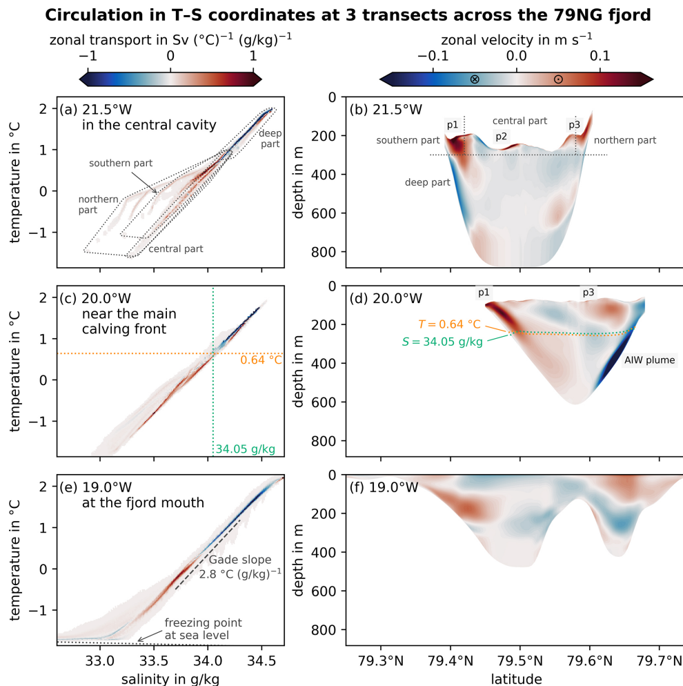
Figure 8. Overturning circulation in the 79NG fjord in temperature–salinity coordinates at three meridional transects: in the central cavity (a, b) and near the main calving front, inside (c, d) and outside (e, f) the cavity. The left column shows the zonal volume transport binned in temperature- and salinity-classes, the right column shows the corresponding zonal velocities in physical coordinates with positive velocities in the out-of-screen direction. The parts of the T – S diagram annotated in (a) correspond approximately to the areas marked in (b). The dividing salinity and temperature marked in (c) correspond to the isohaline and isotherm drawn in (d). The dotted line in (e) shows the freezing temperature at sea level pressure; note that lower temperatures can exist under the ice (e.g., in panel c) due to higher pressure. The labels p1–p3 mark the subglacial plumes annotated in Fig. 4.
