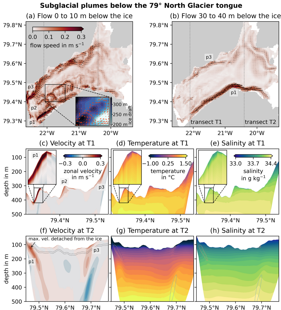
Figure 4. Details of the subglacial meltwater plumes below the 79NG ice tongue: the southern (p1), central (p2) and northern plume (p3). (a) Velocity of the flow averaged over the 10 m directly below the ice tongue; panel (b) is the same for the range of 30 to 40 m below the ice. The inset in (a) shows how the flow turns around cone-like features in the ice topography; the area shown in the inset is about 13 km \times 10 km wide. For the transect T1 marked in (a) and (b) , vertical profiles are shown in (c) , (d) , (e) for zonal velocity, temperature and salinity, respectively; panels (f) – (h) are analogous for transect T2. Zoomed insets in (c) – (e) show the fine vertical model resolution in the plume. Dotted lines in (f) mark the 30–40 m-range shown in (b) . The \pm 0.1 \text{ m s}^{-1} velocity contours are shown in (g) and (h) for orientation.
