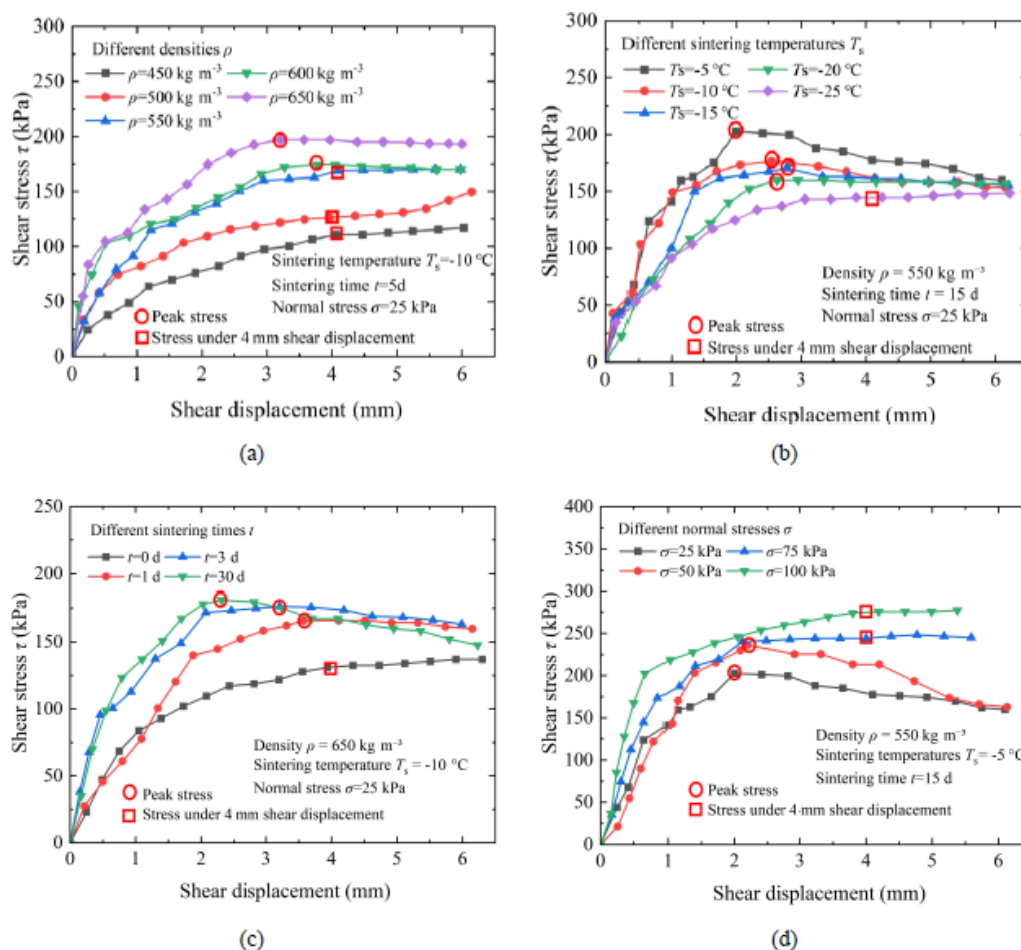
Figure 7. Shear stress–displacement curves under different test conditions (a, different densities; b, different sintering temperatures; c, different sintering times; d, different normal stresses).
