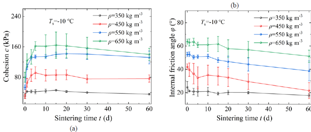
Figure 14. Variation of shear strength parameters with different sintering times under sintering temperature of -10^\circ\text{C} (a, cohesion c ; b, internal friction angle \varphi ).
