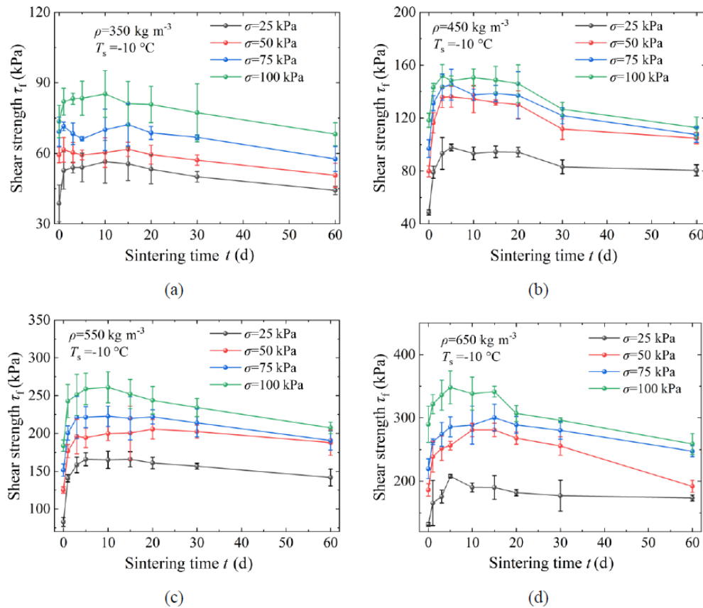
Figure 13. Variation of shear strength \tau_f with different sintering times under sintering temperature of -10^\circ\text{C} (a, \rho = 350 \text{ kg m}^{-3} ; b, \rho = 450 \text{ kg m}^{-3} ; c, \rho = 550 \text{ kg m}^{-3} ; d, \rho = 650 \text{ kg m}^{-3} ).
