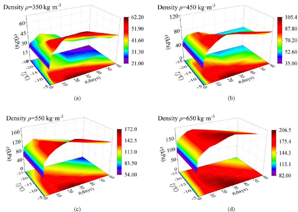
Figure 22. Predicted cohesion c values for various combinations (a, \rho = 350 \text{ kg m}^{-3} ; b, \rho = 450 \text{ kg m}^{-3} ; c, \rho = 550 \text{ kg m}^{-3} ; d, \rho = 650 \text{ kg m}^{-3} ).
