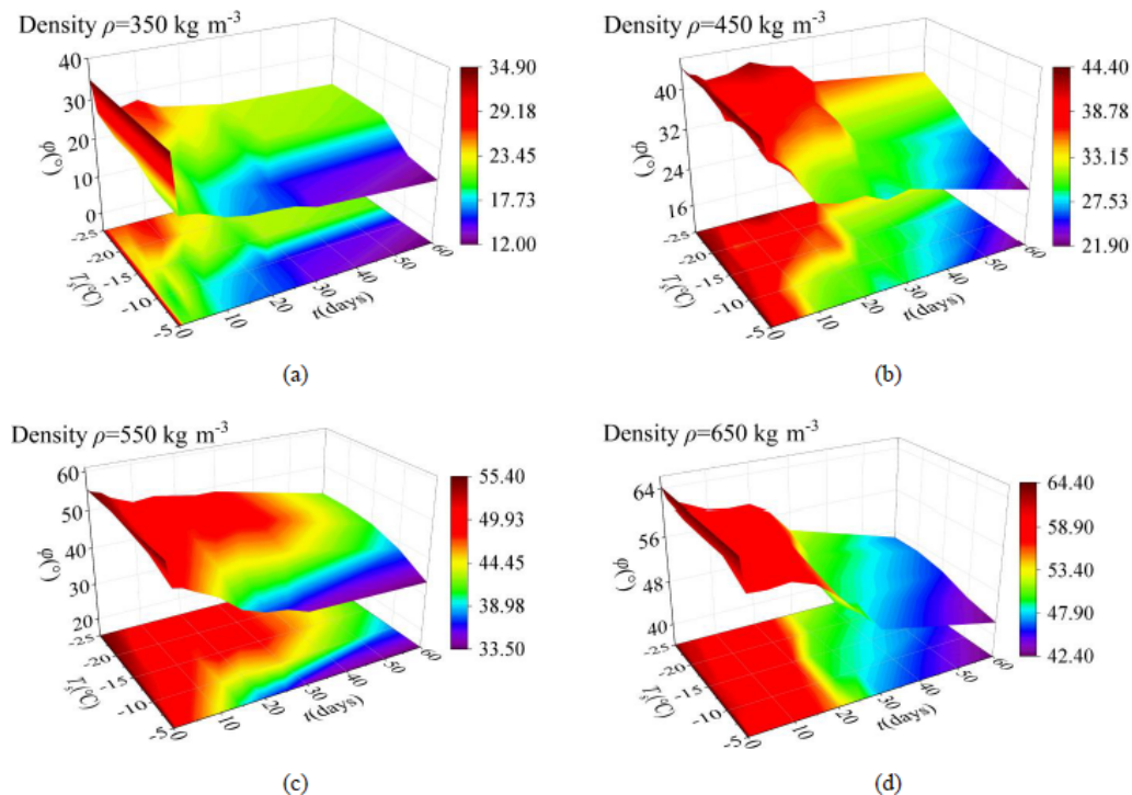
Figure 23. Predicted internal friction angle \varphi values for various combinations ( a , \rho = 350 \text{ kg m}^{-3} ; b , \rho = 450 \text{ kg m}^{-3} ; c , \rho = 550 \text{ kg m}^{-3} ; d , \rho = 650 \text{ kg m}^{-3} ).
