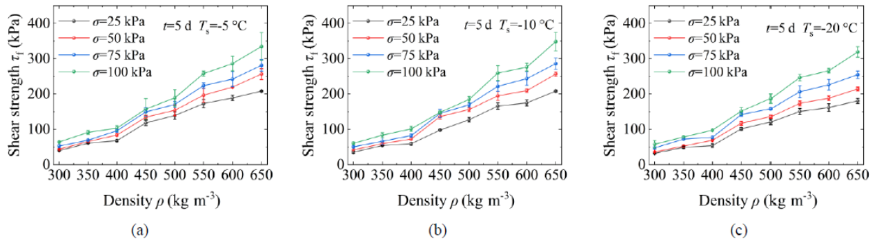
Figure 10. Variation of shear strength with initial density under different normal stresses after 5 d ( a , T_s = -5^\circ\text{C} ; b , T_s = -10^\circ\text{C} ; c , T_s = -20^\circ\text{C} ).
