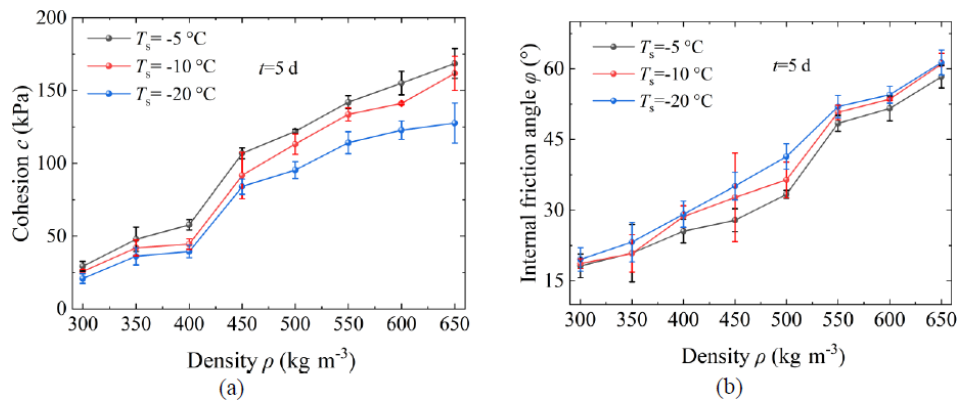
Figure 11. Variation of shear strength parameters at different initial densities after 5 d ( a , cohesion c ; b , internal friction angle \varphi ).
