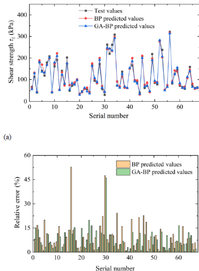
Figure 20. Shear strength prediction errors of the neural network model on the test set (a, Prediction value error; b, relative error of prediction value).
