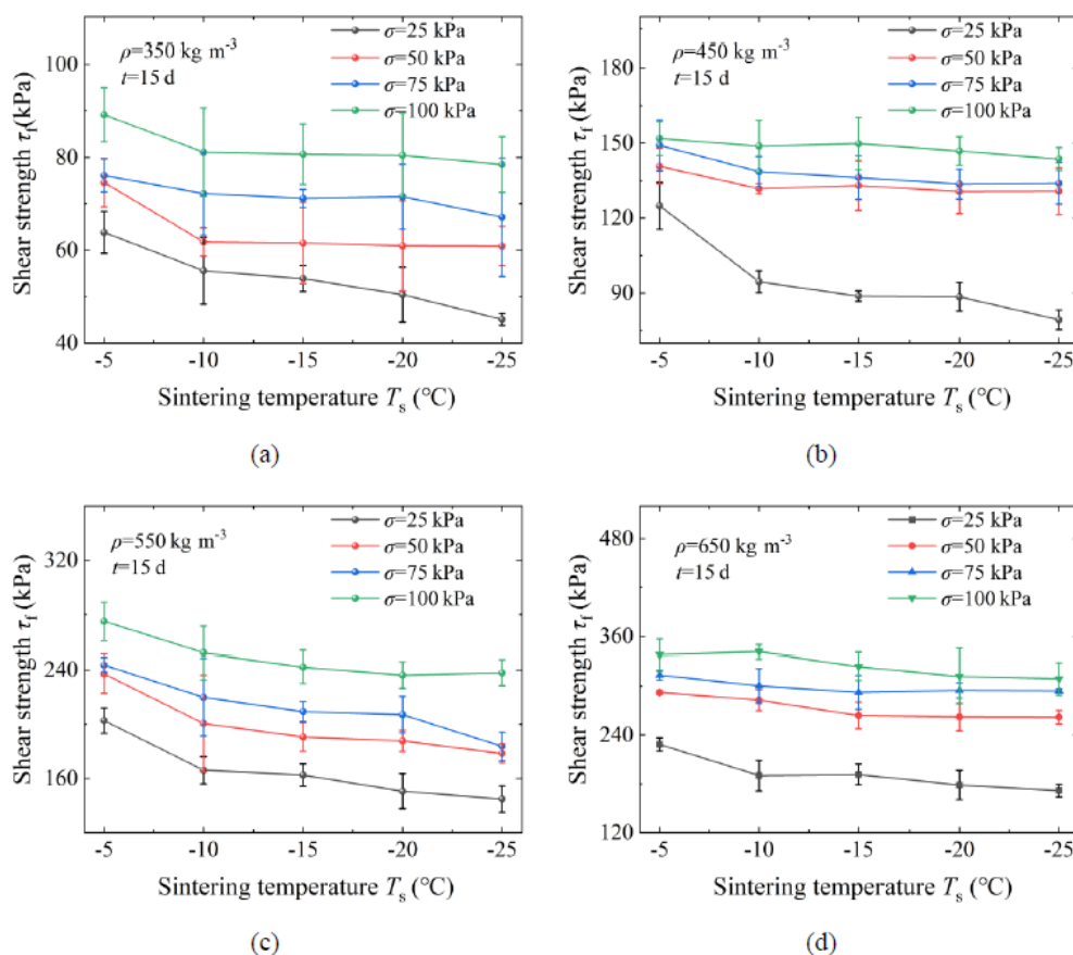
Figure 15. Variation of shear strength \tau_f at different sintering temperatures after 15 d (a, \rho = 350 kg m -3 ; b, \rho = 450 kg m -3 ; c, \rho = 550 kg m -3 ; d, \rho = 650 kg m -3 ).
