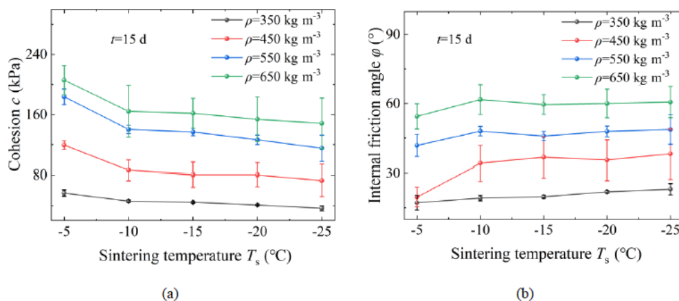
Figure 16. Shear strength at different sintering temperatures after 15 d (a, cohesion c ; b, internal friction angle \varphi ).
