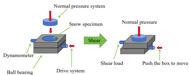
Figure 3. Shearing process.
