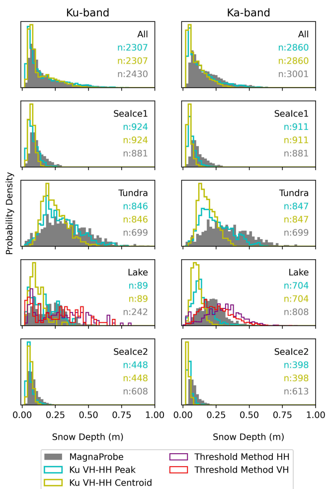
Figure 10. Histograms of snow depths from MagnaProbe (gray), peak differences (blue) and centroid method (yellow) for each surface type collected in April 2025 near Resolute Bay. Top panel shows results for all surfaces combined. Note there are slightly different number of data points between Ku- and Ka-band because of data outages and slight differences in the sampling between the frequencies.
