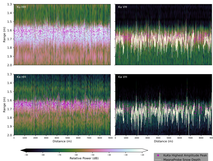
Figure A10. KuKa data echograms from 11 December 2021 over landfast sea ice. Shown are the Ku- and Ka-band (top and bottom panels) full bandwidth, HH- and VH-polarized (left and right panels) waveforms. Magenta markers indicate where the highest amplitude peak occurs in each radar waveform. Light yellow lines indicate MagnaProbe snow depths overlaid on the VH data; MagnaProbe depths were divided by c' to scale them to account for the reduced speed of radar wave propagation in the snow pack.
