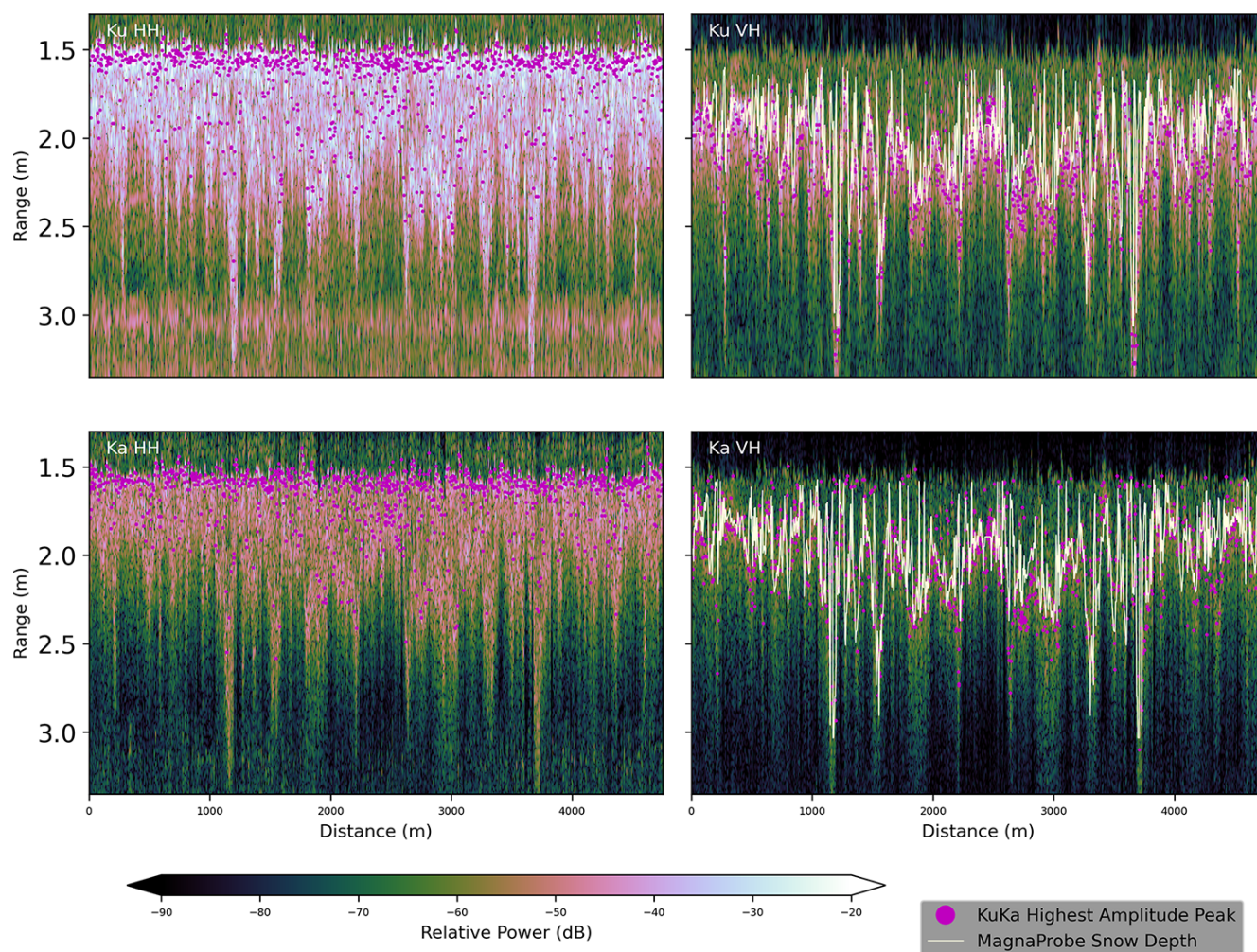
Figure 9. As in Fig. 7, but for tundra areas sampled in Resolute on 4 April 2025.
