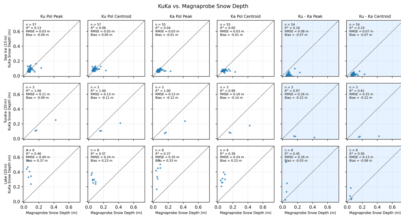
Figure 13. Same as in Fig. 12 but for the data collected near Churchill in December 2021.
