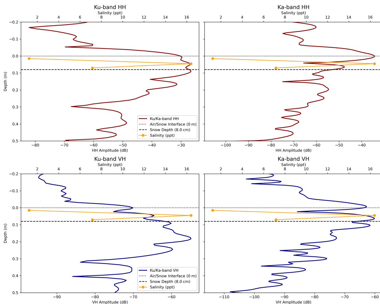
Figure 16. Same as in Fig. 15 but from the 4th snow pit collected on 2 April 2025 where a higher salinity layer is observed at intermediate depth in the snowpack.
