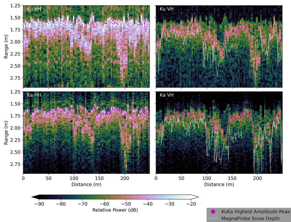
Figure A11. Same as Fig. A10 but for tundra on 6 April 2021.
