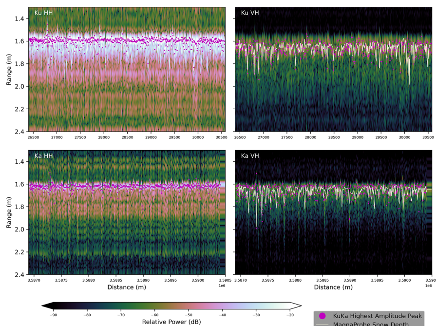
Figure A9. Echograms at Ku- (left) and Ka-band (right) from 6 April 2025 over the second Resolute landfast sea ice location. Shown are the full bandwidth data for HH and VH-polarizations. Magenta markers indicate where the highest amplitude peak occurs in each radar waveform. Yellow lines indicate MagnaProbe snow depths overlaid on the VH data; MagnaProbe depths were divided by c' to scale them to account for the reduced speed of radar wave propagation in the snow pack.
