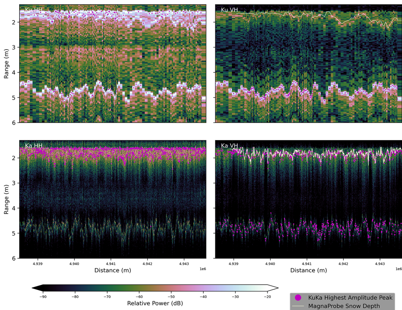
Figure 8. As in Fig. 7, but for Lake Resolute data on 5 April 2025. Note that the distance is not identical for Ku- and Ka-band as a result of Ku-band recording stopping during part of the transect. Note also the deeper ranges plotted compared to Fig. 7.
