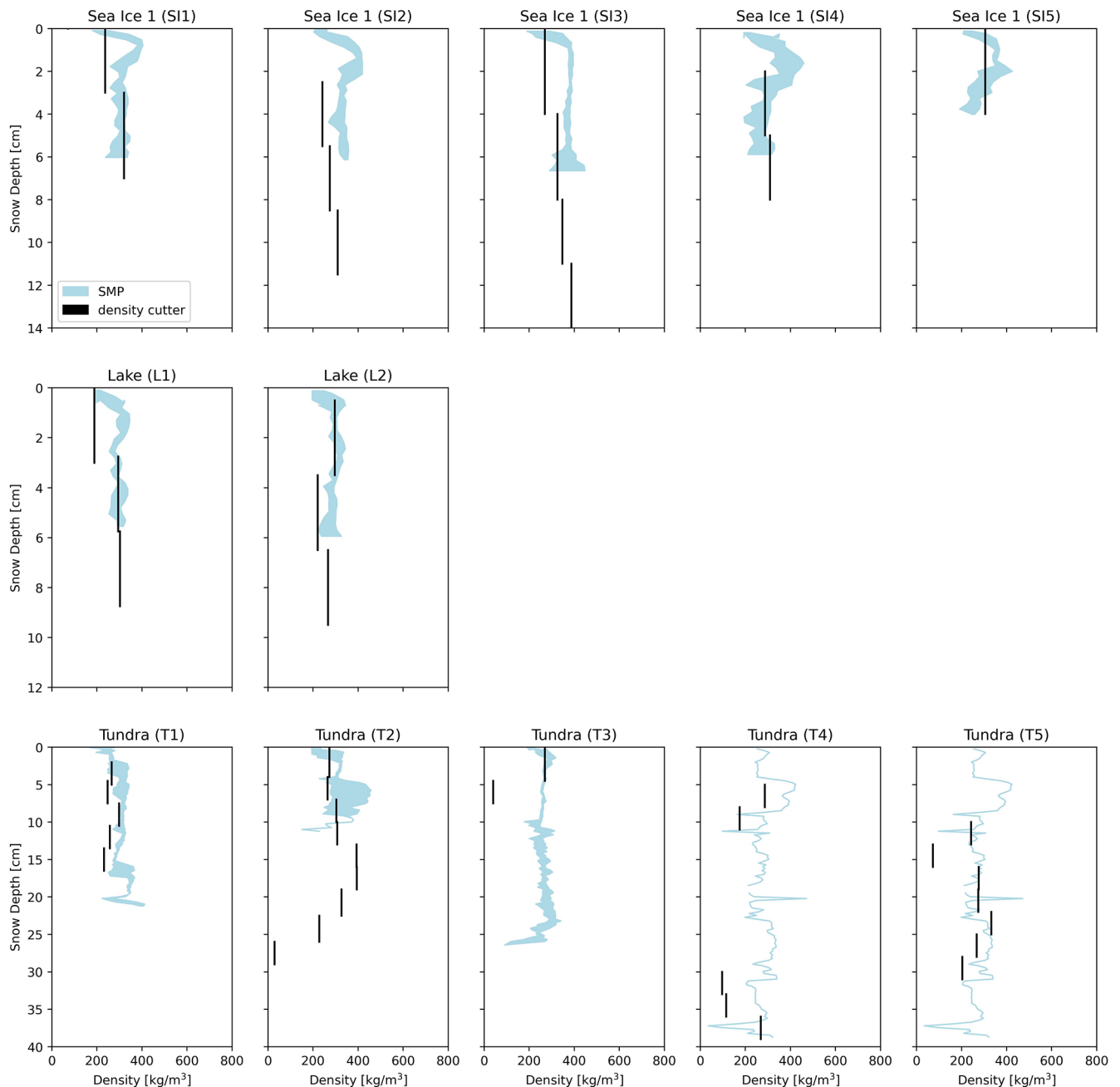
Figure 5. Comparison of SMP-derived density profiles (following King et al., 2020) and those derived using a density cutter. Note the vertical axis is reversed compared to Fig. 4 as the total snow height measured by the SMP was sometimes not achieved due to incomplete penetration of the SMP. All data shown here were collected during the Resolute field campaign.
