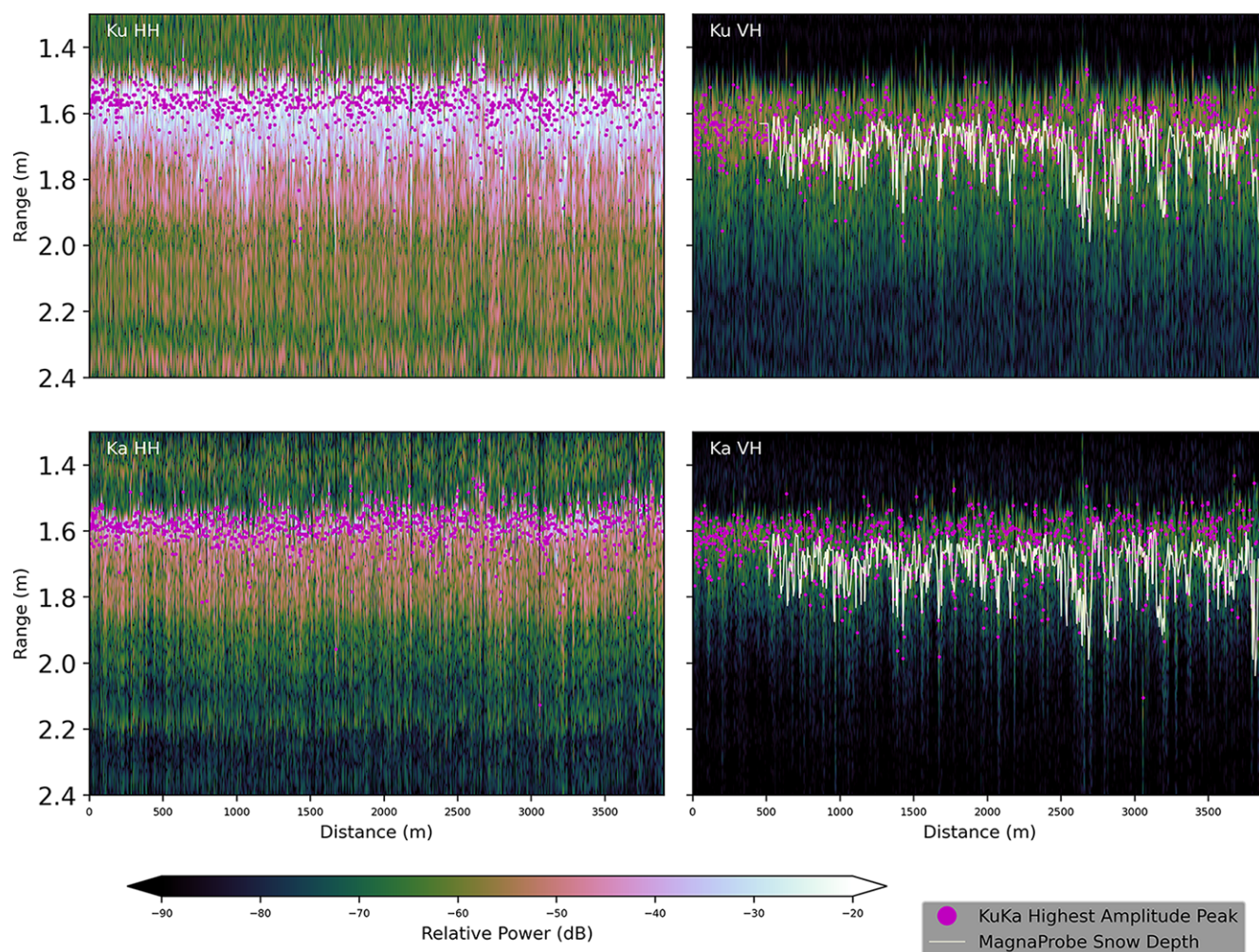
Figure 7. KuKa data echograms from 2 April 2025 over landfast sea ice in Resolute Bay. The vertical axis represents the radar range, defined as the distance from the antenna phase center to the scattering target. Shown are the Ku- and Ka-band (top and bottom panels) full bandwidth, HH- and VH-polarized (left and right panels) waveforms. Magenta markers indicate where the highest amplitude peak occurs in each radar waveform. Light yellow lines indicate MagnaProbe snow depths overlaid on the VH data; MagnaProbe depths were divided by c' to scale them to account for the reduced speed of radar wave propagation in the snow pack and referenced from a constant height of 1.56 cm (estimated distance from snow to radar).
