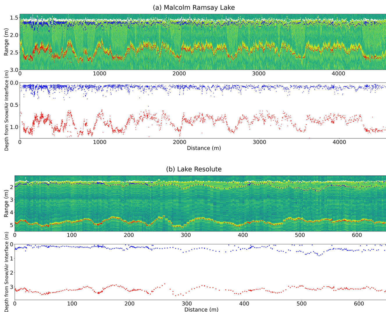
Figure 17. Echograms and corresponding derived lake ice thickness (red) and snow depth (blue) from Malcolm Ramsay Lake (a) and Lake Resolute (b).
