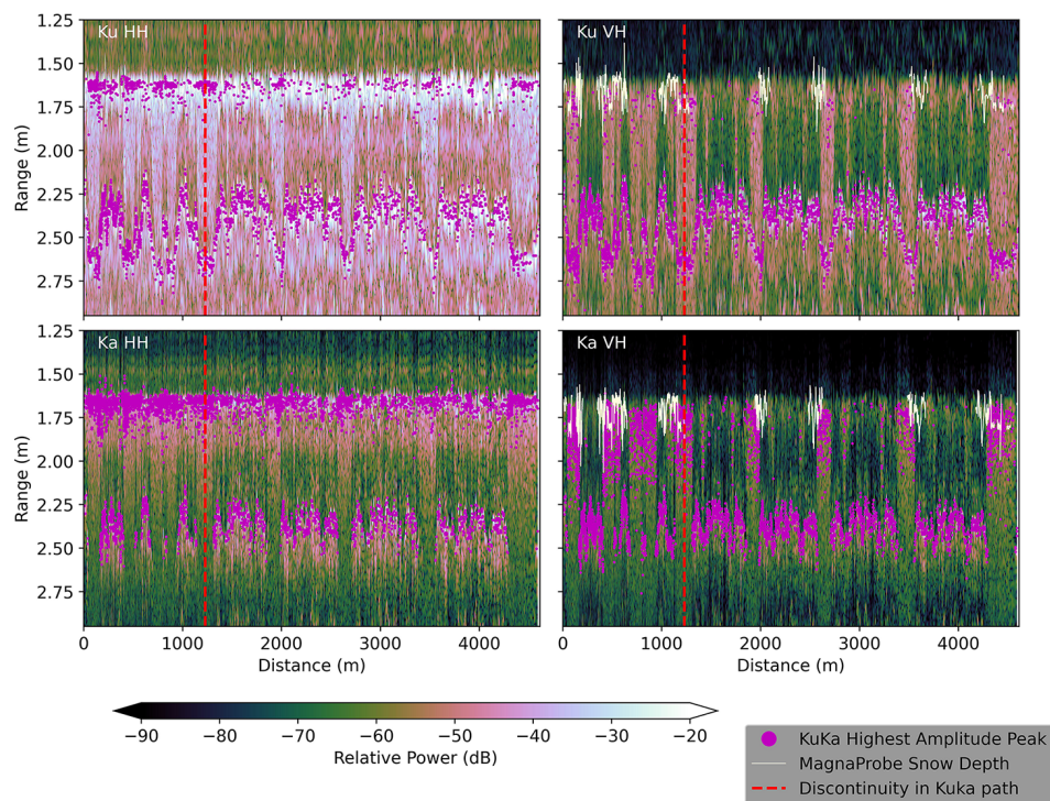
Figure A12. Same as Fig. A10 but for Lake ice on 4 December 2021. For this case, the HH polarization maximum is not consistently found at the air-snow interface, therefore the air-snow threshold value as defined in Table 2 was used for the plotting of this echogram.
