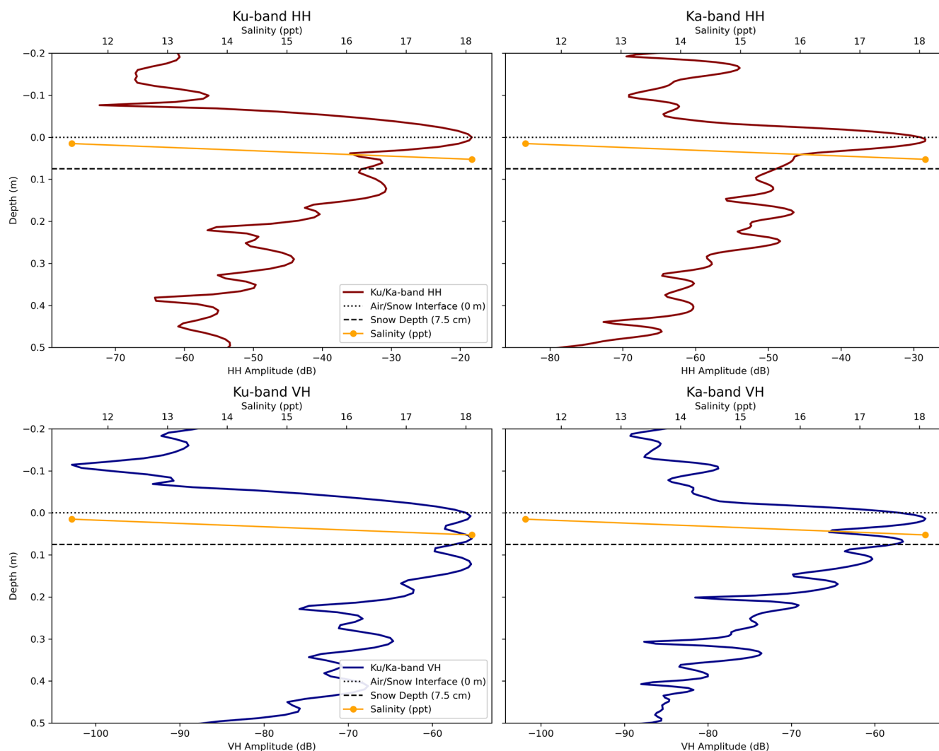
Figure 15. Waveforms from the 6th snow pit collected on 2 April 2025 where a higher salinity layer is observed just above the ice surface. Plotted with the Ku-band (red) and Ka-band (blue) HH and VH waveforms in dB is the salinity profile measured at 3 cm intervals. Results are shown as the average for the 5 closest waveforms to the snow pit location.
