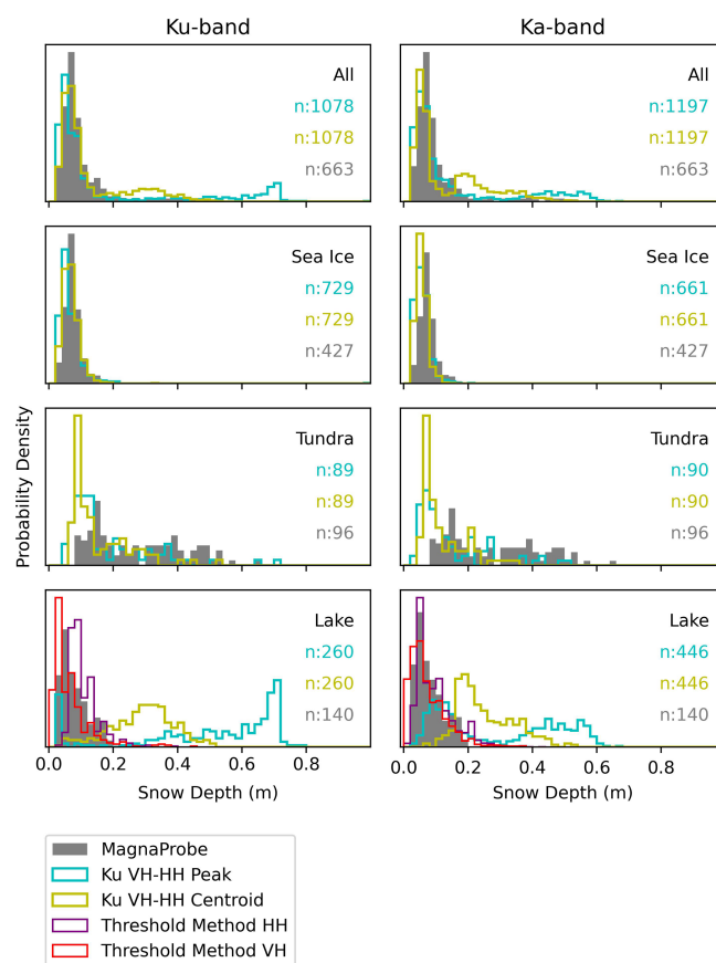
Figure 11. As in Fig. 10 but for each surface type collected in December 2021 near Churchill.
