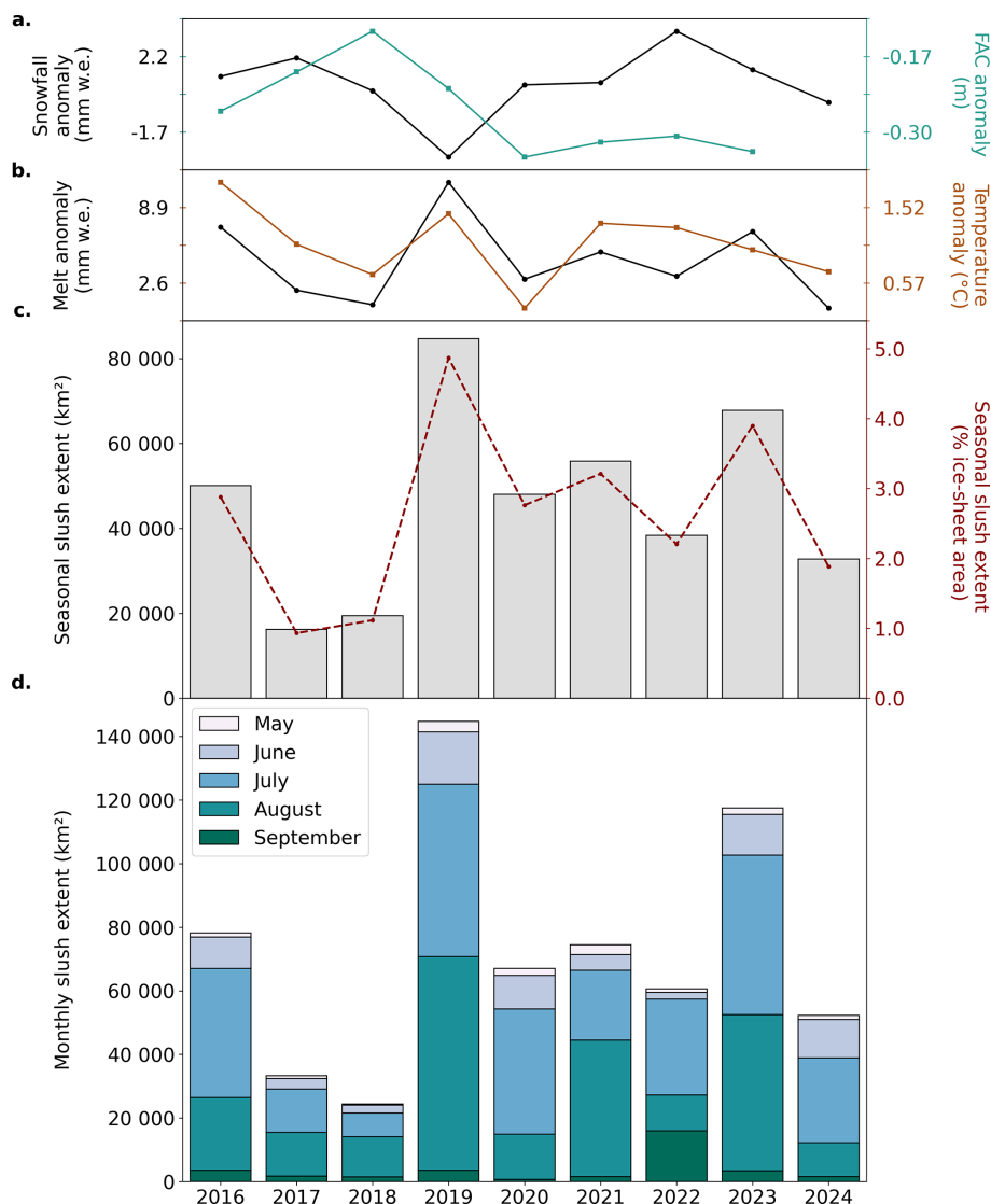
Figure 4. Mean annual climate and slush variability across the GrIS from 2016–2024. (a) Ice-sheet-wide mean snowfall anomalies (black) and FAC anomalies (teal) relative to the 1960–1989 mean. (b) Ice-sheet-wide mean snowmelt anomalies (black) and 2 m air temperature anomalies (orange) relative to the 1960–1989 mean. (c) Seasonal slush extent for May–September, shown as absolute area (left y-axis, grey bars) and as a percentage of total ice-sheet area (right y-axis; dashed dark-red line). (d) Stacked monthly slush extent for May–September in each year (note: monthly segments are not spatially additive). Snowfall, snowmelt, and 2 m air temperature are derived from RACMO, while FAC is derived from the IMAU-FDM (available through 2023 only).
