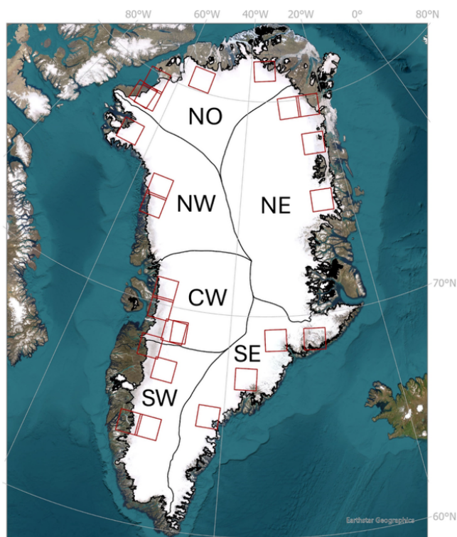
Figure 2. Overview map of the GrIS divided into six drainage basins: SW, CW, NW, NO, NE, and SE (Mouginot and Rignot, 2019). Red boxes indicate the footprints of the 24 S2 images used in this study for classifier development and evaluation: 18 for training and internal validation of the RF classifier and a further 6 for comparison with threshold-based classification methods. Base map source: Esri (2024) Earthstar Geographics | Powered by Esri.
