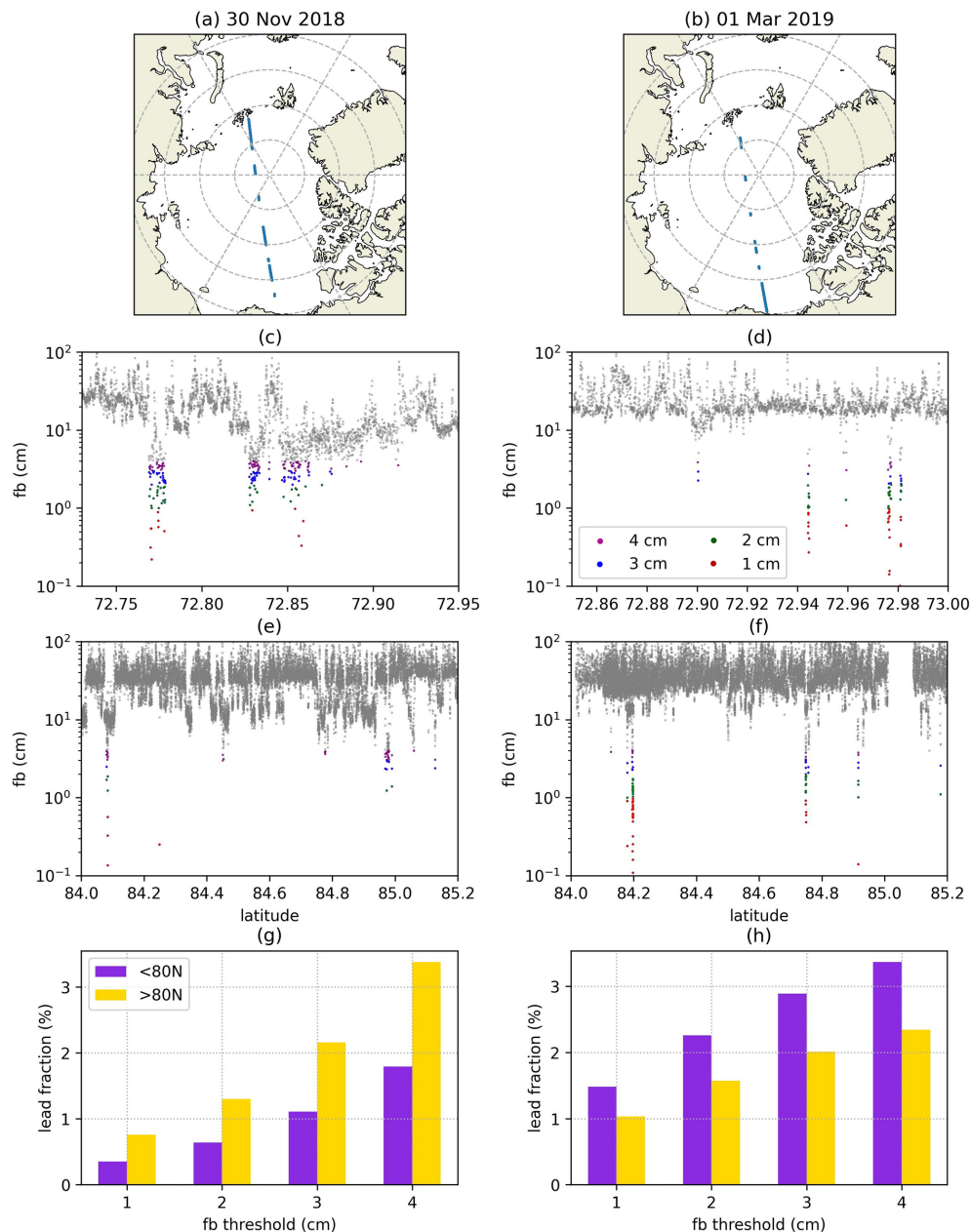
Figure 8. (a, b) Selected ICESat-2 track on (a) 30 November 2018 and (b) 1 March 2019. Only segments with freeboard less than 5 m and the quality check passed are shown. The total numbers of segments are 178594 on 30 November 2018 and 131663 on 1 March 2019. (c, f) Snapshots of freeboard over the part of the track with (c, d) thinner and thicker (e, f) ice in (c, e) November and (d, f) March. (g, h) Along-track lead fraction in regions of (g) thinner (south of 80°) and (h) thicker (north of 80°) ice.
