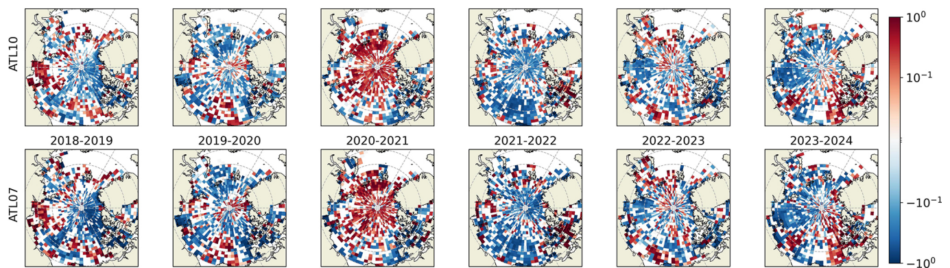
Figure 5. Lead fraction anomaly relative to their climatology (%) in each winter from (top row) ATL10 and (bottom row) ATL07. Only grid cells with the same signs in lead fraction anomaly derived from the two products are shown, highlighting features that are consistent between the two products.
