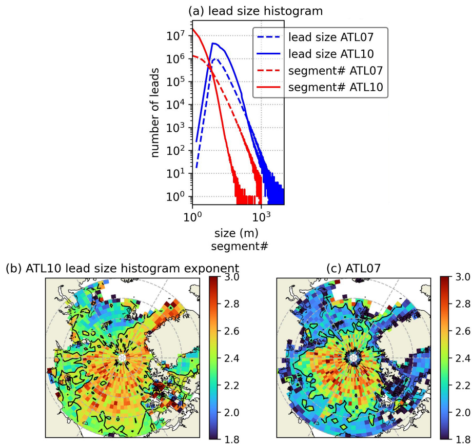
Figure 4. (a) Histogram of individual lead size (blue) and the number of segments that consist of a single lead (red), from ATL07 (dashed) and ATL10 (solid). (b–c) Exponents of the power-law distribution of lead size estimated between lead size of 20 and 100 m in (b) ATL10 and (c) ATL07. Only cells with p -value < 0.05 when estimating histogram slopes are shown.
