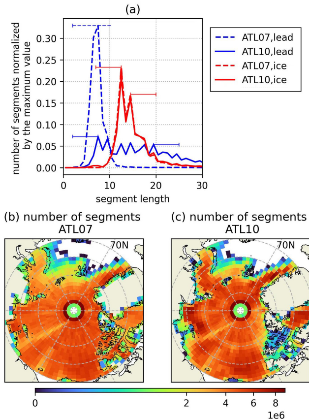
Figure 2. (a) Histogram of length of a single lead (blue) and ice (red) segment in ATL07 (dashed) and ATL10 (solid). Error bars represent half of the ICESat-2 footprint size (5.5 m). (b–c) Total number of segments in grid cells of 1^\circ longitude \times 4^\circ latitude in the winter of 2018–2024 in (b) ATL07 and (c) ATL10.
