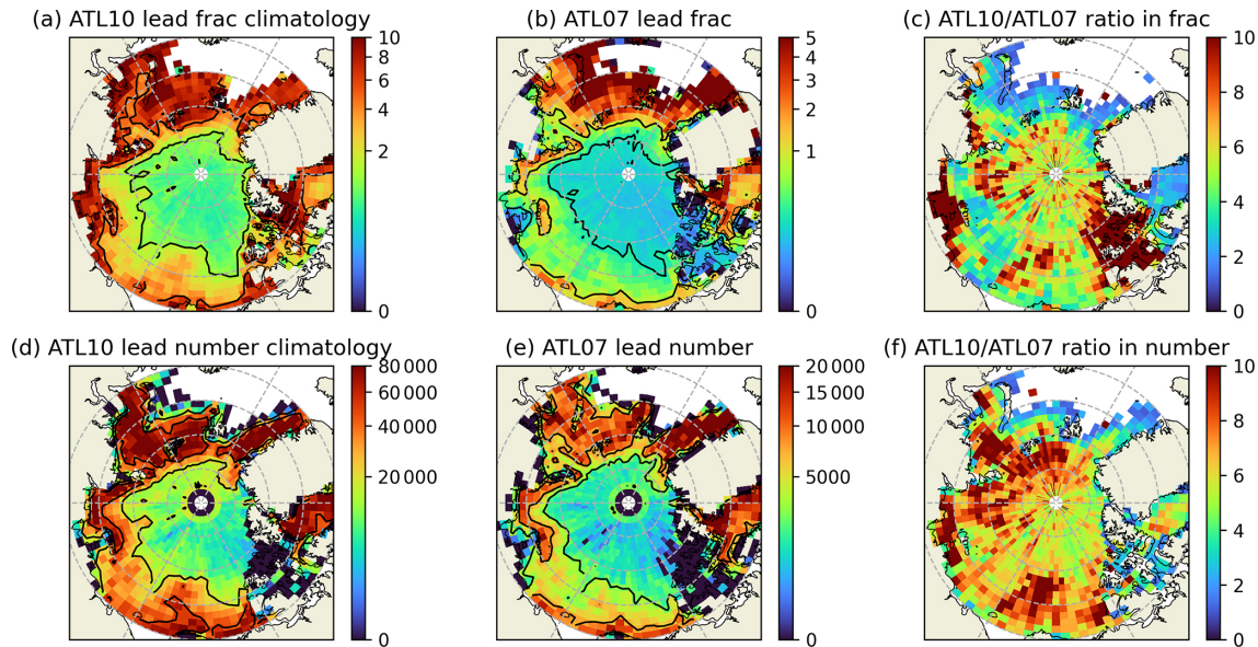
Figure 3. (a, b, d, e) Climatological wintertime (a, b) lead fraction and (d, e) lead number in (a, d) ATL10 and (b, e) ATL07. Contours in (a) and (b) indicate 1.3 % and 5 %, and 0.2 % and 1 %. Contours in (d) and (e) indicate 20 000 and 50 000, and 3000 and 7500. (c, f) The ratio of (c) lead fraction and (f) number in ATL10 to those in ATL07.
