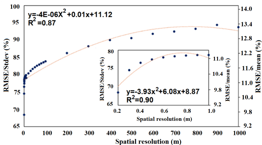
Figure 6. ALT uncertainties change with spatial resolutions from 0.2 to 1000 m with a detailed subset analysis from 0.2 to 1 m (inset). The uncertainties were determined using the 0.1 m ALT benchmark and normalized by the standard deviation (left vertical axis) and mean (right vertical axis; fitted polynomial function) of the 0.1 m ALT values.
