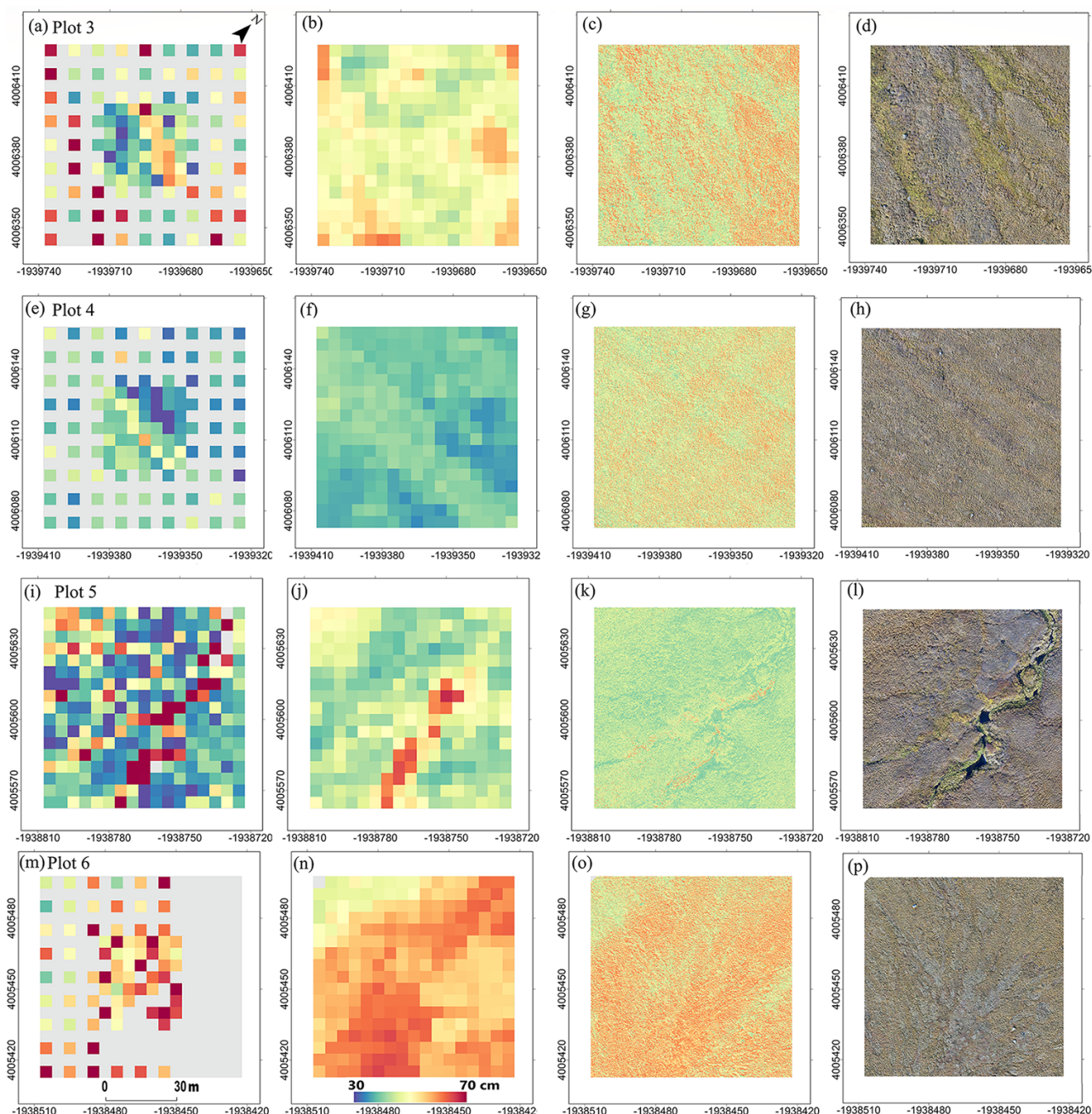
Figure 4. Comparisons of ALT spatial patterns derived from field measurements ( a, e, i, m ; grey shading indicates areas without sampling), 5 m ML outputs ( b, f, j, n ), and 0.1 m ML estimates ( c, g, k, o ), and images acquired from drone-based RGB camera ( d, h, l, p ) for the intensively sampled plots. The map was plotted using Canada Albers Equal Area Conic projection.
