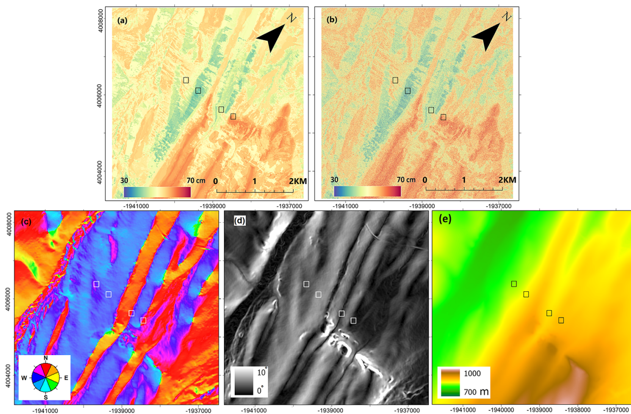
Figure 5. Comparisons between ALT distributions at 10 m resolution derived from ML (a), the synthetic ALT map at 0.1 m resolution (b), terrain aspect (c), slope (d), and elevation (e) over a larger 5 km × 5 km area surrounding the sampling plots (black rectangles). The map was plotted using Canada Albers Equal Area Conic projection.
