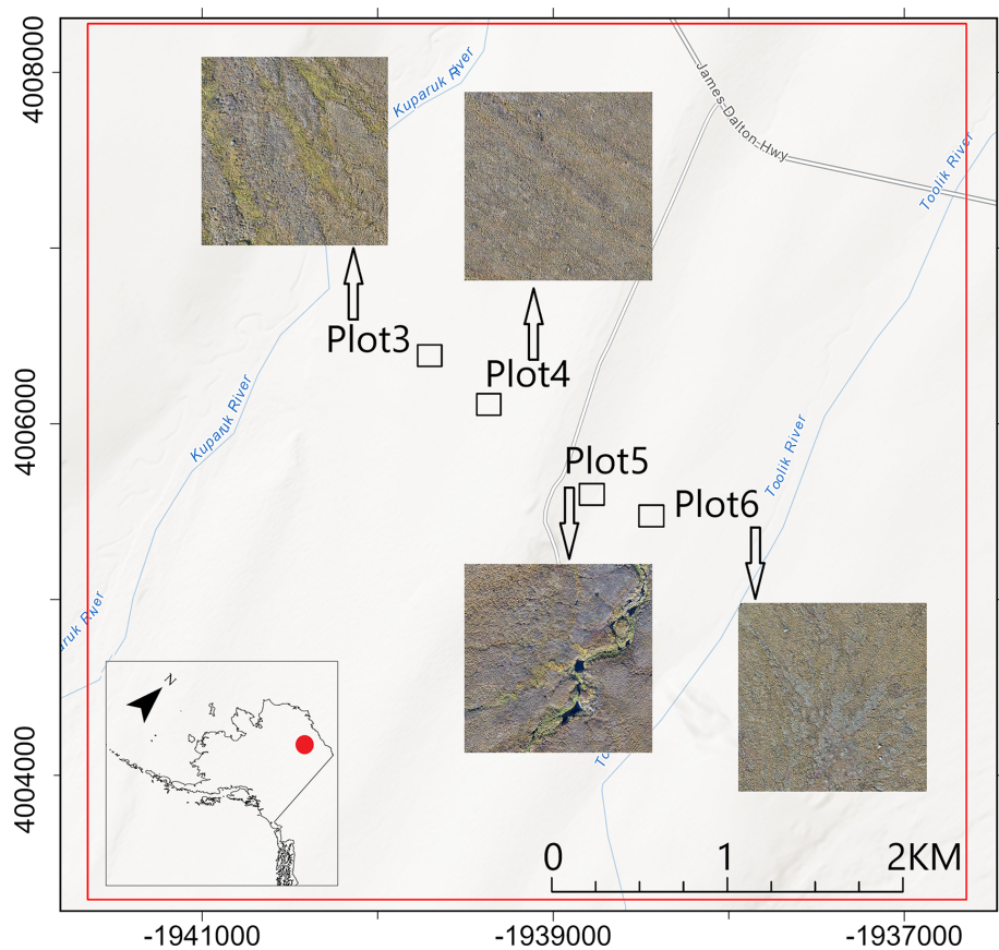
Figure 1. The study region encompasses an Arctic tundra area (68.6167° N, 149.3167° W; red dot in the inset) in the northern foothills of the Brooks Range, Alaska. The region consists of four intensively sampled plots (Plot 3, Plot 4, Plot 5, and Plot 6; 90 m × 90 m each) with their corresponding true-color RGB (red-green-blue) drone images displayed alongside for visual inspection only, and surrounded by a larger 5 km × 5 km study region (red rectangle) used for analyzing ALT scaling effects. The map was plotted using Canada Albers Equal Area Conic projection.
