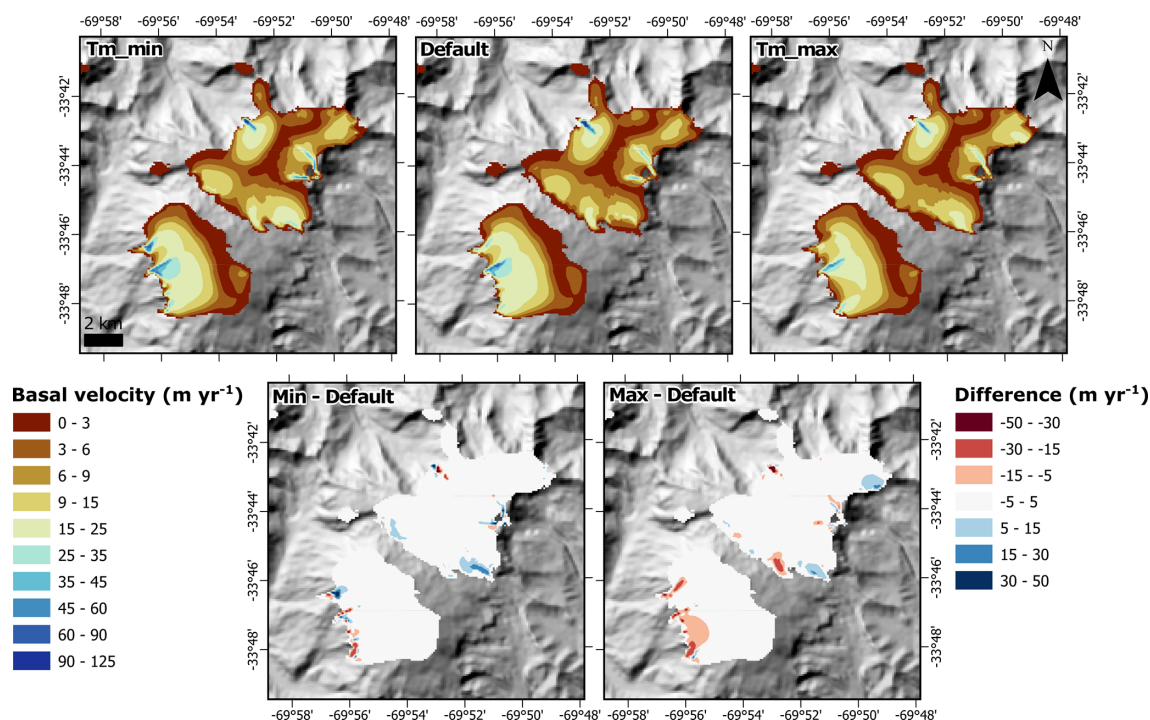
Figure 8. An example of the influence of the W_{\text{till}}^{\text{max}} (Tm in figure panels) parameter on the output of ice basal velocity in the Mendoza, Maipo, and Rapel (#5) domain (Volcán Marmolejo). Remaining examples are shown in the Supplement. Increased values the Tm parameter generally sees no, or very little changes in basal ice velocities. Values that correspond to “max” and “min” parameter values are found in Table 1.
