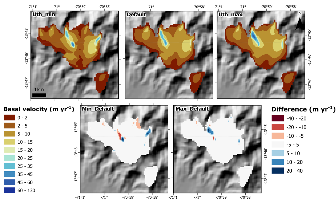
Figure 11. An example of the influence of the u_{\text{threshold}} (Uth in figure panel) parameter on the output of ice basal velocity in the Vilcanota (#2) domain (Quelccaya Ice Cap). Remaining examples are shown in the Supplement. An increase in the u_{\text{threshold}} parameter sees increased basal velocities, while the opposite is seen when values are decreased. Values that correspond to “max” and “min” parameter values are found in Table 1.
