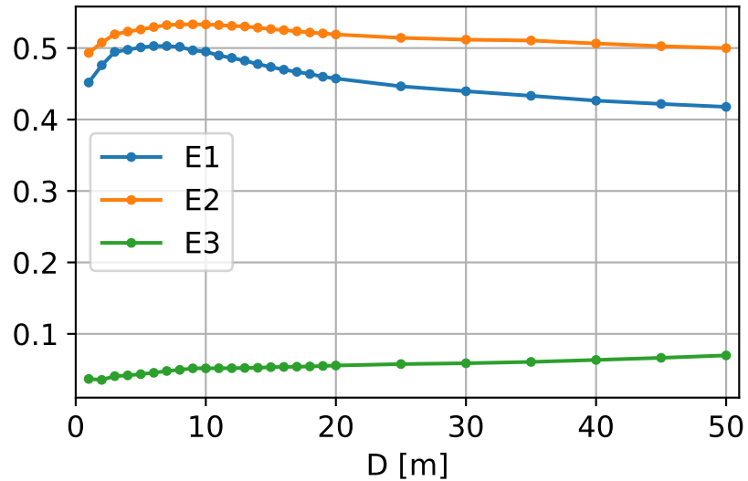
Spearman correlations Sx - \Delta HS
