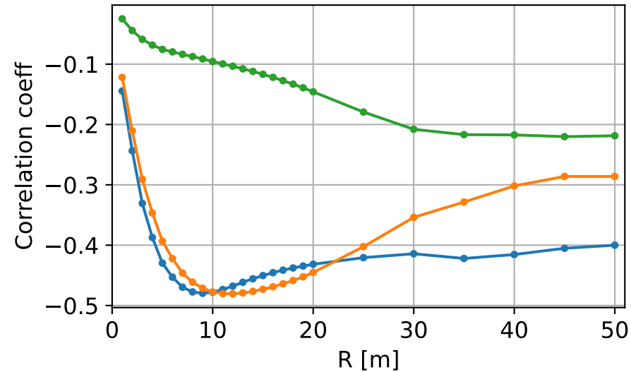
Spearman correlations TPI - \Delta HS
