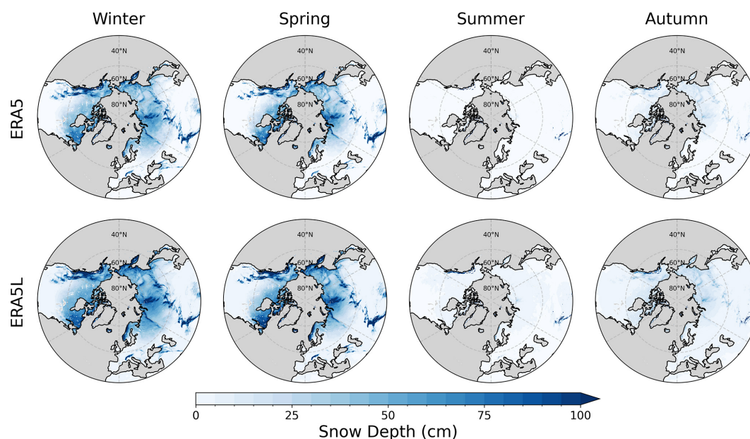
Figure B6. Comparison of the seasonal climatology (1986–2022) of SD over mid- to high-latitude regions (30–90° N) of the Northern Hemisphere between ERA5 (top row) and ERA5L (bottom row).
