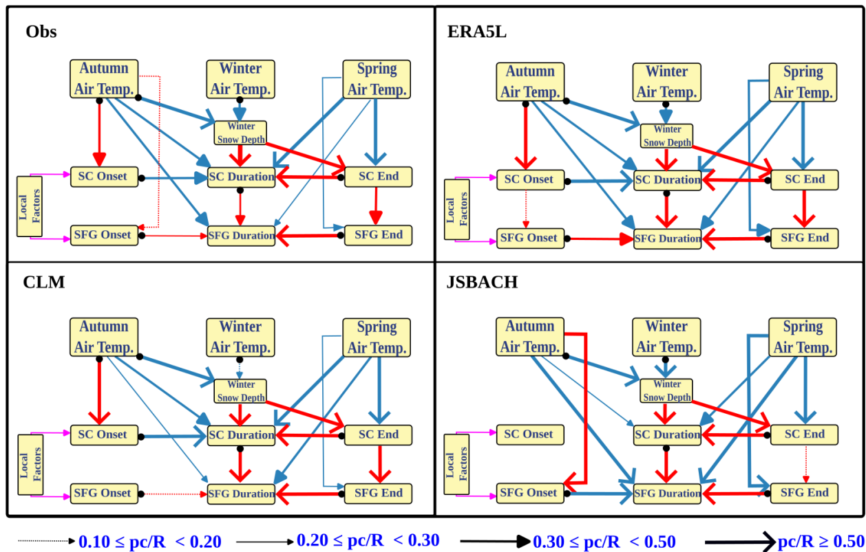
Figure 11. Schematic representation of the statistically significant Pearson and partial correlations derived from Appendix Table A3, illustrating the interactions among seasonal air temperature, snow cover, snow depth, and seasonally frozen ground characteristics for (a) OBS, (b) ERA5L, (c) CLM, and (d) JSBACH. Red and blue lines denote positive and negative correlations, respectively, while the magenta-coloured line indicates possible local influences affecting the variables. Filled circles at the arrow origin indicate Pearson correlation coefficients; all other values represent partial correlations.
