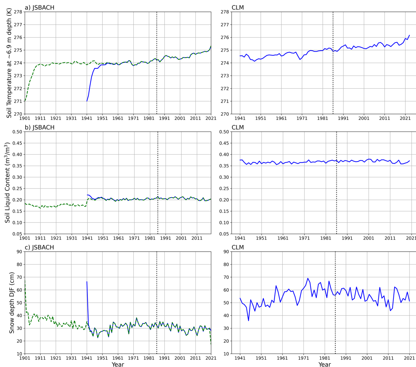
Figure B2. Time series of (a) winter mean soil temperature at 6.9 m depth, (b) summer mean volumetric soil liquid water content (0–1 m) ( \text{m}^3 \text{m}^{-3} ), and (c) winter mean snow depth, averaged over the region shown in Fig. B1, simulated by JSBACH (first column) and CLM5 (second column) for the period 1941–2022 (blue solid lines). In addition, an extended JSBACH simulation forced with GSWP3 (1901–1940) and subsequently ERA5 (1941–2022) is shown (green dashed line), which converges to the same trajectory as the standard simulation well before the start of the analysis period, indicating that the soil thermal and hydrological states become effectively independent of the initial conditions before 1986.
