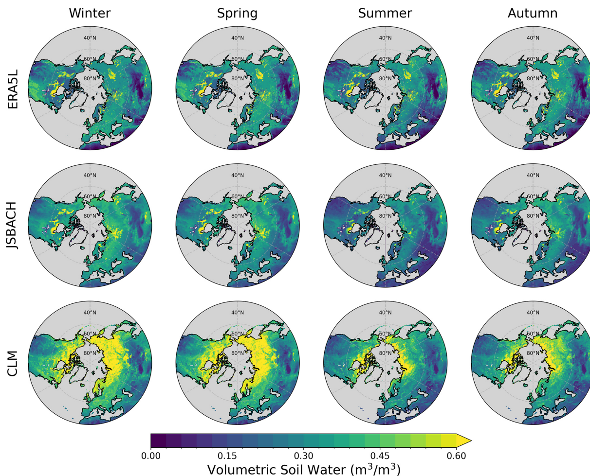
Figure 3. Seasonal climatology (1986–2022) of total soil moisture (liquid + ice) at 20 cm depth across Northern Hemisphere mid- to high-latitude regions (30–90° N), as simulated by ERA5L (top row), JSBACH (middle row), and CLM (bottom row).
