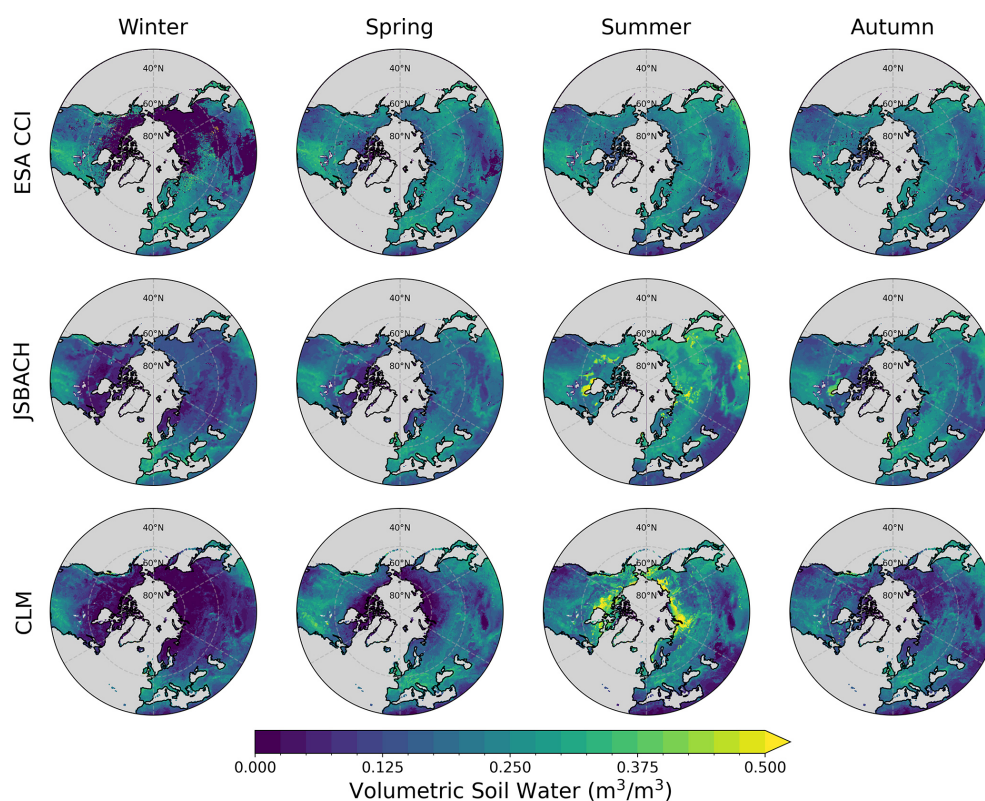
Figure B5. Comparison of the seasonal climatology (1986–2022) of top-layer soil liquid water content over mid- to high-latitude regions (30–90° N) of the Northern Hemisphere, as derived from satellite data (ESA-CCI; top row) and simulated by models: JSBACH (middle row) and CLM (bottom row).
