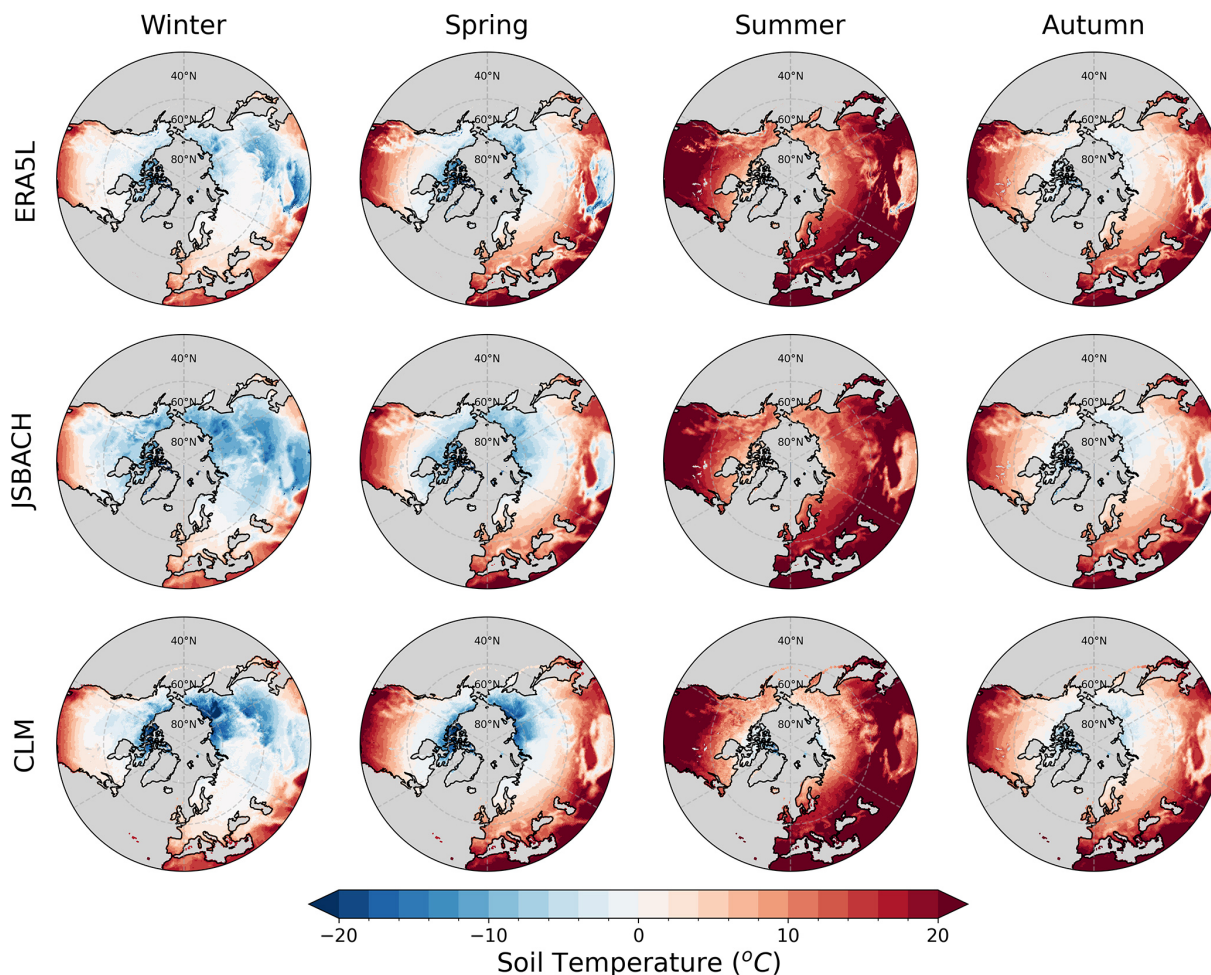
Figure 4. Same as Fig. 3 but for soil temperature at 20 cm depth.
