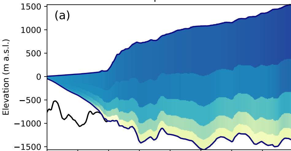
CCSM4-RCP8.5-2300 at 2150 with temperature solver
