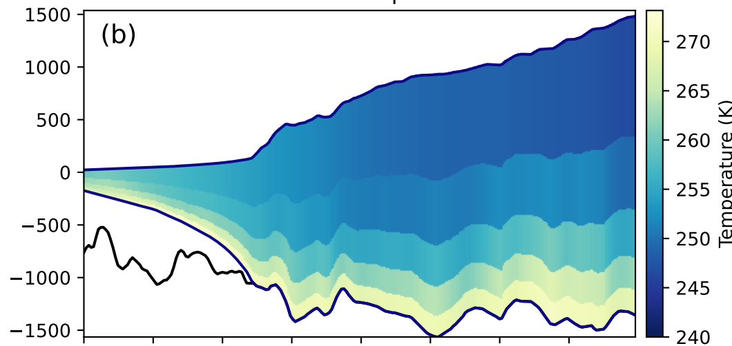
CCSM4-RCP8.5-2300 at 2150 with fixed temperature
