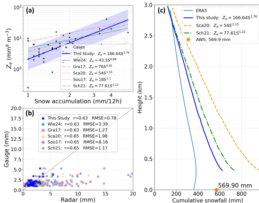
Figure 3. (a) Scatterplot of MRR equivalent reflectivity (linear units) versus 12 h snowfall accumulation from a standard weighing rain gauge (black dots), together with the Z_e – S relationship derived using DE regression (solid blue line). The blue shaded region represents the regression RMSE estimated in \ln(Z_e) space. Also shown are published Z_e – S relations from Wiener et al. (2024) (light-blue solid), Grazioli et al. (2017b) (red dashed), Scarchilli et al. (2020) (yellow dashed), Souverijns et al. (2017) (purple dashed) and Schoger et al. (2021) (green dashed). (b) Comparison between 12 h snowfall accumulation estimated from MRR reflectivity using the same Z_e – S relations as in panel (a) and the time-scheduled precipitation amounts recorded by the automatic weather station (scatterplot). (c) Cumulative snowfall profiles from ERA5 and from the MRR-based retrieval using the locally fitted relation (solid blue), together with profiles computed using the relations of Scarchilli et al. (2020) (yellow dashed) and Schoger et al. (2021) (green dashed).
