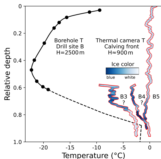
Figure 7. Temperature ( T ) and blue color index profiles scaled and located into the ice column. The icebergs B3, B4 and B5 from Fig. 3 are scaled and situated in the ice column to be compared with the temperature profile at drill site B (black line) and its extrapolation (dashed line) (Funk et al., 1994). Temperature is plotted on the horizontal axis as a function of relative depth. Ice color is represented by the color of the points (dark blue indicates blue ice). Vertical positions of B3 and B4 are uncertain.
