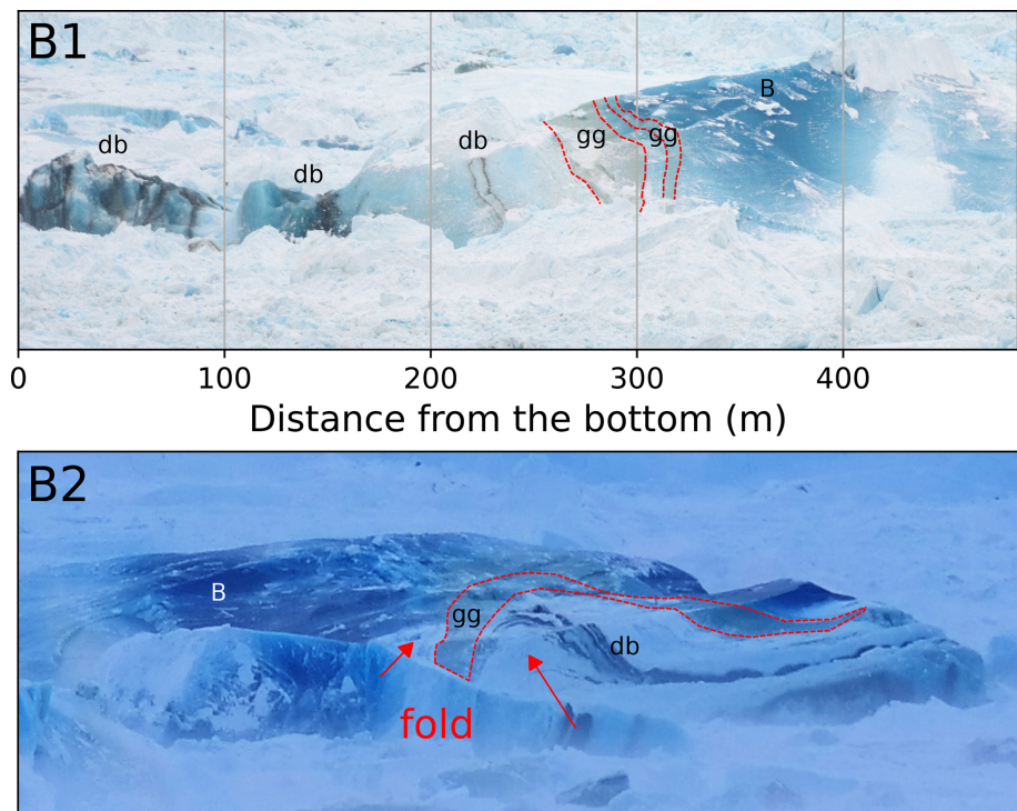
Figure 2. Icebergs B1 and B2 show large portions of blue (B) and green-greyish (gg, delimited in red) ice, and contain dark banded structures (db) and folds (red arrows). The scale in B2 could not be measured, but the displayed width amounts to \approx 500 m.
