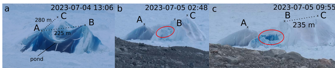
Figure 5. Evolution of the blue color of iceberg B6. Black crosses and dotted lines are used to show distances and orientation change of the iceberg. In panel (a), a pond is similar to those studied previously, except that here it is sea water trapped during calving, not melt water from the iceberg. In panel (b), an area about to collapse is circled in red. In panel (c), blue ice is revealed after the surface layer collapsed.
