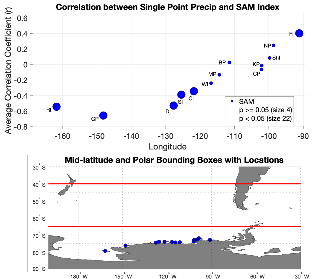
Figure 5. Correlation between precipitation at each ice rise and the Southern Annular Mode Index (Marshall, 2003). The index is defined by averaging MSLP across narrow latitude bands centered on -40 and -65^\circ (red lines) and calculating the difference.
