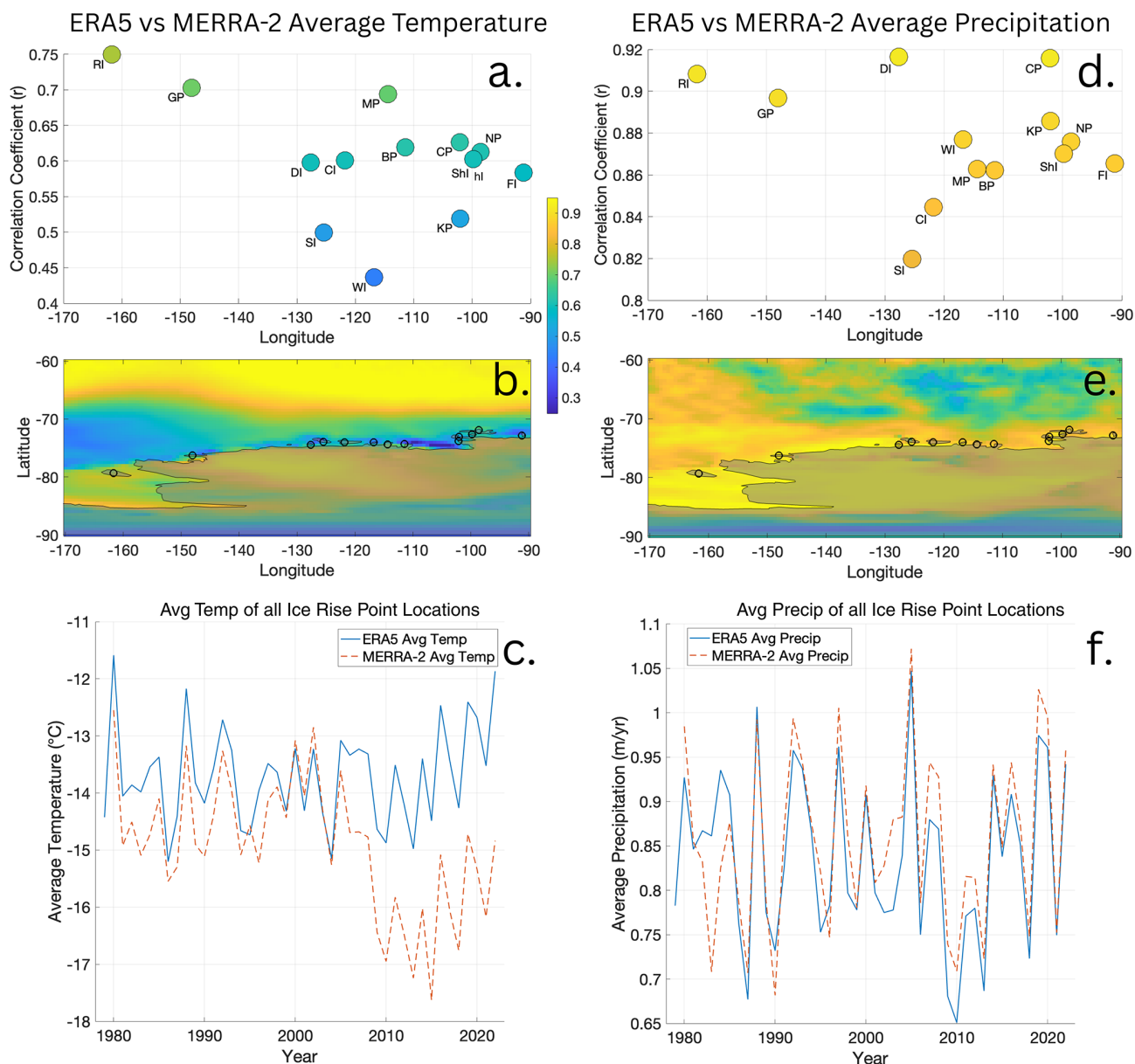
Figure 3. Correlation between ERA5 and MERRA-2 reanalysis datasets for temperature (a–c) and precipitation (d–f) at each ice rise for the 1979–2022 period. Panels (a), (b), (d), and (e) show a correlation field visualized with a color-coded heatmap (higher correlation coefficients in yellow, lower coefficients in blue) and the 13 ice rise locations plotted. Statistical significance of the ERA5 and MERRA-2 comparison is indicated by marker size. Panels (c) and (f) average the temperature (c) and precipitation (f) for all the ice rise point locations annually for ERA5 (blue line) and MERRA-2 (dotted orange line).
