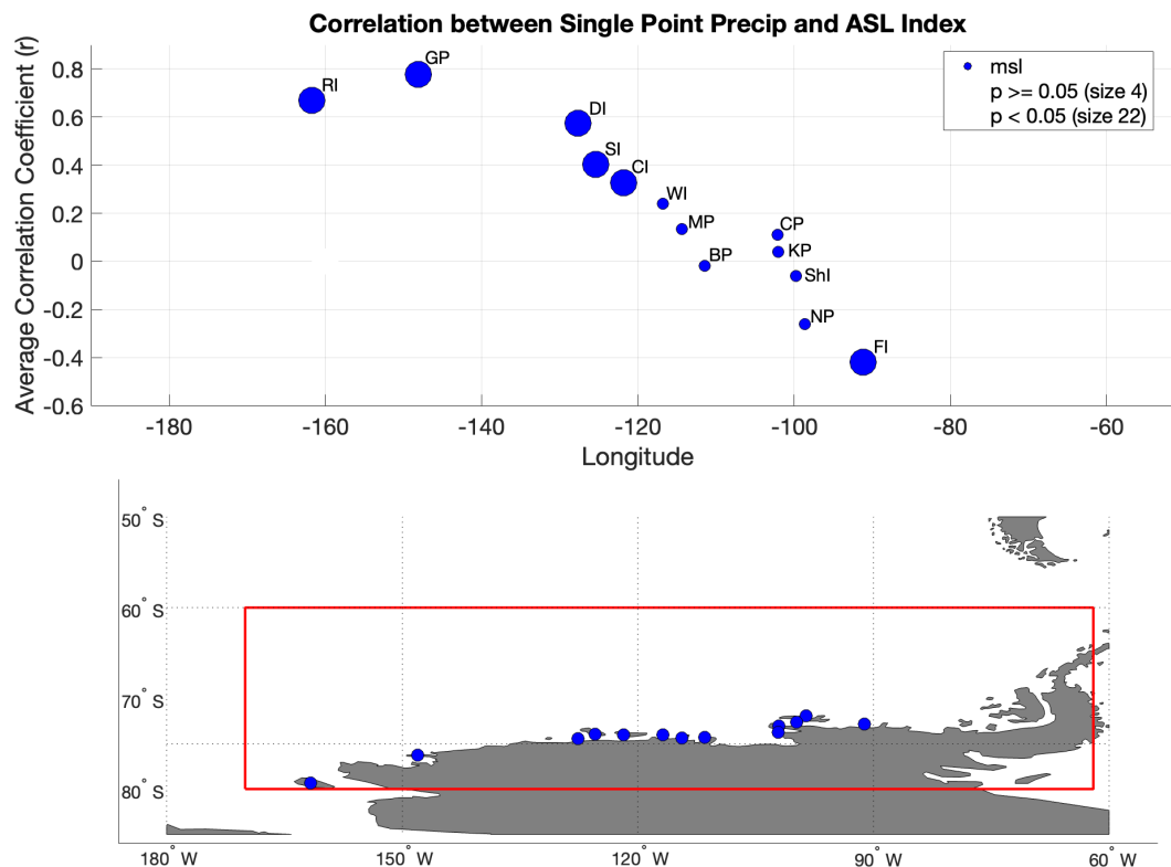
Figure 7. Correlation between precipitation at each ice rise and regional MSLP averaged over the Amundsen Sea Low index region (170 to 298° E, 80 to 60° S; Hosking et al., 2013). Marker size indicates statistical significance ( p < 0.05 for larger markers).
