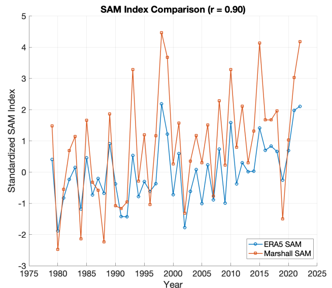
Figure A1. Comparison of standardized SAM index values, ERA5-derived SAM vs. Marshall (2003) calculated SAM.
