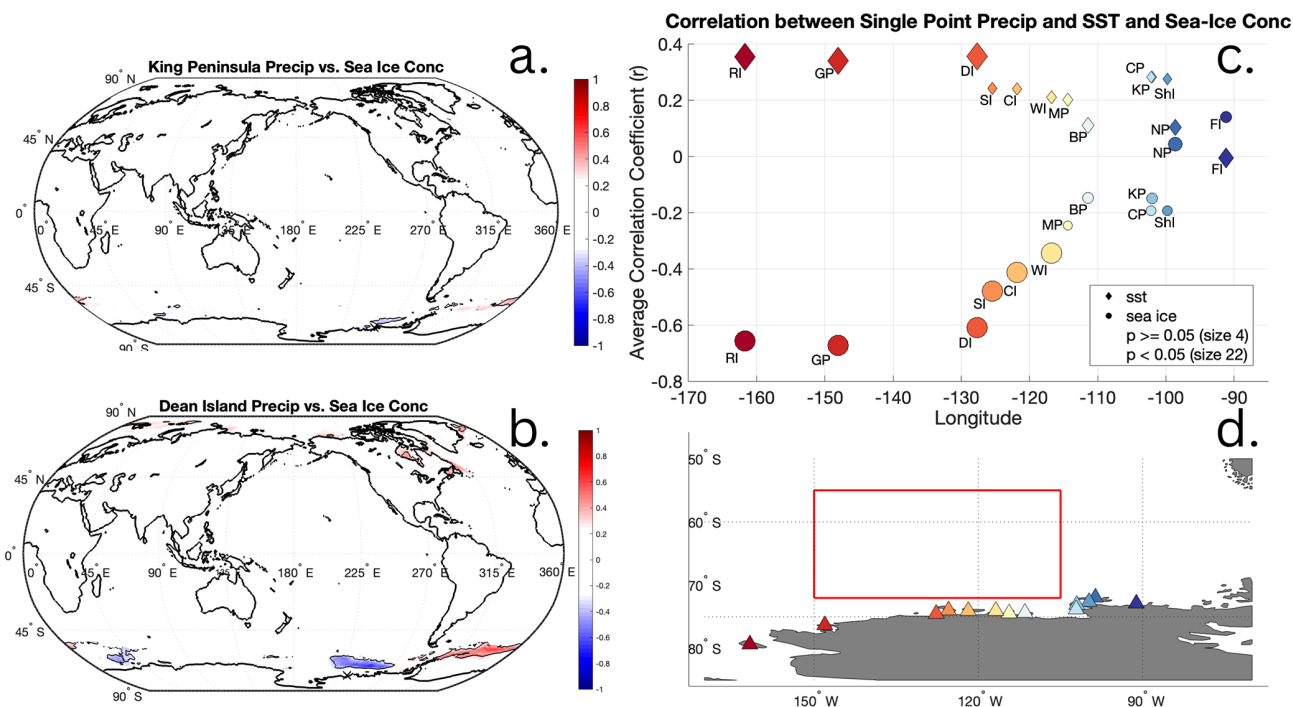
Figure 9. Sea surface temperature and sea ice concentration comparison. (a, b) Correlation between precipitation at each ice rise and global sea ice concentration at King Peninsula (a) and Dean Island (b). (c) Correlation between precipitation at each ice rise and sea surface temperature (SST, diamond) as well as sea ice concentration (SIC, circle) averaged over the Amundsen Sea box (d).
