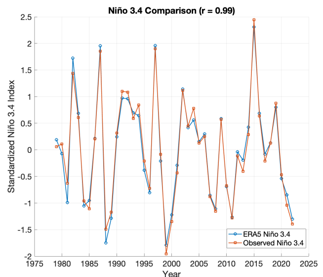
Figure A2. Comparison of standardized Niño 3.4 index values, ERA5-derived Niño 3.4 vs. Trenberth (2025) observed Niño 3.4.
