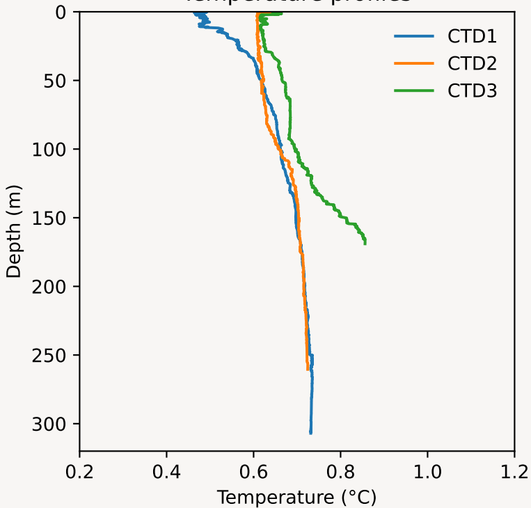
Temperature profiles
