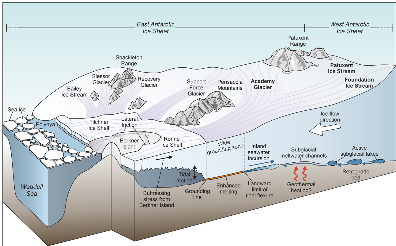
Figure 10. Visualisation of the Foundation Patuxent Academy System (FPAS), showing its pattern of ice flow, landscape setting, and subglacial and grounding zone processes. Also shown is the FPAS's relationship to surrounding outlet glaciers in the Weddell Sea sector, the Filchner-Ronne Ice Shelf (including the grounded Berkner Island), the Southern Ocean, and major mountain ranges. Note that the visualisation is not true to scale, with some features exaggerated relative to others for display purposes.
