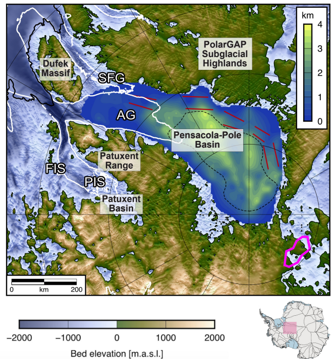
Figure 5. Geological structure of the FPAS catchment. Gravity anomaly modelling indicates that the Pensacola-Pole Basin (PPB) is underlain by a sedimentary basin 2–3 km thick in places (Paxman et al., 2019; see interior colour scale); the potential sedimentary infill within the Patuxent Basin was not analysed in Paxman et al. (2019). The southern part of the PPB (thin black dashed line) is characterised by the largest thicknesses of sedimentary fill and also exhibits topography and high-frequency magnetic anomalies characteristic of Jurassic dolerite sills, which are commonly intruded into Beacon Supergroup sediments (Paxman et al., 2019). Red lines mark a series of deep (1–2 km below sea level) troughs located along the eastern margin of the PPB. Magenta polygon demarcates a zone of basal melting attributed to elevated geothermal heat flux (Jordan et al., 2018). White line marks the 50 m yr -1 ice-surface velocity contour (Mouginot et al., 2019). Thick black dashed line is Bedmap3 grounding line (Pritchard et al., 2025). Bed topography is from BedMachine v4 (Morlighem, 2025). Outlet glaciers are: Foundation Ice Stream (FIS), Academy Glacier (AG), Patuxent Ice Streams (PIS), Support Force Glacier (SFG). Inset map shows extent of figure (pink rectangle).
