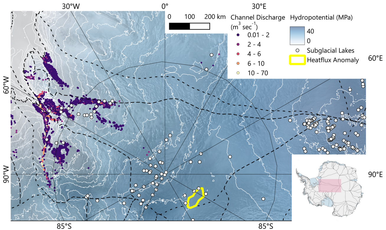
Figure 6. Subglacial hydrology of the FPAS catchment showing location of subglacial lakes (Livingstone et al., 2022), modelled subglacial channel discharge (Ehrenfeucht et al., 2025), and zone of basal melting attributed to elevated geothermal heat flux (Jordan et al., 2018), underlain by hydropotential surface derived from Bedmap3 (Pritchard et al., 2025) with contours (white lines) at 2 MPa intervals. Black lines are Ice Sheet Mass Balance Inter-comparison Exercise (IMBIE) catchments (Mouginot et al., 2017) and Bedmap3 grounding zone (Pritchard et al., 2025). Inset map shows extent of figure (pink rectangle).
