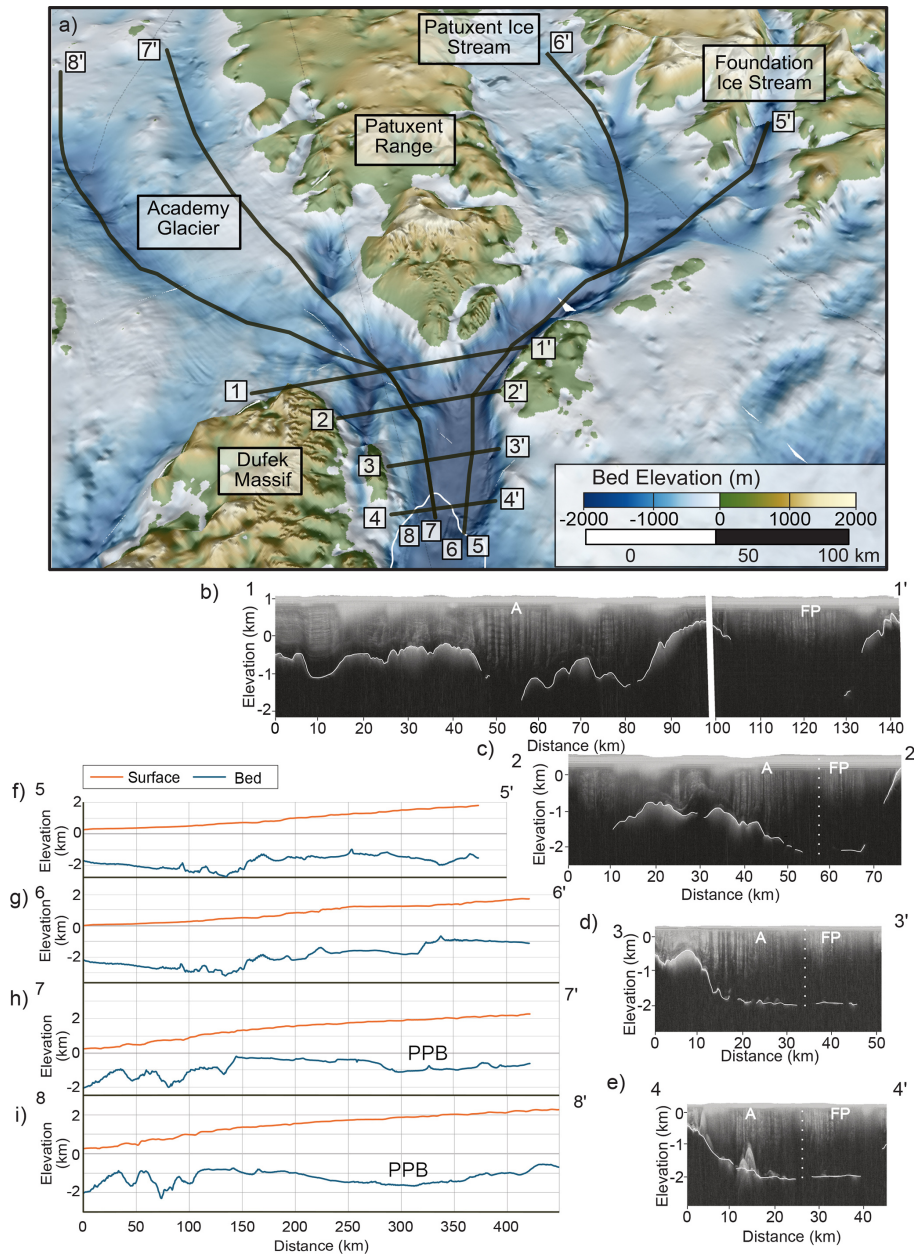
Figure 2. Perspective view of topography and geometry of lower trunk of FPAS, illustrating low ice surface elevation, and extent, size and depth (> 2 km below sea level) of the Foundation-Thiel trough beneath the FPAS trunk. (a) 3D bed topography (Bedmap3, Pritchard et al., 2025) with profile lines shown in subplots (b)–(i). Bedmap3 is used in this figure as this product emphasises the deep troughs beneath the FPAS. View is into the ice sheet from the grounding zone. Grounding line (Pritchard et al., 2025) is white line; Black lines are approximate locations of radar profiles shown in (b)–(e) and topographic profiles in (f)–(i); (b–e) radargrams, with ice thickness picks (white lines) overlain, from the Filchner Ice Shelf System (FISS) survey (profiles 1–4 on (a) – radar transect names: FISS2015_FOU1 (b), FISS2015_FOU2 (c), FISS2015_FOU4 (d), FISS2015_FOU6 (e)) (Nicholls et al., 2024). The bright “englacial” reflections ~ 12–16 km along 4–4’ represent ice shelf channels; (f–i) Glacier surface (orange) and bed (blue) profile elevations (Bedmap3) for Foundation Ice Stream (profile 5 on a), Patuxent Ice Stream (profile 6 on a) and Academy Glacier (profiles 7 & 8 on a). 0 m on x axes of (f)–(i) represents position of Bedmap3 grounding line. On (b)–(e): A: Academy Glacier, FP: Foundation-Patuxent (vertical dashed lines mark boundary between the two flow zones). On (h)–(i): PPB: Pensacola-Pole Basin.
