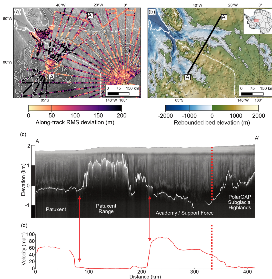
Figure 4. Roughness and ice-free bed topography beneath lower parts of FPAS. (a) Along-track root mean square deviation of bed elevation within a moving window of 2 km (a proxy for roughness) from PolarGAP, FISS, and Operation IceBridge RES profiles (Corr et al., 2021; Nicholls et al., 2021; CReSIS, 2025; MacGregor et al., 2021), showing relatively smooth (pale yellow) zones beneath parts of Academy Glacier and Patuxent Ice Stream; (b) Rebounded (“ice-free”) topography of lower FPAS derived from BedMachine v2 (Paxman et al., 2022). In (a) and (b) the grey contour lines represent the rebounded 0 m contour, the thick white line is the Bedmap3 grounding line (Pritchard et al., 2025) and the white dashed lines are the IMBIE mass balance basins (Mouginot et al., 2017). The smoothest bed topography beneath FPAS is located below the 0 m contour (grey line) for both Academy and Foundation-Patuxent tributaries. These “smooth” zones correspond to the model-derived low basal shear stress zones of Joughin et al. (2006), based on the BEDMAP DEM; (c) example radargram (radar transect name: POLARGAP_P13A), with ice thickness picks overlain, from the PolarGAP survey (profile A–A’ on b ) (Ferraccioli et al., 2021). Ice flow direction is into page; (d) ice velocity (Mouginot et al., 2019) along profile A–A’. Vertical dashed red line on (c) and (d) is the boundary between Academy and Support Force glaciers. Vertical red arrows on (c) and (d) denote the shear margins where Patuxent Ice Stream and Academy Glacier abut the Patuxent Range. These correspond to scattering zones in the overlying radargram. Inset map shows extent (pink rectangle) of (a) and (b) .
