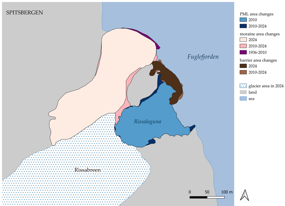
Figure A3. The map shows changes in the surface area of the Rissalaguna, barriers, and moraines over the years.
