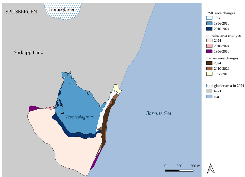
Figure A5. The map shows changes in the surface area of the Tromsølaguna, barriers, and moraines over the years.
