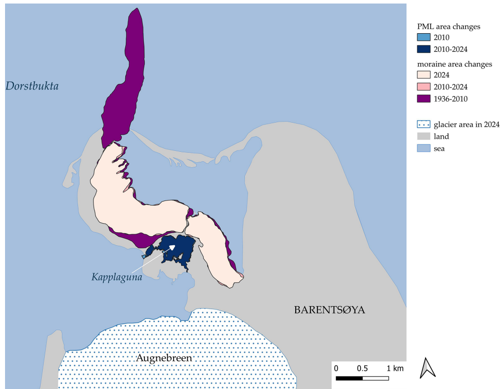
Figure A1. The map shows changes in the surface area of the Kapplaguna, barriers, and moraines over the years.
