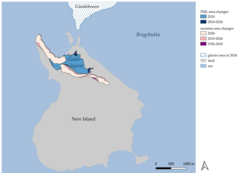
Figure A2. The map shows changes in the surface area of the Gimlelaguna, barriers, and moraines over the years.
