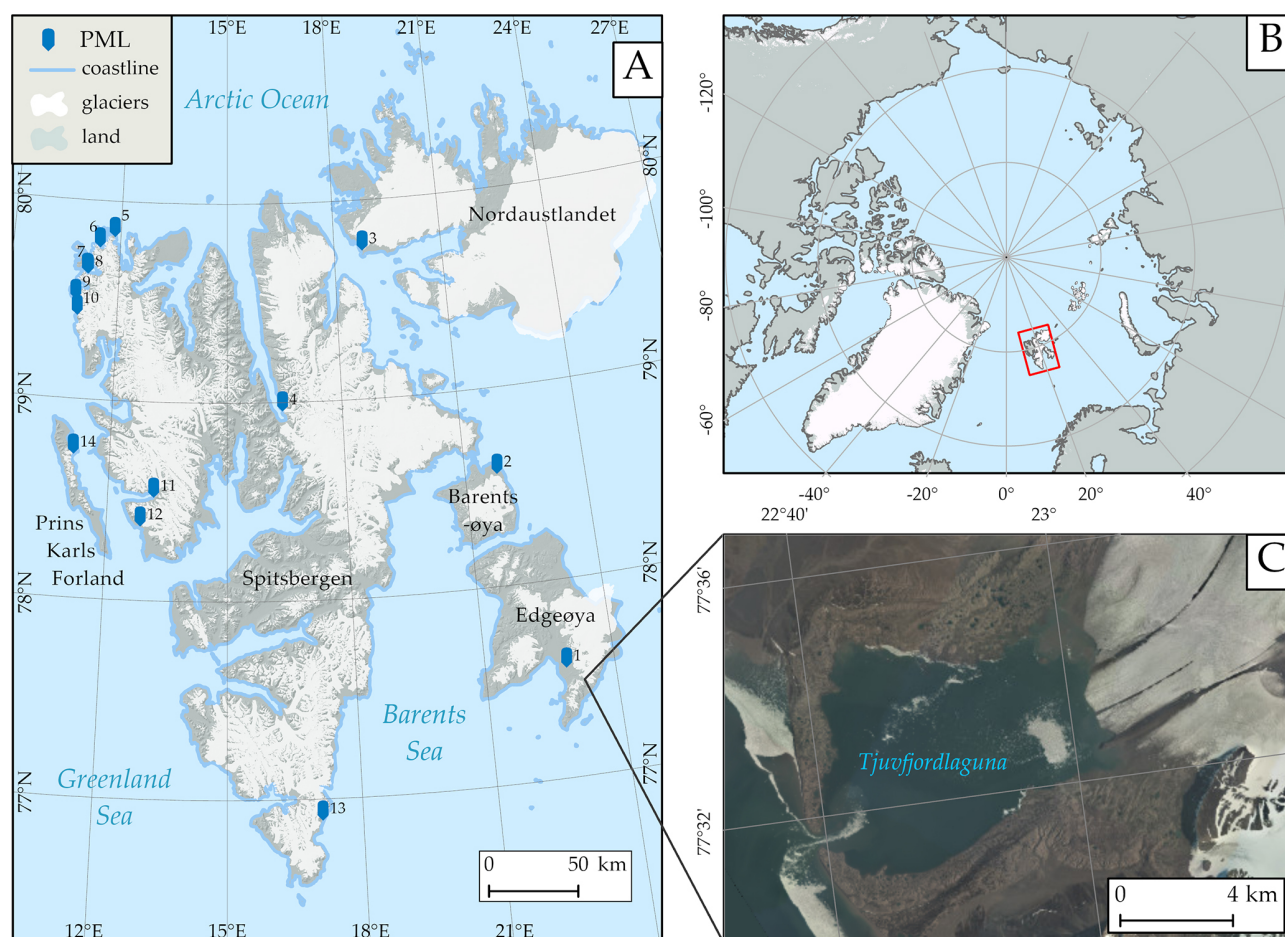
Figure 1. (A) PMLs' location on Svalbard. 1: Tjuvfjordlaguna, 2: Kapplaguna, 3: Gimlelaguna, 4: Snaddlaguna, 5: Makarovlaguna, 6: Rissalaguna, 7: Schielaguna, 8: Skodelaguna, 9: Sjulaguna, 10: Femtelaguna, 11: Charleslaguna, 12: Eidemlaguna, 13: Tromsølaguna, 14: Murraylaguna. (B) Svalbard (marked with a red rectangle) on an Arctic map. (C) The most representative paraglacial moraine lagoon in Svalbard – Tjuvfjordlaguna. Base map: 2010 orthophotomorph comes from the (Norwegian Polar Institute, 2026).
