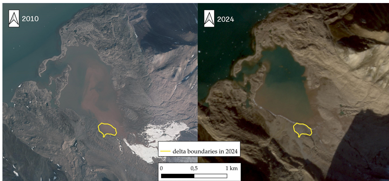
Figure 11. Development of a new delta (approximately 0.04 km 2 ) on the southern Charleslaguna shore. Base maps: the 2010 orthophotomap comes from (Norwegian Polar Institute, 2026), and the 2024 satellite imagery comes from (Planet Labs, 2025).
