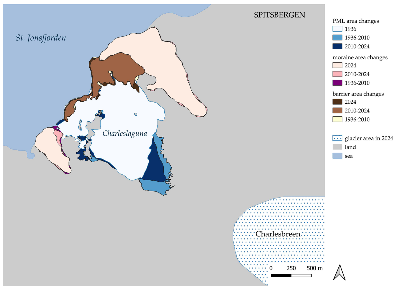
Figure 5. The map shows changes in the surface area of the Charleslaguna, barriers, and moraines over the years.
