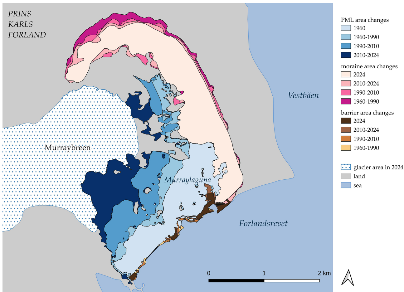
Figure 10. The map shows changes in the surface area of the Murraylaguna, barriers, and moraines over the years.
