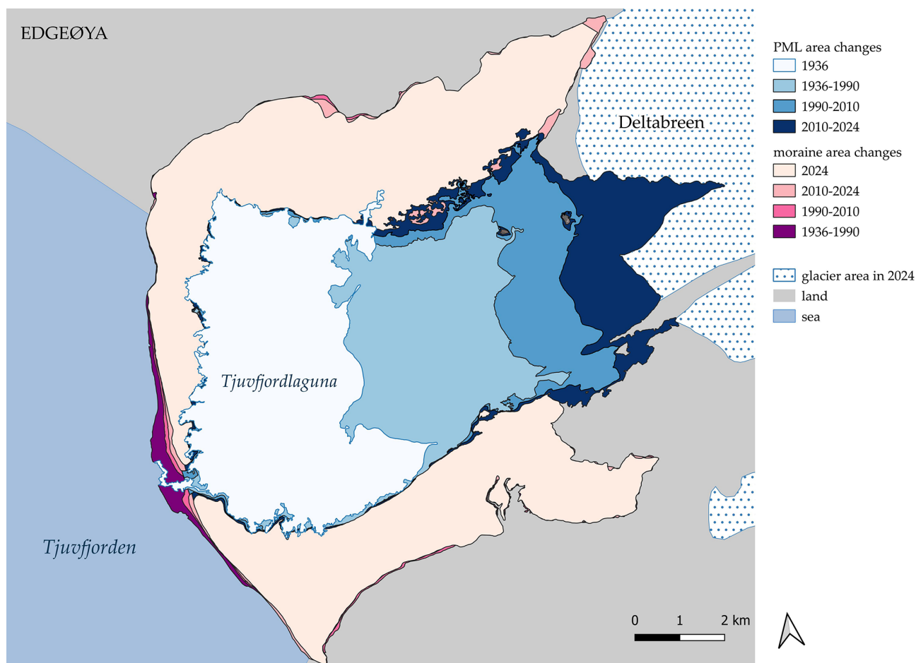
Figure 2. The map shows changes in the surface area of the Tjuvfjordlaguna and moraines over the years.
