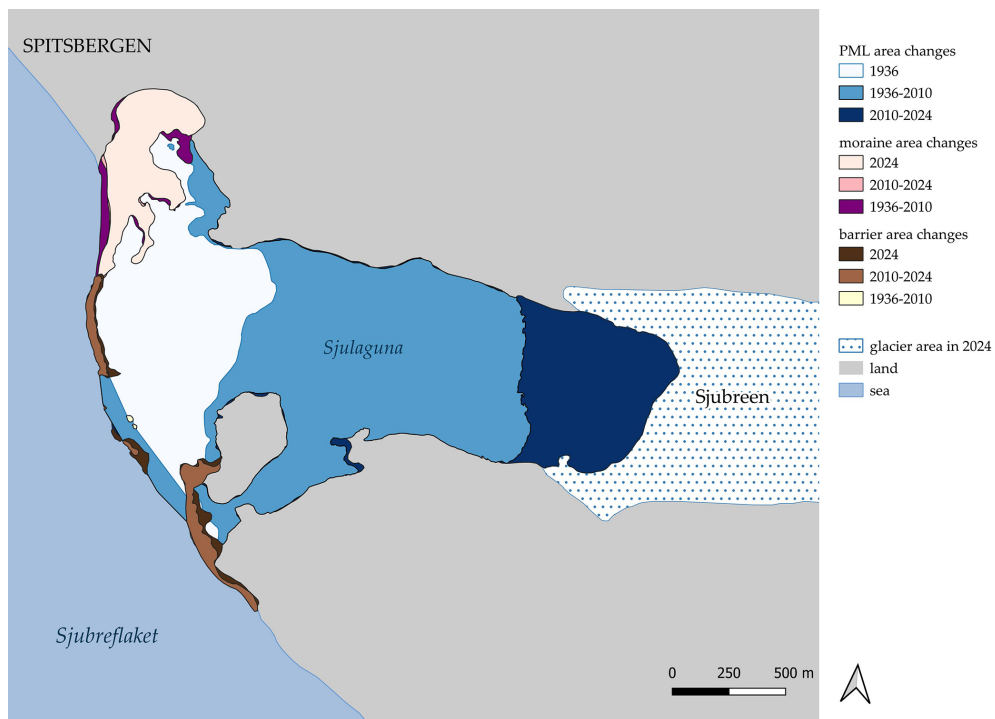
Figure A4. The map shows changes in the surface area of the Sjulaguna, barriers, and moraines over the years.
