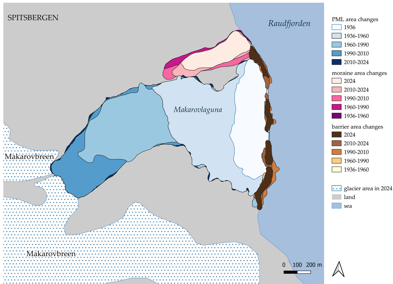
Figure 7. The map shows changes in the surface area of the Makarovlaguna, barriers, and moraines over the years.
