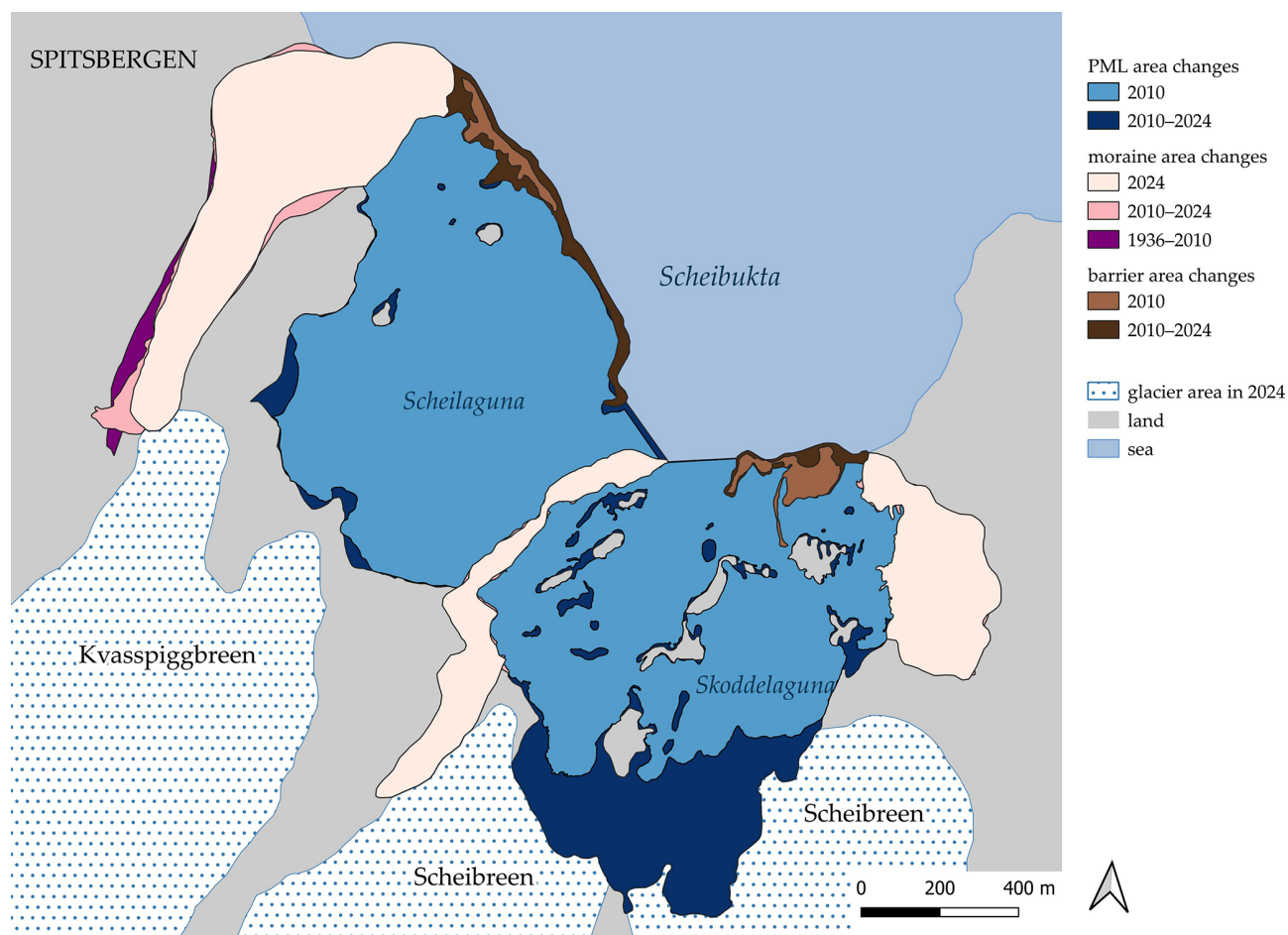
Figure 9. The map shows changes in the surface area of the two PLMs – Scheilaguna and Skoddelaguna – barriers and moraines over the years.
