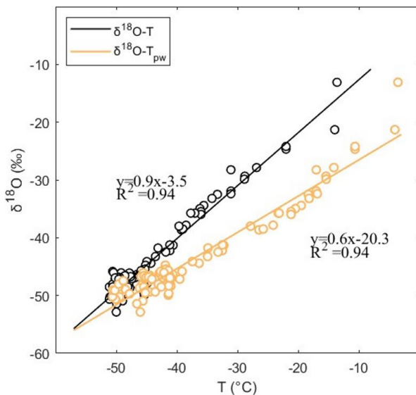
Figure 3. \delta^{18}\text{O}-T vs. \delta^{18}\text{O}-T_{\text{pw}} relationships evaluated for surface snow samples, calculating mean temperature and precipitation-weighted temperature over time intervals corresponding to 3 cm of snow precipitation.
