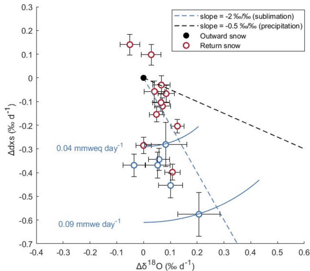
Figure 9. d-excess vs. \delta^{18}\text{O} evolution of snow per day for Section I (empty red dots) and II (empty blue dots) centered on outward composition (black dot), in comparison with modeled dx_s/\delta^{18}\text{O} sublimation slope (blue dashed line) and precipitation slope (black dashed line). The fluxes relative to sublimation are expressed in \text{mm w.e. d}^{-1} . The errorbars represent the uncertainty from spatial variability.
