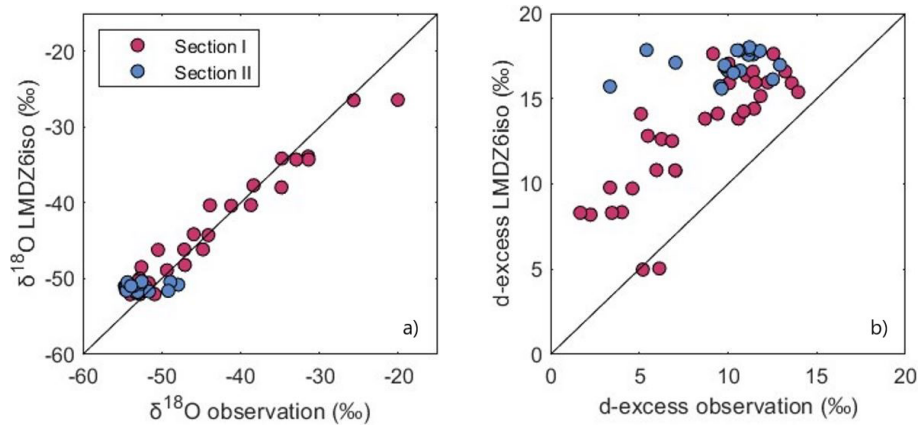
Figure 7. (a) \delta^{18}\text{O} and (b) d-excess LMDZ6iso values vs. bulk observations. The black line is for linear regression.
