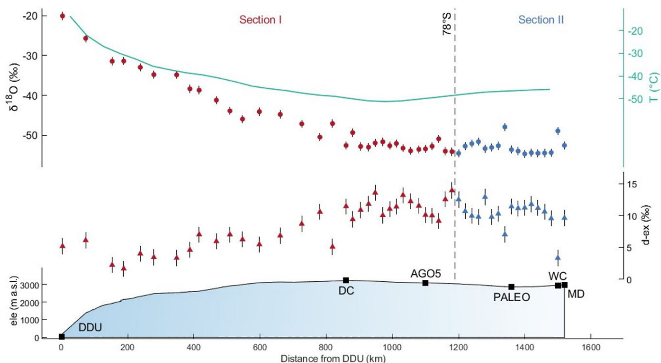
Figure 5. Spatial distribution of \delta^{18}\text{O} and d-excess values of bulk samples for Section I (red dots – north of 78^\circ\text{S} ) and Section II (blue dots – south of 78^\circ\text{S} ). The vertical bars represent the uncertainty associated with local variability. Temperature, elevation and distance from DDU are reported.
