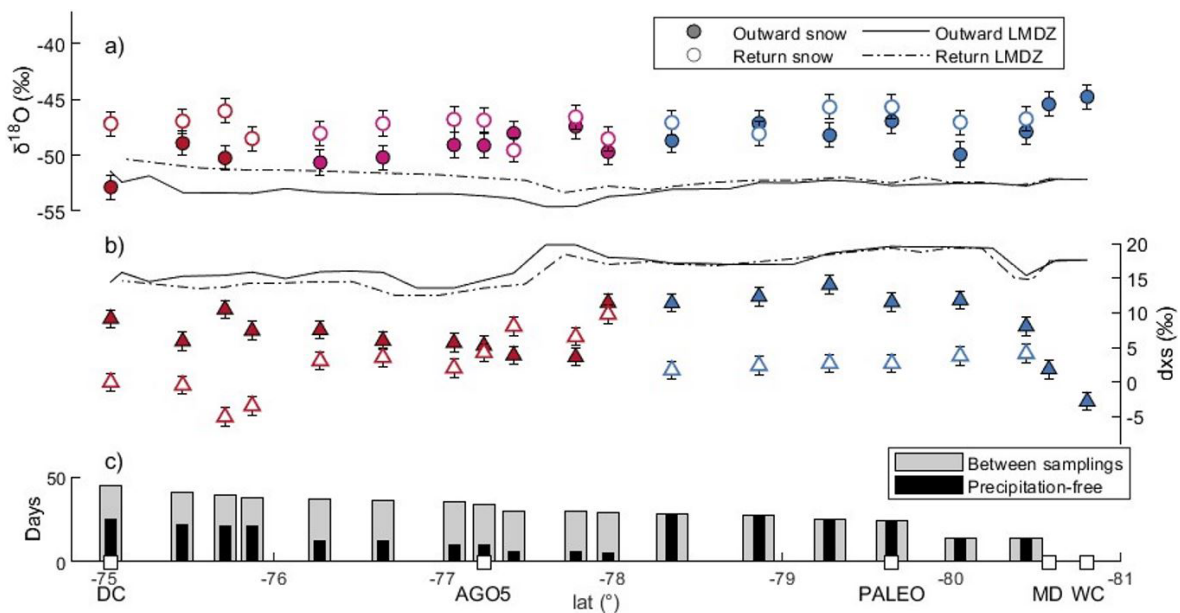
Figure 8. (a) \delta^{18}\text{O} and (b) d-excess composition of outward and return surface snow samples (dots) in comparison to the LMDZ6iso model outputs (lines). Vertical bars indicate spatial variability. (c) The days between the two journeys (grey) and the precipitation-free days prior the return sampling (black).
