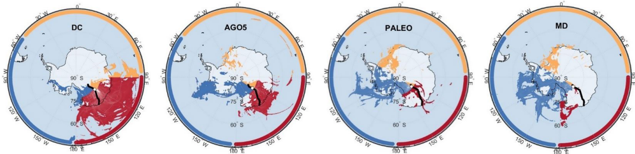
Figure 2. Precipitation-weighted air mass back-trajectory distributions for the period 2009–2019 at four key sites: DC, AGO5, PALEO, and MD. Colors indicate air mass origins: Indian (red), Pacific (blue) and Atlantic (orange) oceans.
