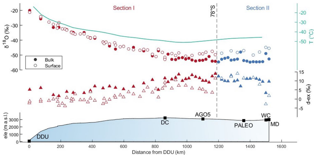
Figure B1. Spatial distribution of \delta^{18}\text{O} and d-excess values of surface (empty markers) and bulk (filled markers) samples for Section I (red – north of 78^\circ\text{S} ) and Section II (blue – south of 78^\circ\text{S} ). Temperature, elevation and distance from DDU are reported.
