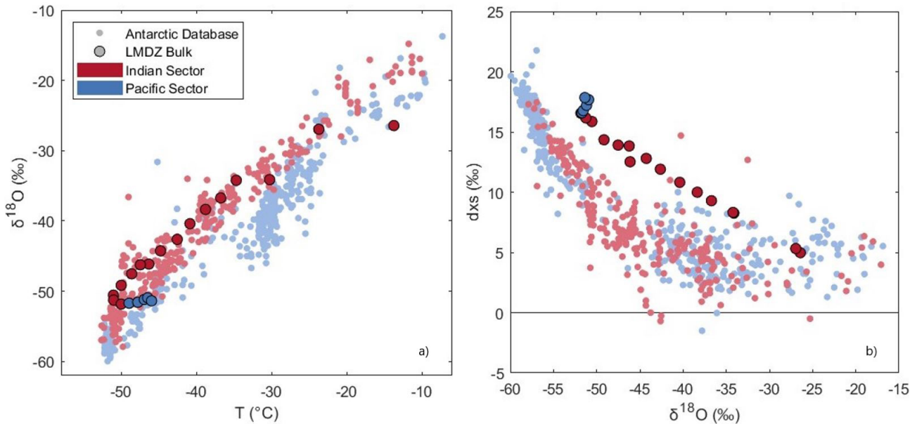
Figure C1. (a) \delta^{18}\text{O} - T relationship and (b) d-excess vs. \delta^{18}\text{O} for LMDZ6iso bulk samples of the traverse compared to observations from Antarctic database, separated into Pacific and Indian sectors.
