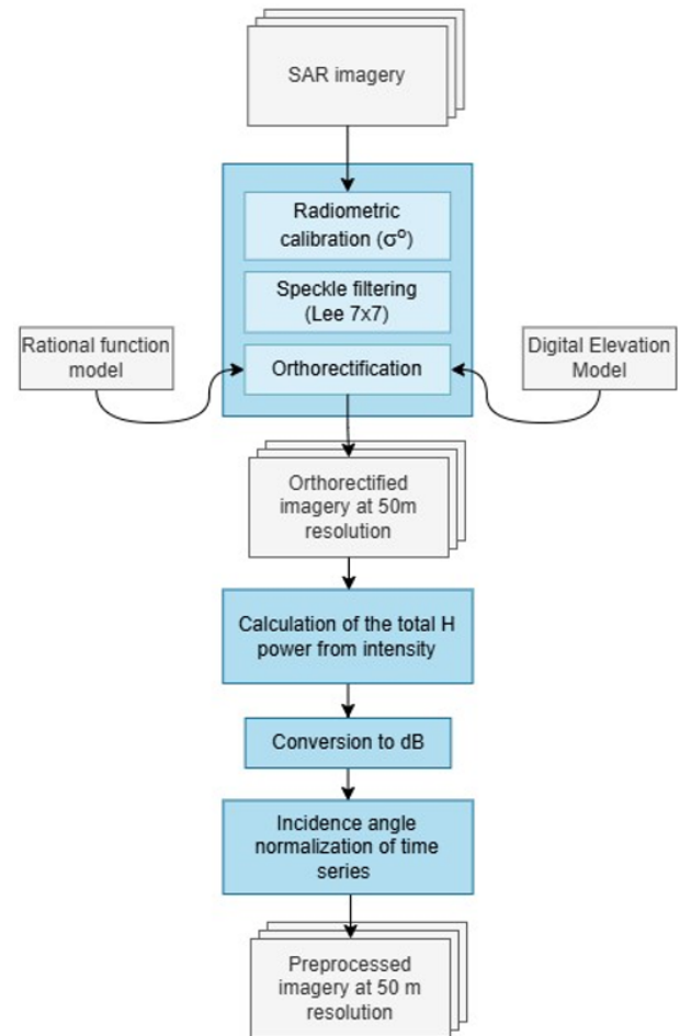
Figure 3. Flowchart of the SAR imagery (i.e., Sentinel-1 and RADARSAT-2) preprocessing.
