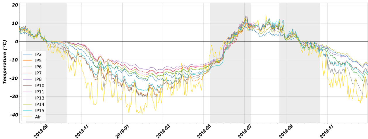
Figure 2. T_{soil} for the 10 reference sites (IP) and T_{air} from ECCC for the study period of August 2018 to December 2019 with the transition seasons (in grey) for freezing in 2018 and 2019 and thawing in 2019.
