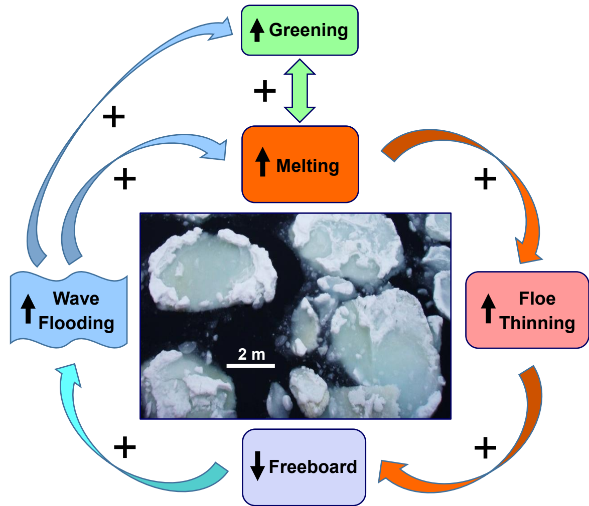
a) Wave flooding–ice thinning feedback
