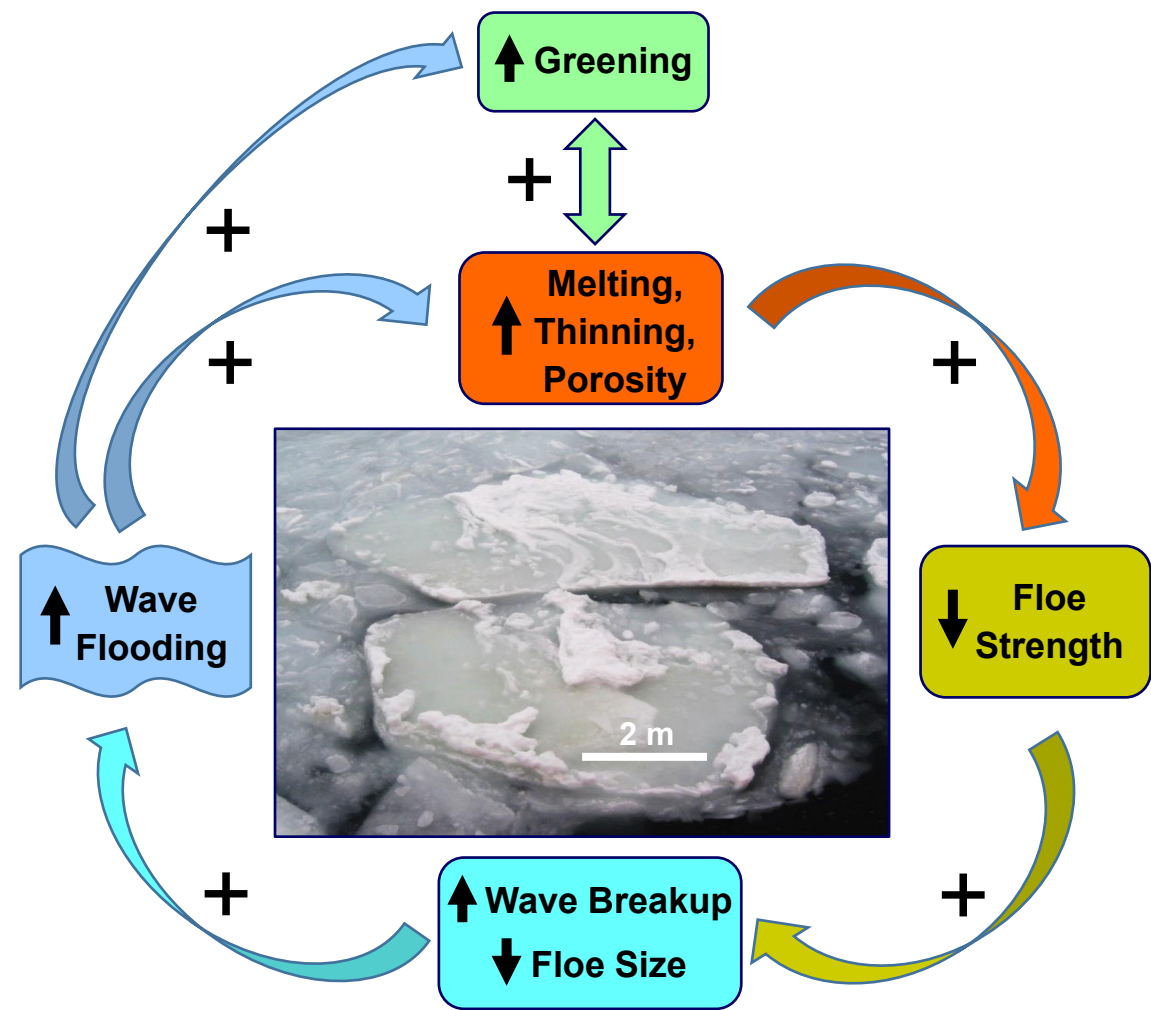
b) Wave flooding–floe fragmentation feedback
