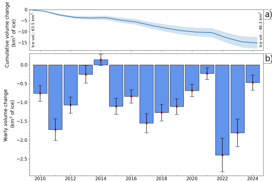
Figure 6. Swiss-wide ice volume change over 2010–2024. (a) The cumulative ice volume change (blue line) over the study period is shown with the respective uncertainty (shaded area). (b) Yearly volume changes (blue bars) with respective uncertainty ranges are shown.
