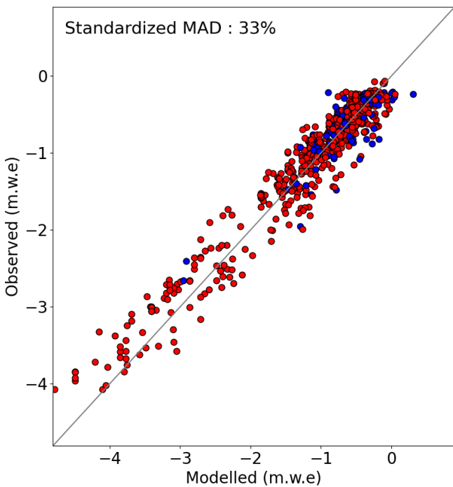
Figure 5. Evaluation of cumulated modelled daily mass balance against point mass balance measurements for periods spanning 7–90 d. Blue dots correspond to locations above the median glacier elevation, and red ones below it.
