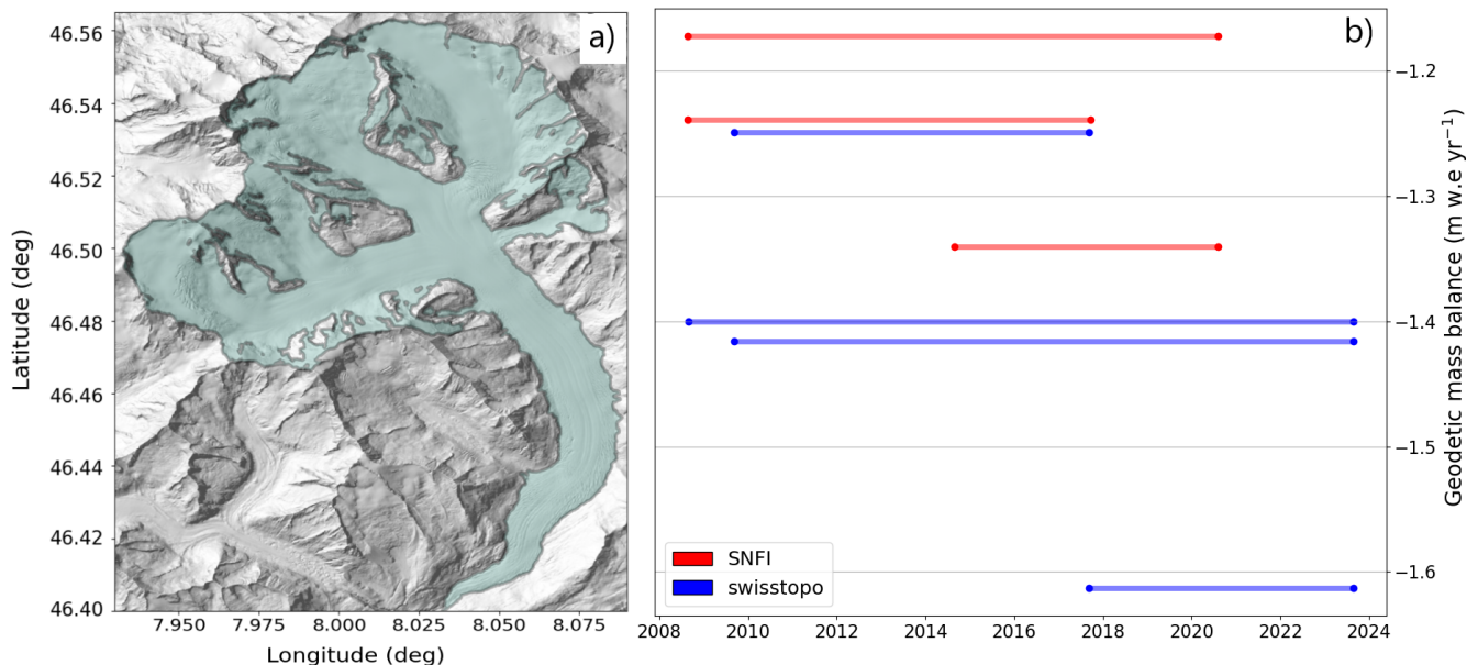
Figure 2. Temporal coverage of the geodetic ice volume changes available for Grosser Aletschgletscher. (a) Overview of Grosser Aletschgletscher with glacier outline from the SGI2016. (b) Geodetic mass balance based on the SNFI DEMs (red) and swisstopo DEMs (blue).
