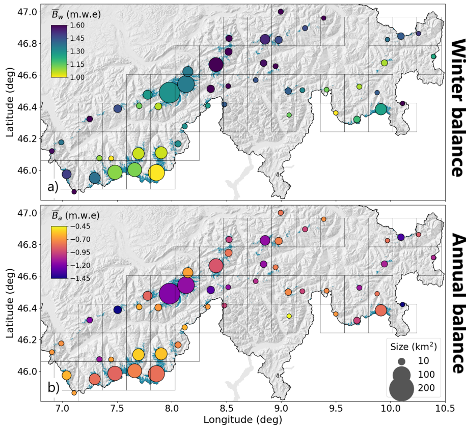
Figure 7. Average seasonal mass balance for the Swiss Alps over 2010–2024. (a) Average winter balance (30 April), and (b) average annual balance (30 September). Glacier-wide values are aggregated over a 20 km × 20 km grid with area-weighted averaging, whereby the size of the circles shows the glacierized area within each grid cell.
