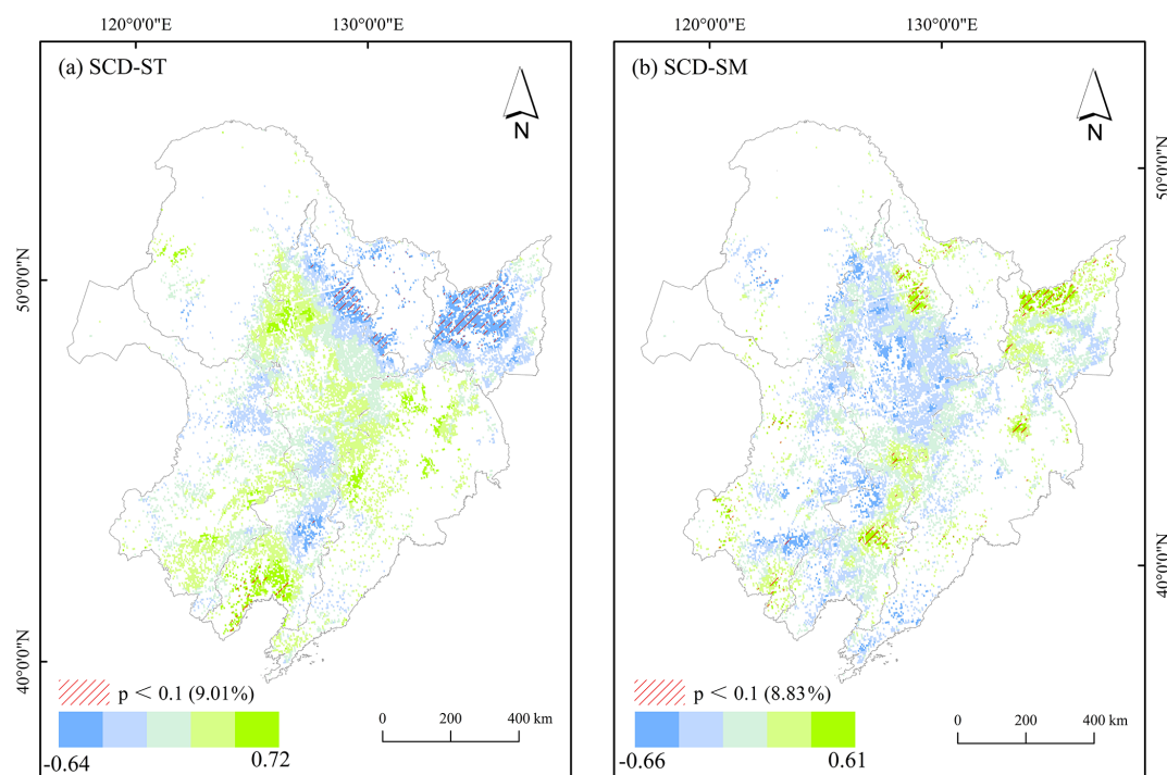
Figure 6. The correlation coefficients between SCD and soil properties: (a) soil temperature; (b) soil moisture. Blue and green pixels represent negative and positive correlations, respectively. The shaded regions denote pixels that were significant at the 90 % confidence level.
