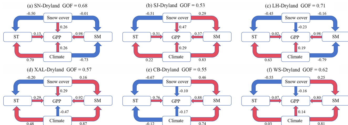
Figure 11. The standardized path coefficients between snow cover and GPP via soil properties. The model was validated through goodness-of-fit (GOF), demonstrating acceptable parameter estimation accuracy. Blue arrows denote inhibitory effects, whereas red pathways indicate facilitative relationships. Arrowhead orientation specifies causal pathways from exogenous to endogenous variables. ST and SM stand for soil temperature and soil moisture. SN, SJ, LH, XAL, CB and WS stands for Songnen Plain, Sanjiang Plain, Liaohe Plain, Xing'an Mountains, Changbai Mountains and West Sand Area.
