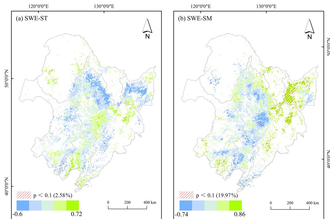
Figure 5. The correlation coefficients between SWE and soil properties: (a) soil temperature; (b) soil moisture. Blue and green pixels represent negative and positive correlations respectively. The shaded regions denote pixels that were significant at the 90 % confidence level.
