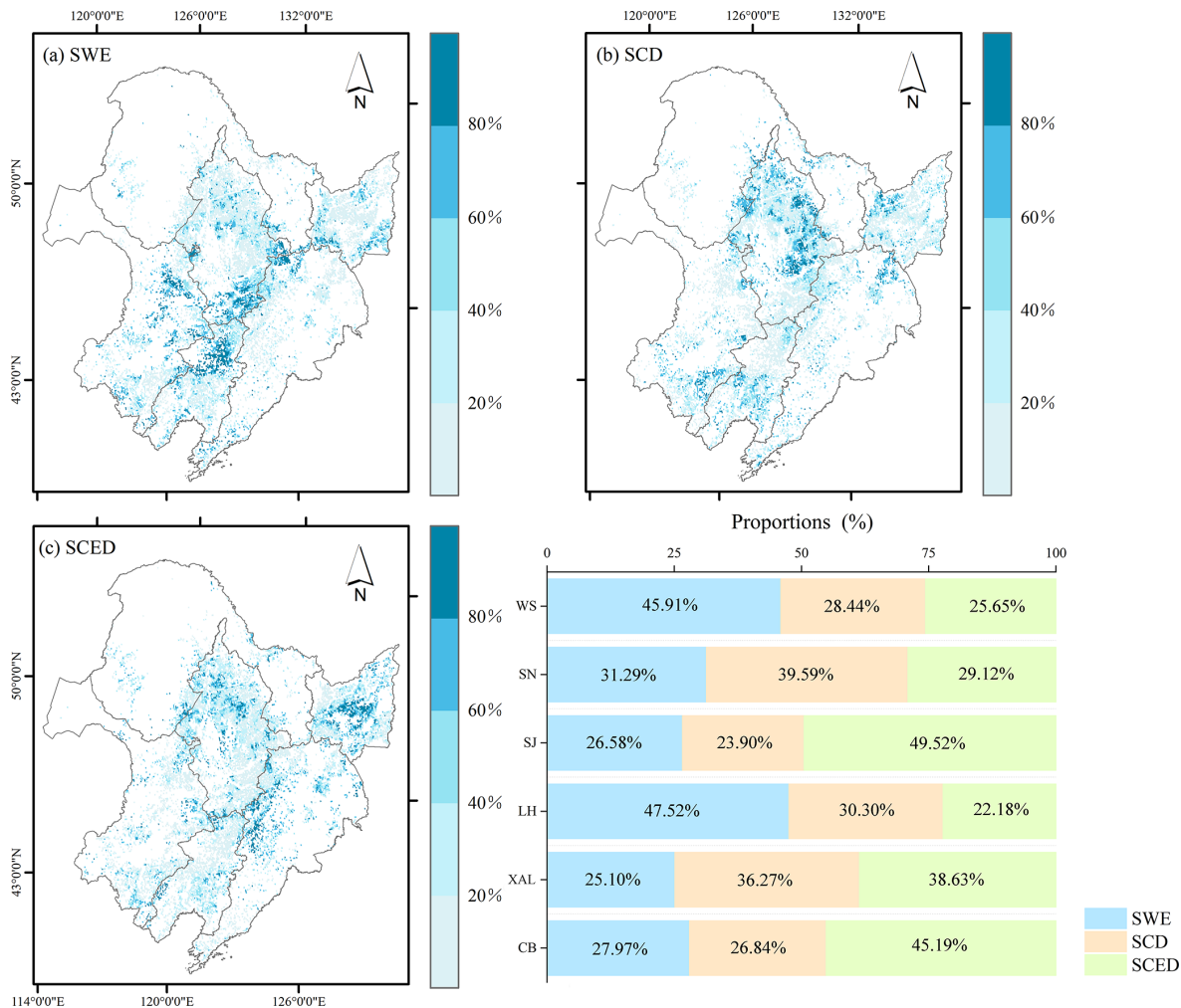
Figure 10. Spatial distribution and area percentage of snow-related indicators driving GPP variation of cultivated land in different regions of Northeast China from HY2001 to HY2020.
