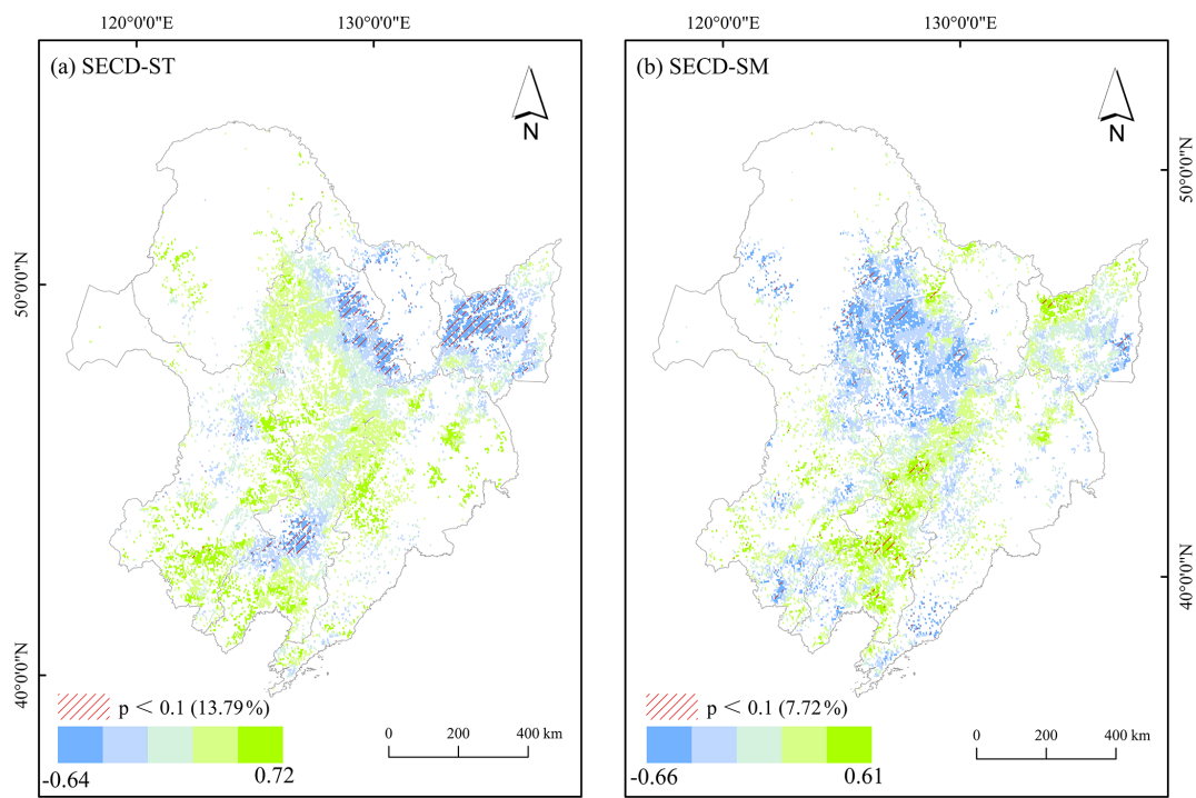
Figure 7. Spatial pattern distribution results of the relationship between SCED and soil properties: (a) soil temperature; (b) soil moisture. Blue and green pixels represent negative and positive correlations, respectively. The shaded regions denote pixels that were significant at the 90 % confidence level.
