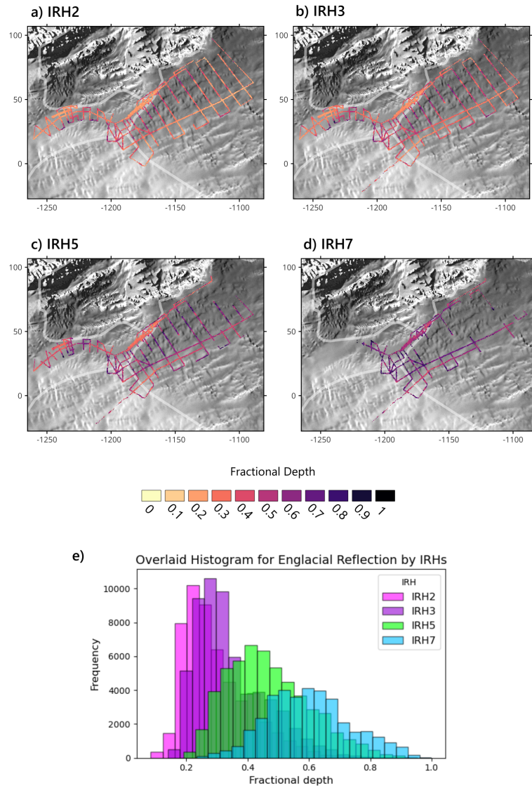
Figure B2. Spatial distribution and fractional depth histograms of internal reflection horizons (IRHs). Panels (a)–(d) show mapped IRHs across the Ellsworth Subglacial Highlands, overlaid on Radarsat Antarctic Mapping Project (RAMP) topography. Thin white lines delineate the ice catchment boundaries (Mouginot et al., 2017). Colours denote fractional depth within the ice column, ranging from 0 (surface; yellow) to 1 (bed; black). (a) IRH2, (b) IRH3, (c) IRH5, and (d) IRH7. Panel (e) presents overlaid histograms of fractional depths for each IRH. The shallower horizons (IRH2, IRH3) cluster at fractional depths of 0.15–0.35, whereas deeper horizons (IRH5, IRH7) extend more evenly through the ice column, with IRH7 reaching depths approaching the bed.
