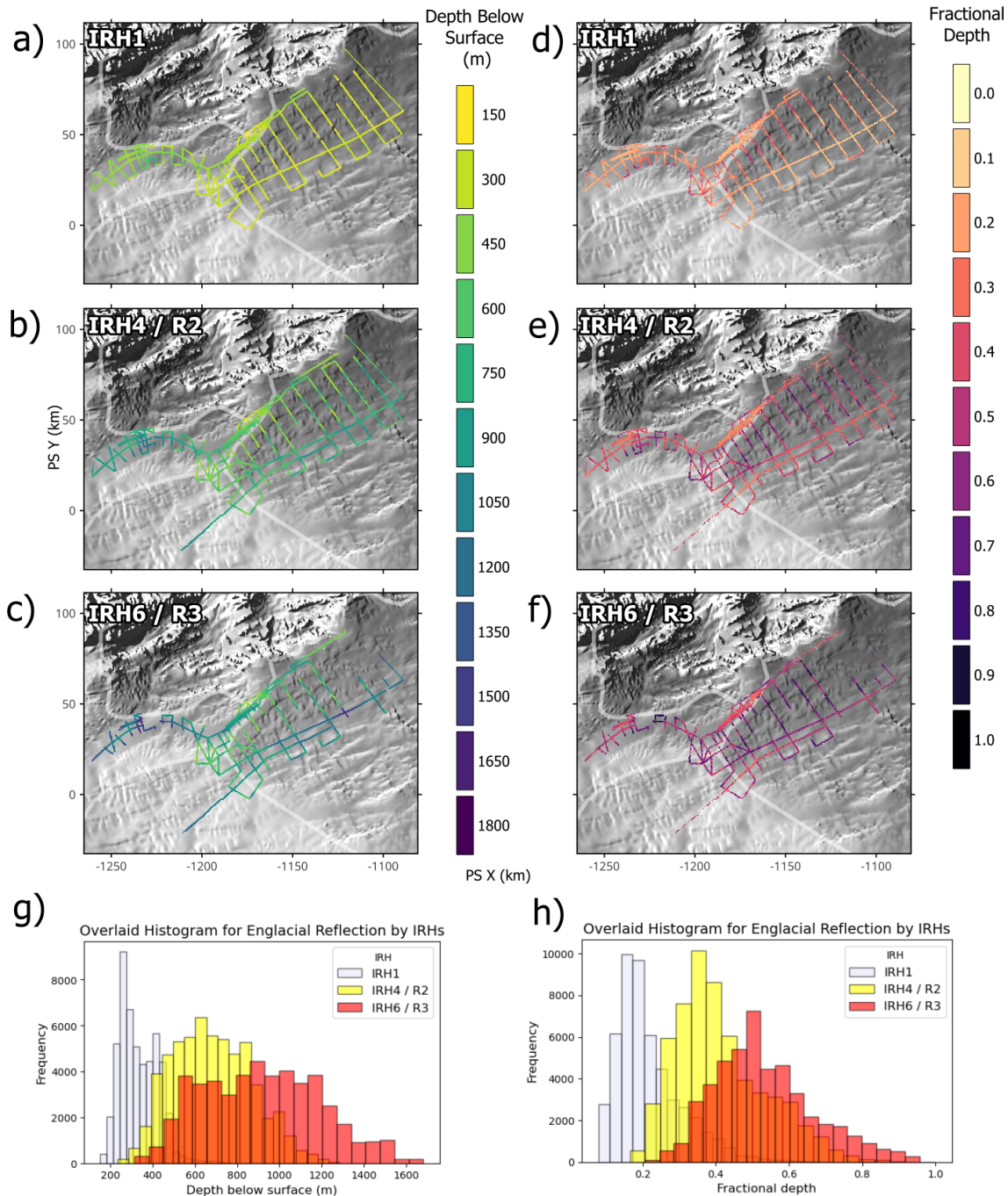
Figure 4. Internal Reflection Horizon (IRH) Depth Locations. Panels (a)–(c) display the absolute depth (in m) below the ice surface for three key englaciated layers: the shallowest layer detected in this study (IRH1), and two additional layers, IRH4 and IR6, which are synchronised with ice-core chronology (corresponding to R2 and R3 in Bodart et al., 2021). Panels (d)–(f) illustrate the fractional depth of each layer (i.e., the ratio of its depth to the total ice thickness), where warmer colours indicate shallower positions and colder colours indicate deeper positions within the ice column. Panels (g)–(h) present the distribution of both the absolute depth below the surface and the fractional depth for these layers. In all panels, the Radarsat Antarctic Mapping Project (RAMP) topography is shown in the background, with thin white lines delineating the ice catchment boundaries (Mouginot et al., 2017). A comprehensive analysis of all englaciated layers identified in this study is available in Appendix B: Figs. B1 and B2.
