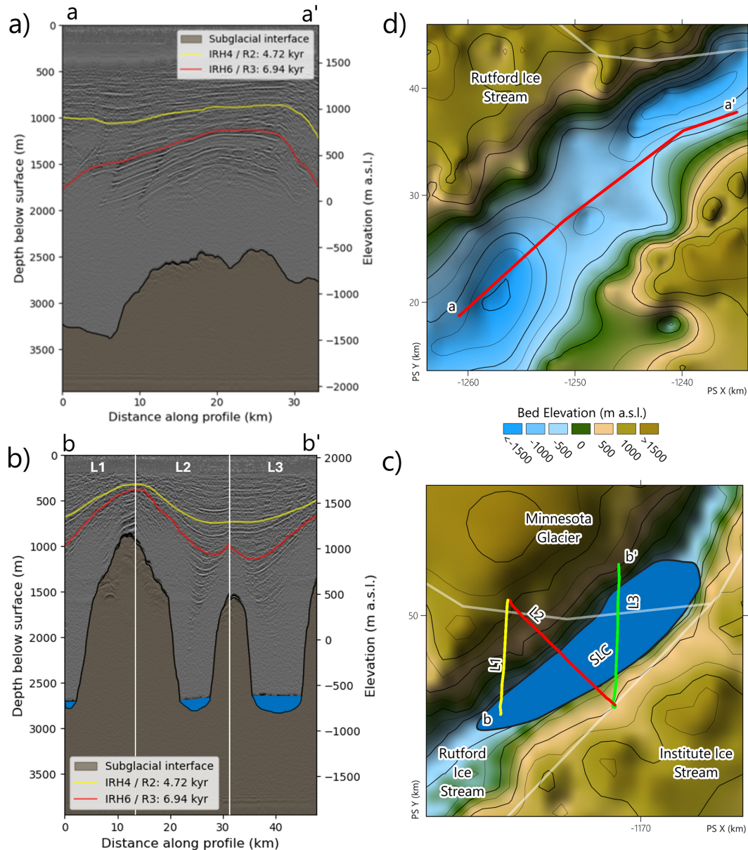
Figure 6. Internal Reflection Horizon (IRH) Continuity along CECs Trough and above Subglacial Lake CECs. Location of panel (a) in Fig. 3b (Area 1), and panel (b) in Fig. 3a (white star). (a) Example of steeply-dipping englacial reflections towards the end of the CECs Trough within the Rutford Ice Stream. The geometry of the IRHs could be indicative of basal melting above SLC. (b) Location of the RES profile shown in panel (a), also indicated in Fig. 1d. (c) Englacial geometry over Subglacial Lake CECs, displaying an evident drawdown of the englacial layers over SLC, and several continuous IRH below IRH6. The bathymetry of Subglacial Lake CECs is independently constrained from reflection seismic data (Brisbourne et al., 2023), providing a robust estimate of lake depth and sediment thickness beneath the ice. (d) RES survey geometry and acquisition setup for profiles shown in panels (c).
