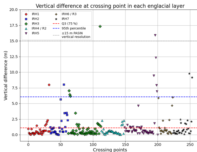
Figure B4. Vertical difference between crossovers of CECs Internal Reflection Horizon (IRH). Differences among IRH depth are presented for each IRHs in different colour and shape from the shallowest (IRH1) to the deepest one (IRH7). Additionally, we also marked the vertical resolution calculated for PASIN1 (Bodart et al., 2021) and key statistical percentiles.
