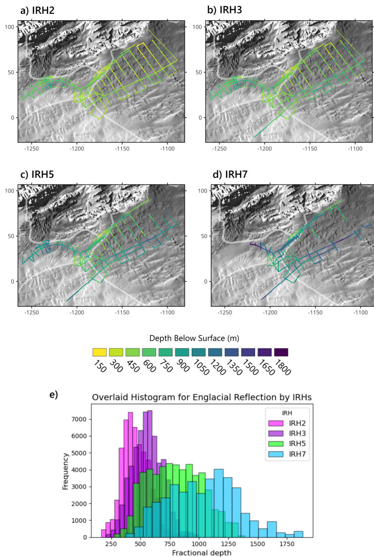
Figure B1. Spatial distribution and depth histograms of internal reflection horizons (IRHs). Panels (a)–(d) show mapped IRHs across the Ellsworth Subglacial Highlands, overlaid on Radarsat Antarctic Mapping Project (RAMP) topography. Thin white lines delineate the ice catchment boundaries (Mouginot et al., 2017). Each colour corresponds to depth below the ice surface, ranging from 150 m (yellow) to 1800 m (dark purple). (a) IRH2, (b) IRH3, (c) IRH5, and (d) IRH7. Panel (e) displays overlaid histograms of fractional depths for each IRH, illustrating their relative depth distributions. Shallower horizons (IRH2, IRH3) are concentrated between 250–700 m, while deeper horizons (IRH5, IRH7) extend to > 1500 m.
