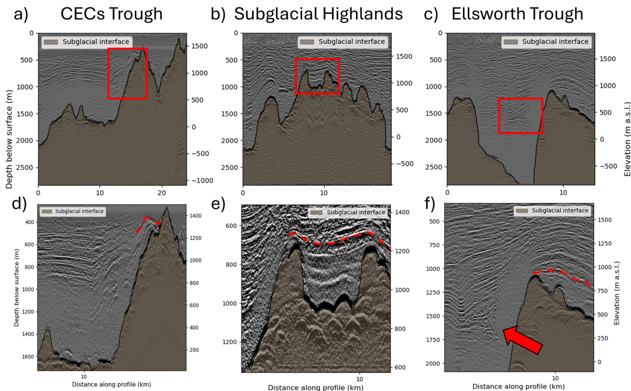
Figure 7. Examples of differences on internal reflectivity near the base of the ice in the Ellsworth Subglacial Highlands (locations of RES lines in Fig. 1d). (a) Southern end of the CECs Trough, and the boundary between englacial reflections near the mountain side (red dashed line in panel d ). (b) Ellsworth Subglacial Highlands, and the boundary between englacial reflections over the interflue and subglacial valley (red dashed line in panel e ). (c) Ellsworth Trough, and the boundary between englacial reflections over the interflue and subglacial valley (red dashed line in panel f ). The red arrow in panel (f) indicate the changes in dipping angle of the englacial layer.
