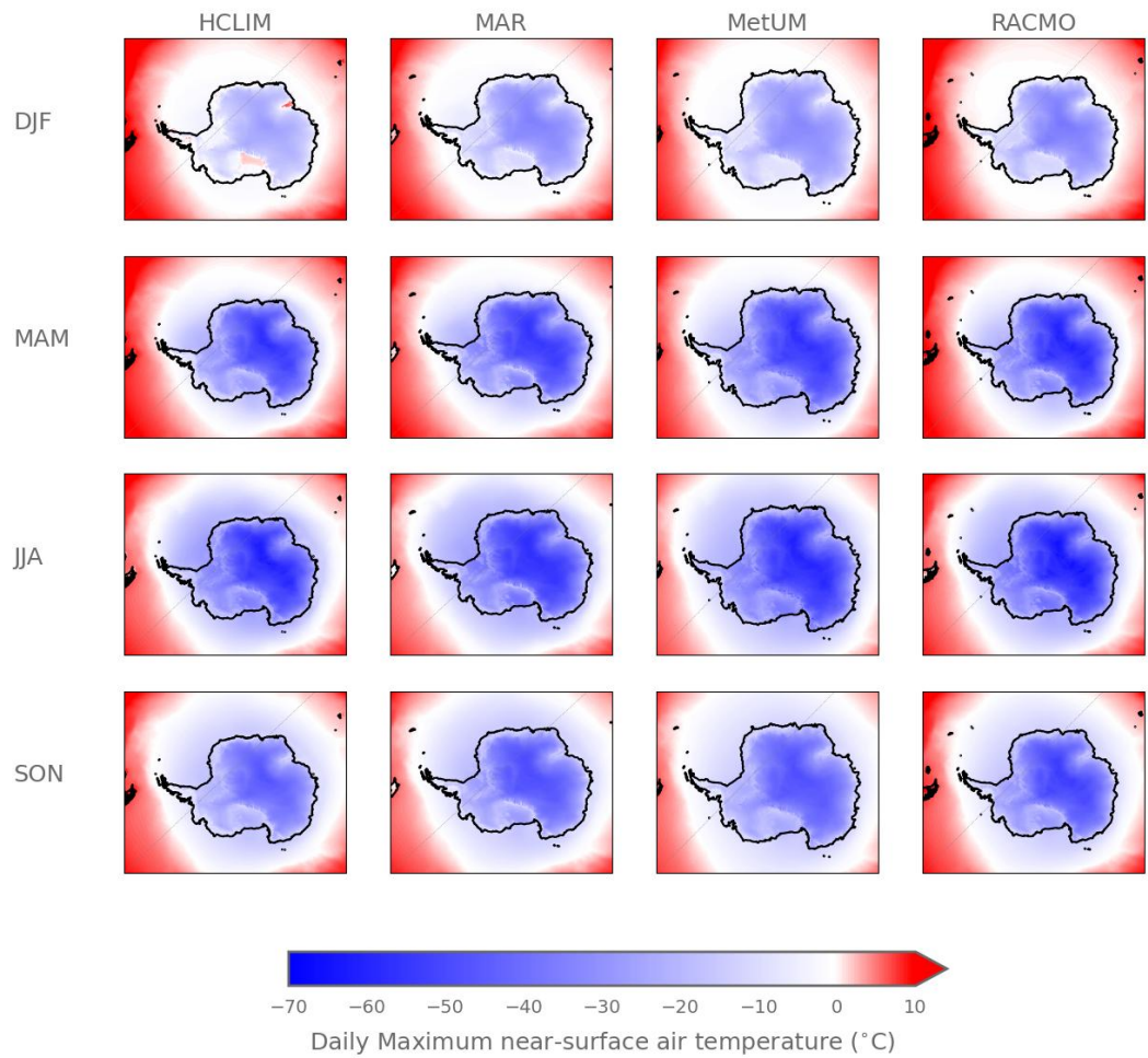
Figure S1: Seasonal mean daily maximum near-surface air temperature, in °C, during the period 2000-2019 for each of the four RCMs: HCLIM, MAR, MetUM and RACMO.
