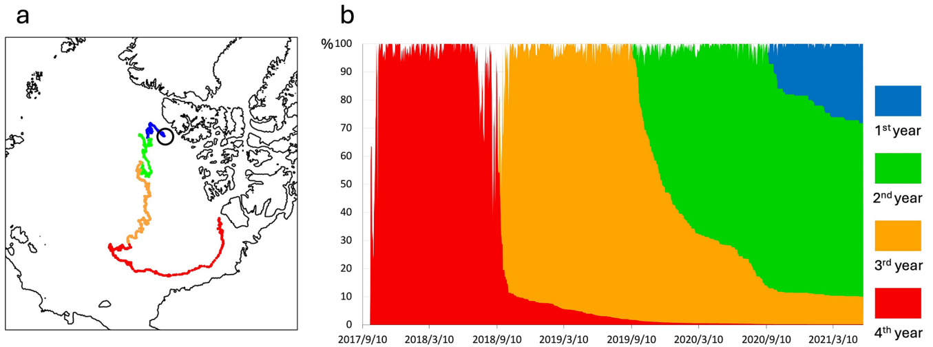
Figure 3. (a) Backward trajectories of a synthetic sea ice particle initialized on 31 May 2021 (white circle). The colored lines represent the particle's drift path in different time periods: blue for 10 September 2020–31 May 2021, green for 10 September 2019–10 September 2020, orange for 10 September 2018–10 September 2019, and red for before 10 September 2018. The earliest traced date corresponds to 1 October 2017, which is considered the formation date of the sea ice. (b) Time series of the ice concentration along the particle's trajectory from 10 September 2017 to 31 May 2021. The vertical axis represents ice concentration (%). The stacked colored areas show the fractional contributions of ice formed in each period: red for ice formed before 10 September 2018, orange for 10 September 2018–10 September 2019, green for 10 September 2019–10 September 2020, and blue for after 10 September 2020. Initially, the ice concentration quickly increases to nearly 100 % and remains high throughout the lifetime.
