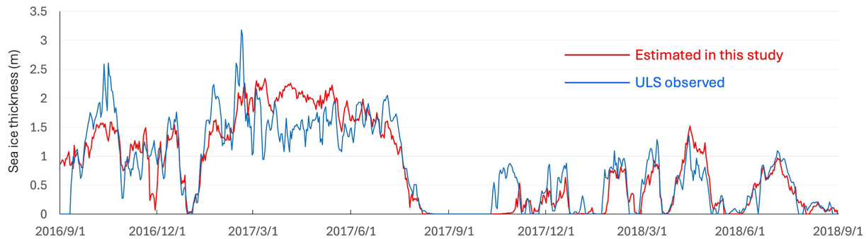
Figure 8. Comparison of sea ice thickness estimated in this study (red line) with observed ice thickness (blue line) by ULS at the Fram Strait mooring site (labeled F in Fig. 1a) from 1 September 2016 to 1 September 2018. The observed values represent the effective ice thickness presented in Sumata et al. (2022).
