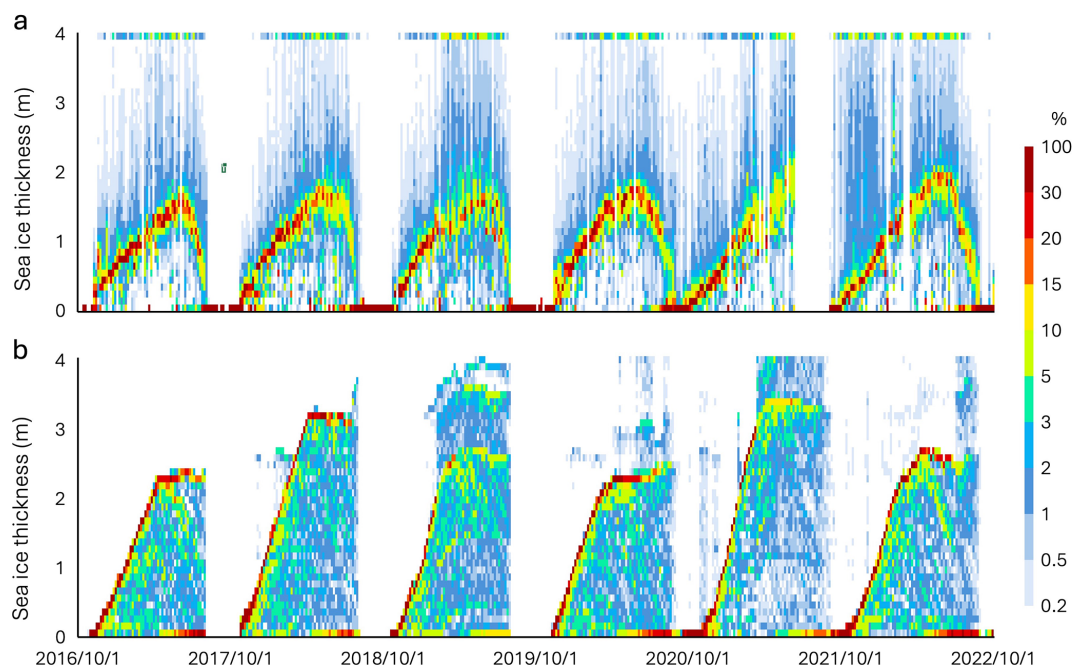
Figure 14. (a) Seasonal evolution of sea ice thickness distribution at mooring site A (location shown in Fig. 1a), shown for (a) ULS observations and (b) our estimates. The horizontal axis spans 1 October 2016 to 1 October 2022 at five-day resolution. The vertical axis shows ice thickness from 0 to 4 m, with ice thicker than 4 m included in the 4 m bin. Colors indicate the fractional contribution (%) of each 10 cm ice thickness category, with warmer colors representing higher percentages. This figure highlights how the distribution of thickness categories evolves through the seasons and allows direct comparison between observed and estimated thickness distribution.
