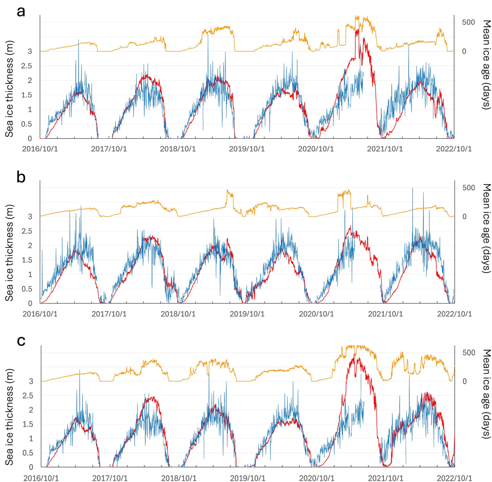
Figure 7. Time series of sea ice thickness and mean ice age at three mooring sites. Panels show data from (a) site A, (b) site B, and (c) site D, corresponding to the locations marked in Fig. 1a. Blue lines indicate sea ice thickness observed by ULS, red lines show estimated sea ice thickness, and orange lines represent the mean sea ice age. The time period is from 1 October 2016 to 1 October 2022. Left vertical axes indicate sea ice thickness, and right vertical axes indicate mean sea ice age.
