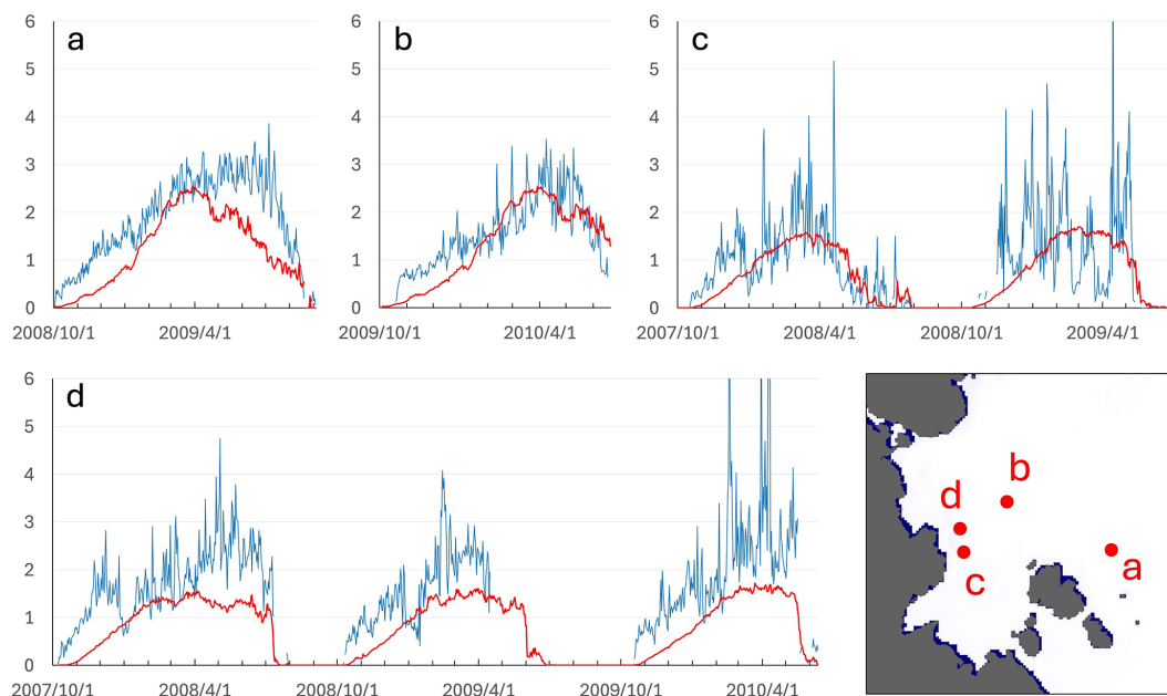
Figure 9. Time series of daily sea ice thickness observed by four ADCP moorings in the Laptev Sea (blue lines) and the corresponding thickness estimated using our method (red lines). Panels (a)–(d) show data from the four mooring sites. The map in the lower-right panel provides a close-up view of the Laptev Sea and indicates the locations of the ADCP moorings.
