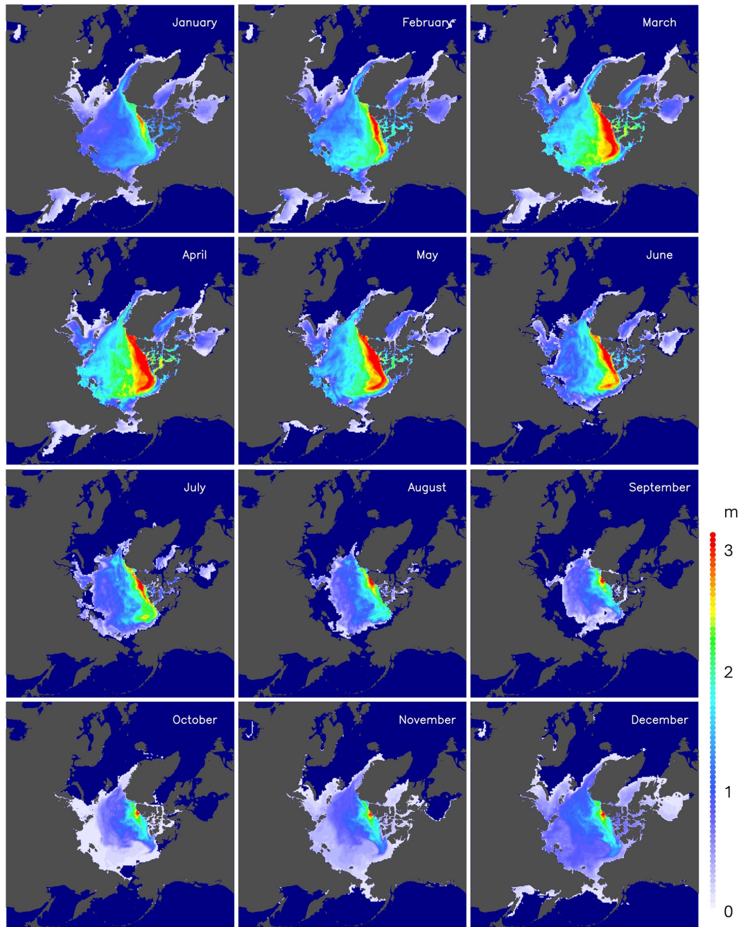
Figure 12. Monthly mean sea ice thickness for each month of 2021.
