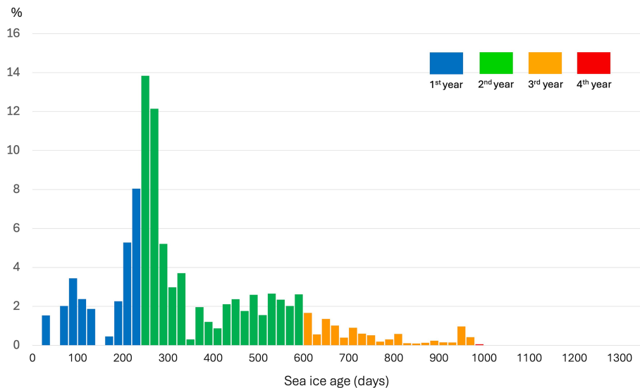
Figure 4. Sea ice age distribution on 31 May 2021. The horizontal axis shows sea ice age in 20 d intervals, and the vertical axis represents the percentage of total sea ice area. Colors indicate the formation period: red for ice formed before 10 September 2018, orange for 10 September 2018–10 September 2019, green for 10 September 2019–10 September 2020, and blue for after 10 September 2020.
