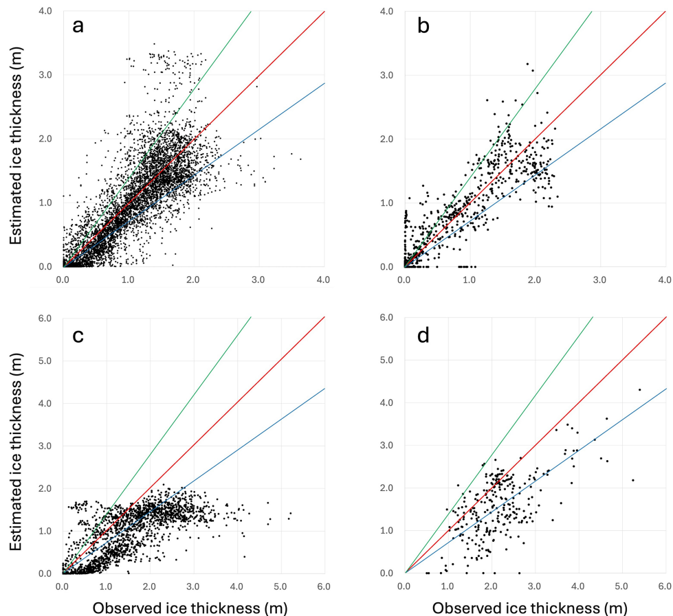
Figure 10. Scatter plots comparing the estimated sea ice thickness with observations from four different datasets. (a) Comparison with ULS observations in the Beaufort Sea (sites A, B, and D in Fig. 1a); (b) comparison with ULS observations in the Fram Strait (star in Fig. 1a); (c) comparison with ADCP observations in the Laptev Sea (red dot in Fig. 1a); and (d) comparison with EM observations (blue dot in Fig. 1a). The horizontal axes represent the observed ice thickness, and the vertical axes represent the corresponding estimated ice thickness. The red, blue, and green lines indicate results with scaling factors of 0.25, 0.35, and 0.15, respectively.
