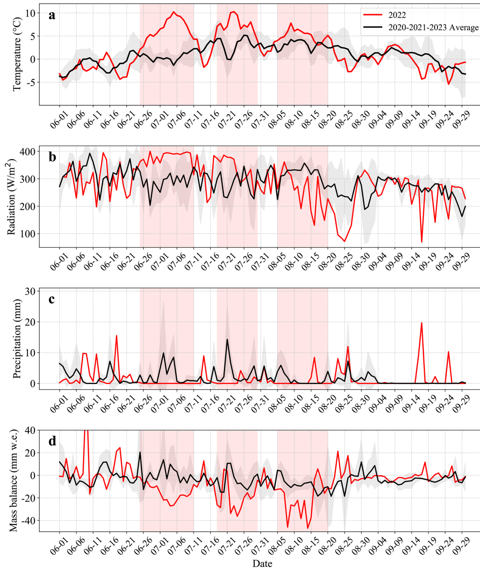
Figure 7. Comparison of daily air temperature (a), daily incoming shortwave radiation (b), daily precipitation (c) and daily glacier-wide mass balance (d) at the Kangxiwa Glacier during the ablation season (June–September), showing the difference between 2022 and the other three years. The grey line shows the average for 2020, 2021 and 2023 with standardized variation (grey shaded area), while the red line shows the records for 2022. Light red rectangles highlight three heatwave events. The meteorological data was derived from the AWS4900.
