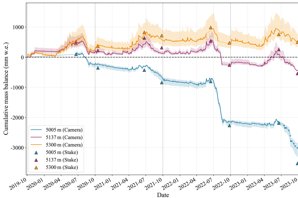
Figure 3. Comparison of the cumulative mass balance estimated using time-lapse cameras (lines) and the glaciological methods (triangles) at the three locations (5005, 5137 and 5300 m) on the Kangxiwa Glacier. The thin dotted lines denote gap-filled data.
