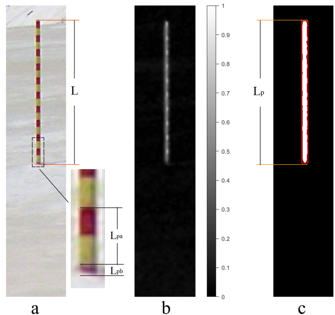
Figure 2. Illustration of image processing workflow. (a) Original image with a frame and a zoomed inset of the coloured stake bottom. (b) Grayscale representation of the S channel from the HSV colour space; (c) calibration stake contour with a red minimum bounding rectangle.
