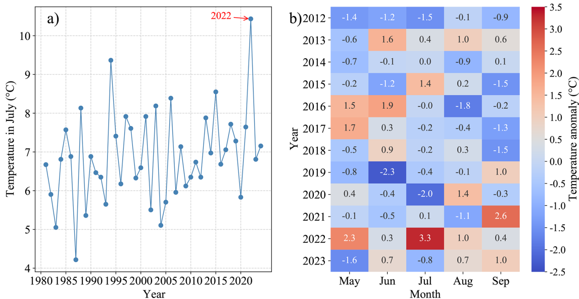
Figure 6. Variation of mean ERA5 air temperature in July at the corresponding grid point of Kangxiwa Glacier during the period from 1981 to 2024 (a) and heatmap of monthly air temperature anomaly from May to September during 2012–2023 recorded by AWS4900 (b).
