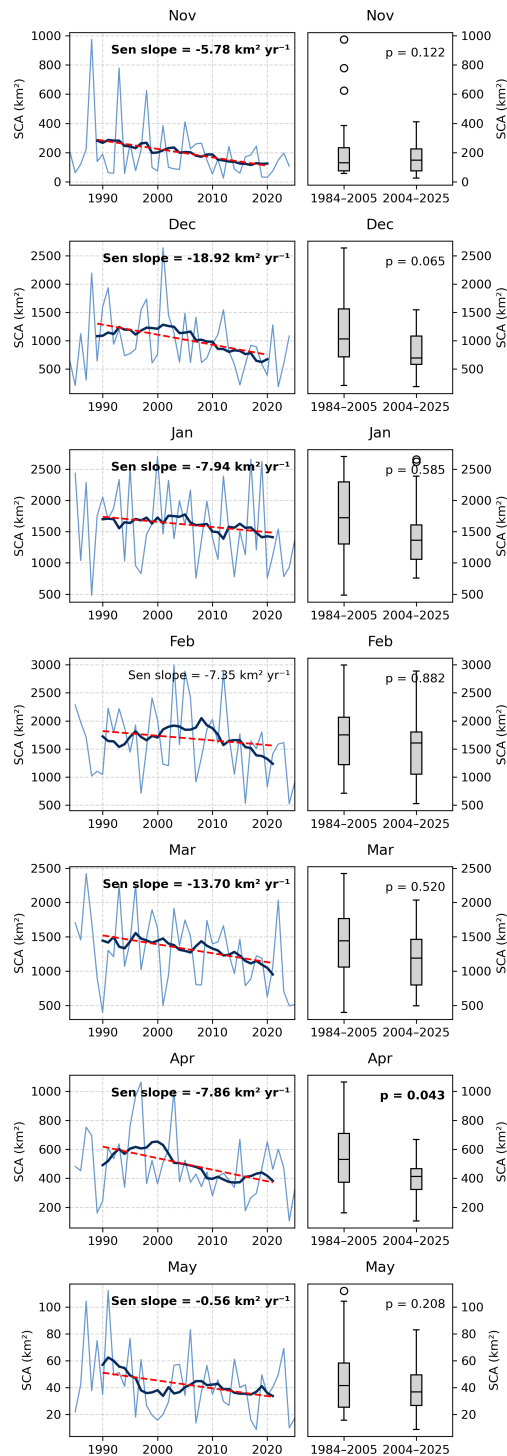
Figure 7. Yearly SCA time-series (light blue lines), 10 year-smoothed SCA (dark blue lines), and overall trends (dashed red lines), along with differences in variability between two 21 year sub-periods across the entire study area. Bold text indicates statistically significant trends (line chart: Mann-Kendall/Sen's slope) and significant differences in variability (boxplot: Levene's test). Massif-level trends and variability differences are shown in Figs. A5 and A6.
