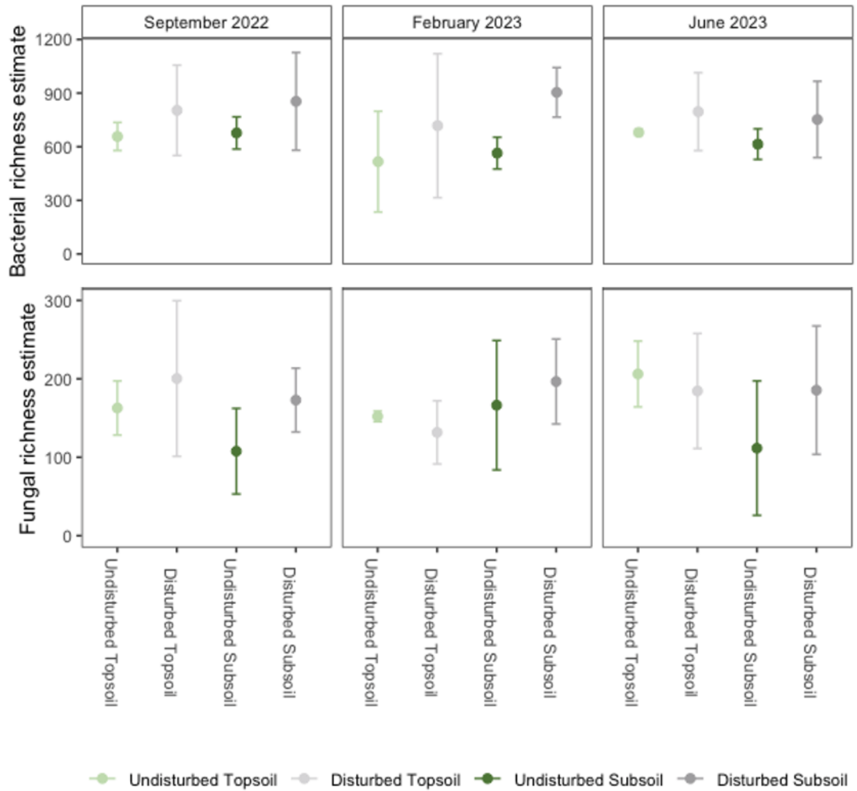
Figure S8. ASV richness estimates across disturbance regimes, soil layers, and sampling dates. Richness was estimated using the weighted linear regression model of OTU richness estimates, which weights observations based on variance. Error bars represent \pm 1.96 SE.
