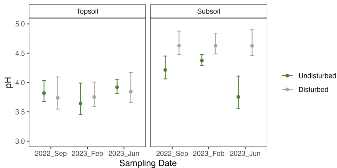
Figure S5. Soil pH, by disturbance and sampling date, faceted by soil layer. pH was significantly higher in the subsoil layer for the disturbed treatment compared to the undisturbed treatment ( p < 0.01 ; ANOVA). Error bars are standard error.
