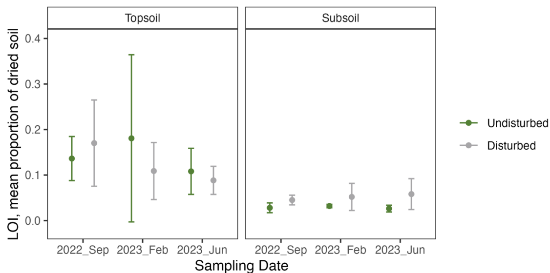
Figure S4. Loss on ignition (LOI), a proxy for soil organic matter content) by disturbance treatment and sampling date, faceted by soil layer. Error bars are 95% confidence intervals ( 1.96 \times standard error).
