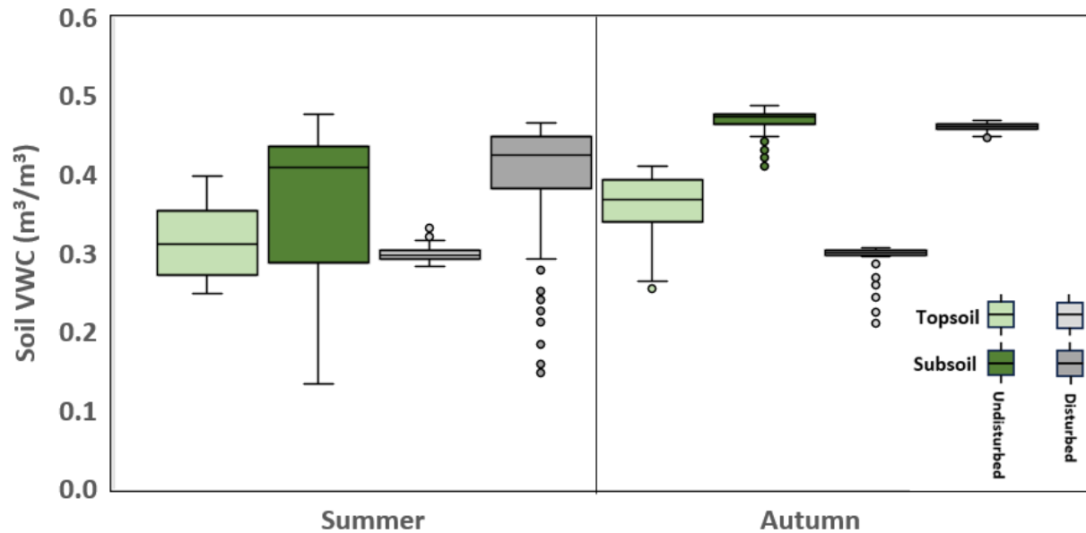
Figure S3. Summer and autumn soil VWC patterns. VWC measurements were restricted to the summer (Jun–Aug) and autumn (Sep and Oct) seasons due to the sensors' operational constraints, which required temperatures to remain above freezing. Soil VWC are average daily values from the topsoil and subsoil layers at the 8 chamber plots: 4 at the undisturbed site and 4 at the disturbed site. The boxplot range indicates the first and third quartiles; the middle line denotes the median. Box whiskers indicate minimum and maximum values, excluding outliers indicated by circles.
