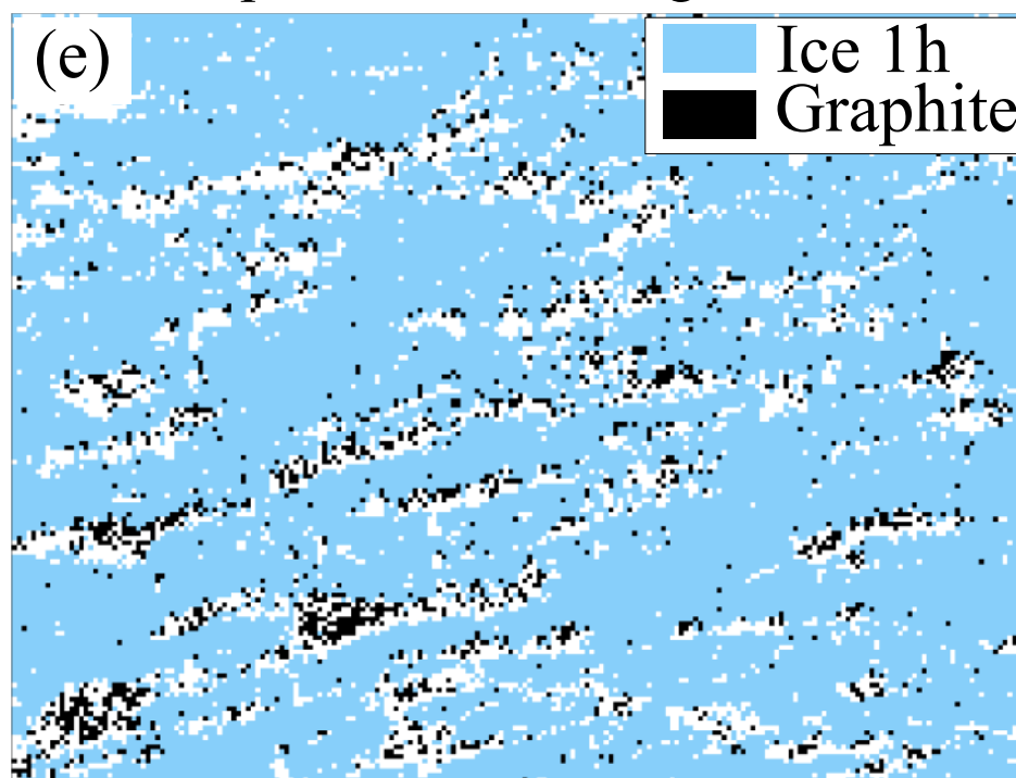
Ice phase combined with processed EDS signal
