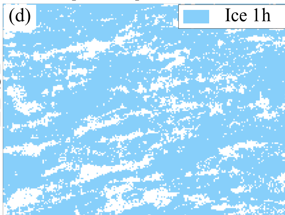
Raw phase map from EBSD
