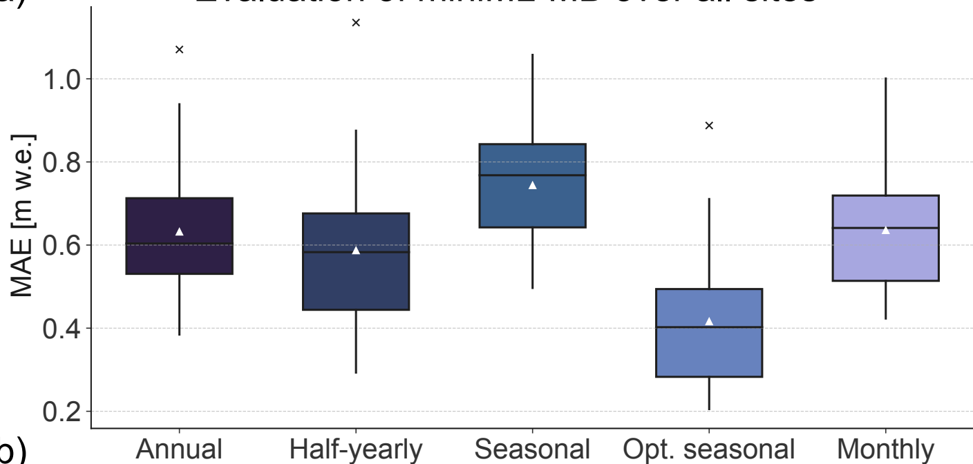
(a) Evaluation of miniML-MB over all sites
