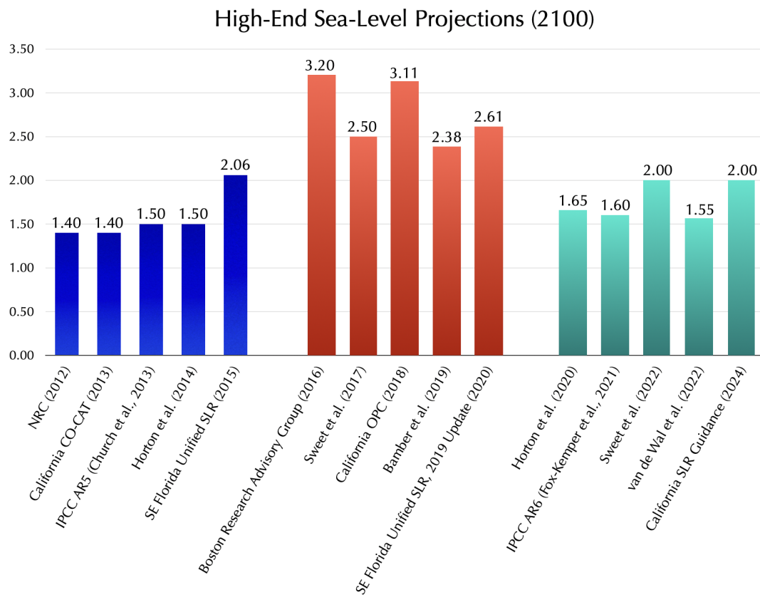
Figure 1. High-end projections for sea-level rise (m) by 2100, arranged chronologically: (1) community assessments and practitioner-oriented reports published before 2016 (blue), (2) reports and assessments published in 2016–2020 (red), and (3) recent reports and assessments (green). The recent reports gave less weight to DP16 and MICI than the 2016–2020 reports; Sweet et al. (2022) and California Sea Level Rise Guidance (2024) included MICI but at a reduced rate, while the other three recent assessments excluded MICI. Most projections are for global sea-level rise, although some jurisdictional reports (e.g., the 2016 Boston and 2018 California reports) include regional effects. The California OPC (2018) value is for the San Francisco tide gauge. The AR6 value is the 95th percentile upper bound based on medium-confidence processes. The van de Wal et al. (2022) value is the upper value in their high-end range, assuming perfect correlation between components. Baseline dates vary but typically are around the year 2000. All reports are cited in the text except for National Research Council (2012), Coastal and Ocean Working Group of the California Climate Action Team (CO-CAT) (2013), and Southeast Florida Regional Climate Change Compact Sea Level Rise Work Group (Compact) (2015).
