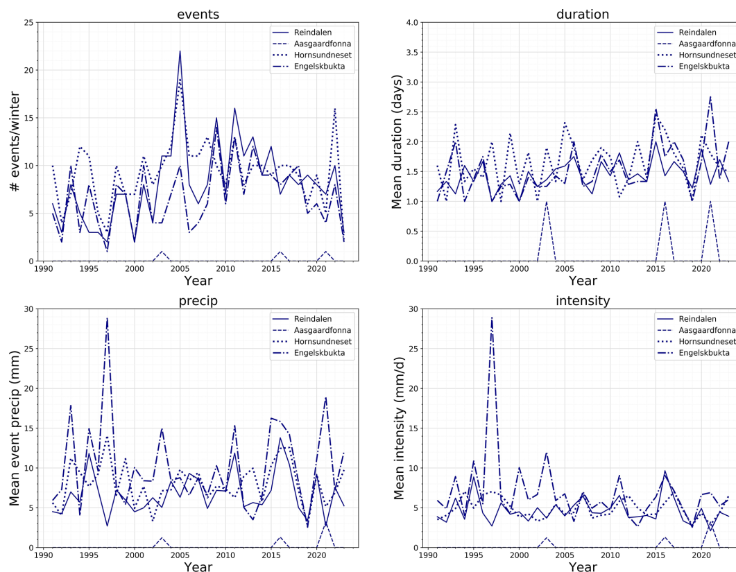
Figure A1. Time series of the ROS characteristics (number of events, mean duration, mean total precipitation and mean intensity) shown for four contrasting sites across Spitsbergen; Reindalen (77.98° N, 16.07° E), Åsgårdfonna (79.61° N, 16.61° E), Hornsundneset (76.88° N, 15.57° E) and Engelsbukta (78.84° N, 11.98° E). The coordinates correspond to one point within each area and are not exact coordinates for each site.
