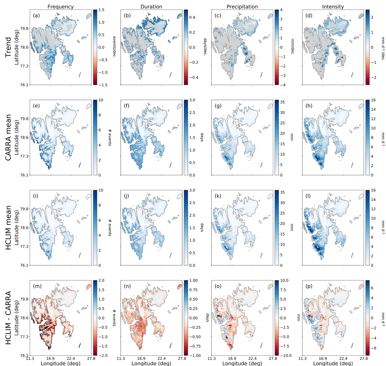
Figure 2. Present day trends derived from the CARRA dataset (a–d) and climatology of ROS frequency, duration, total precipitation per event, and mean intensity for 2000–2020 (e–h). Trends are obtained for the entire CARRA period (1991–2023). ROS climatology for 2000–2020 obtained with HCLIM-ERA5 at 2.5 km resolution (i–l) and the differences between HCLIM-ERA5 and CARRA (m–p).
