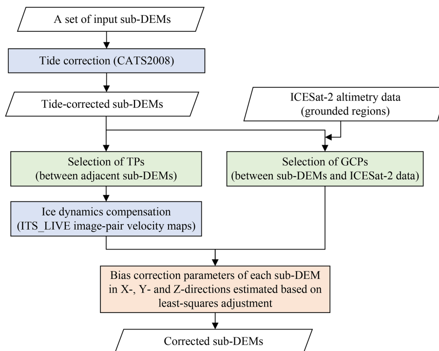
Figure 2. Data processing principle of the multi-temporal DEM adjustment model (MDAM).
