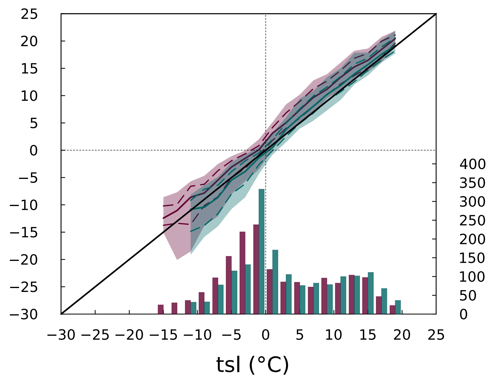
UKESM1-0-LL
