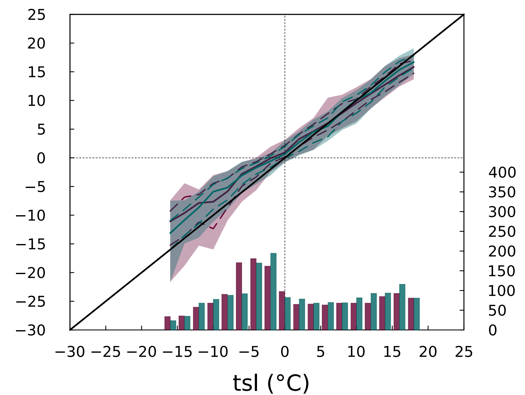
IPSL-CM6A
