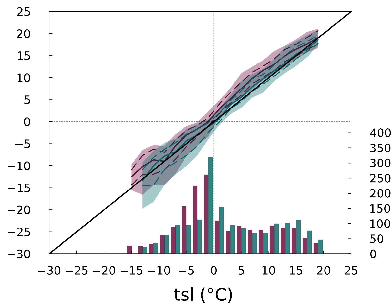
UKESM1-0-LL
