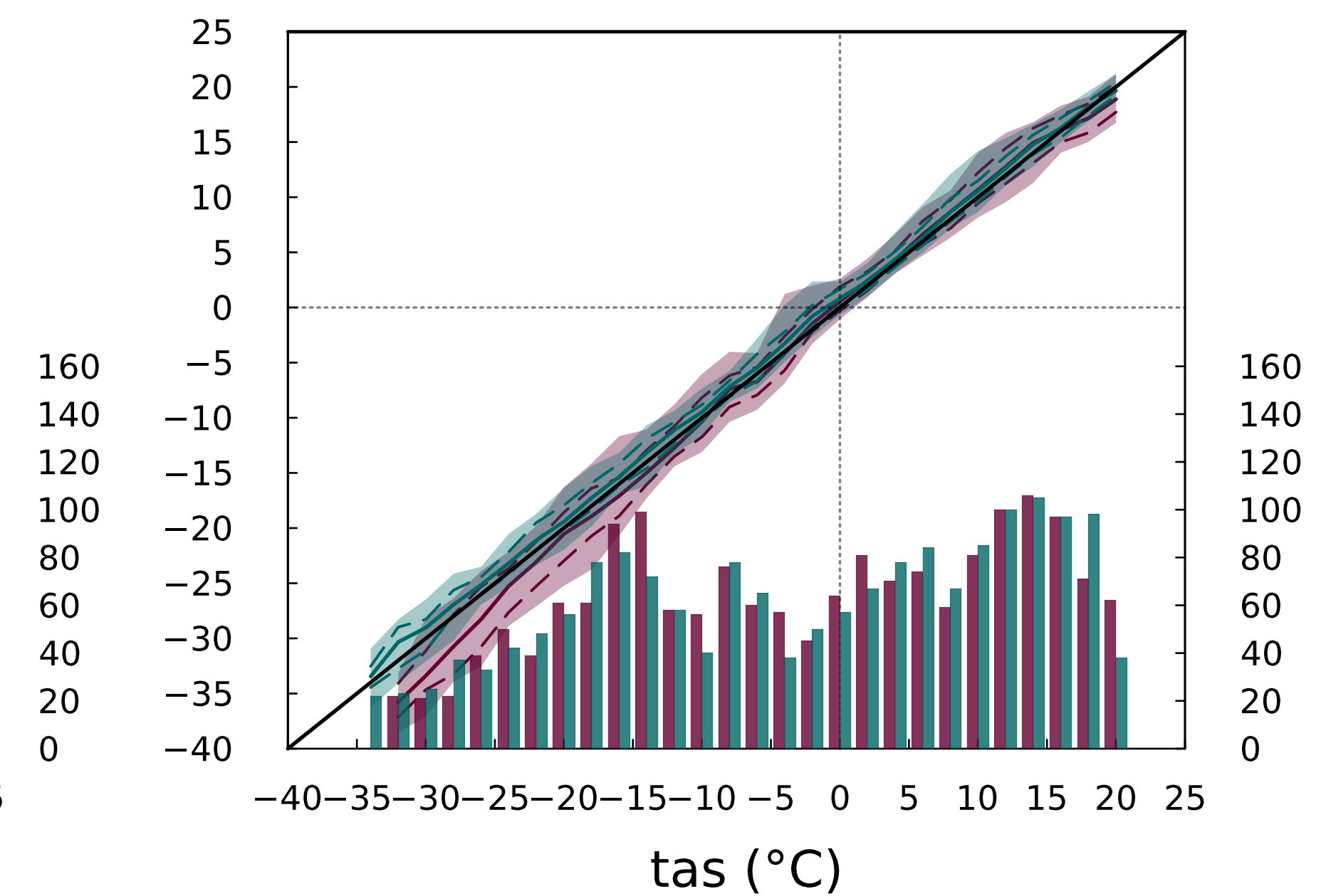
IPSL-CM6A
