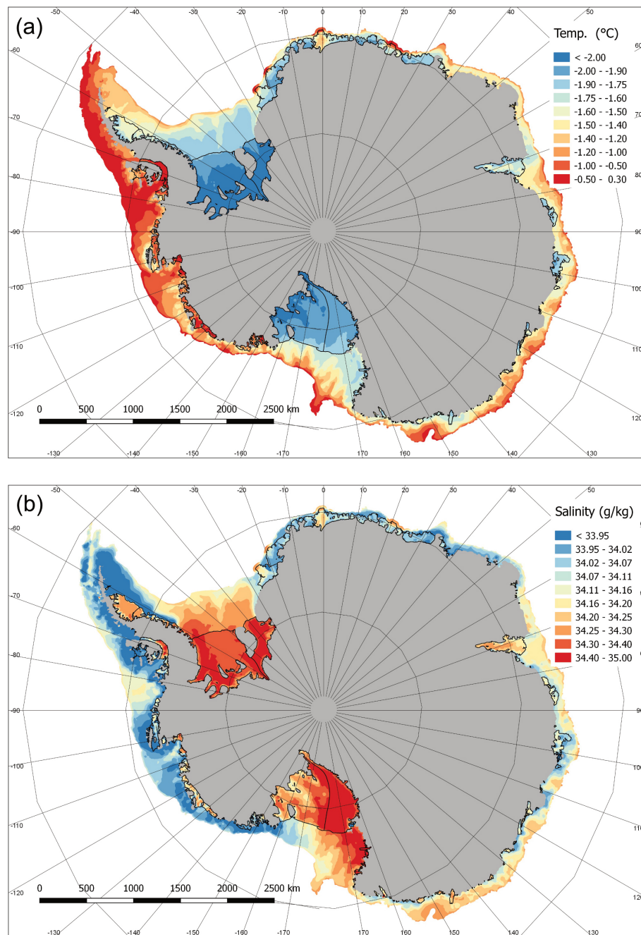
Figure 4. Column-averaged oceanographic properties for the continental shelf region, including the sub-ice-shelf ocean cavities, for (a) temperature and (b) salinity.
