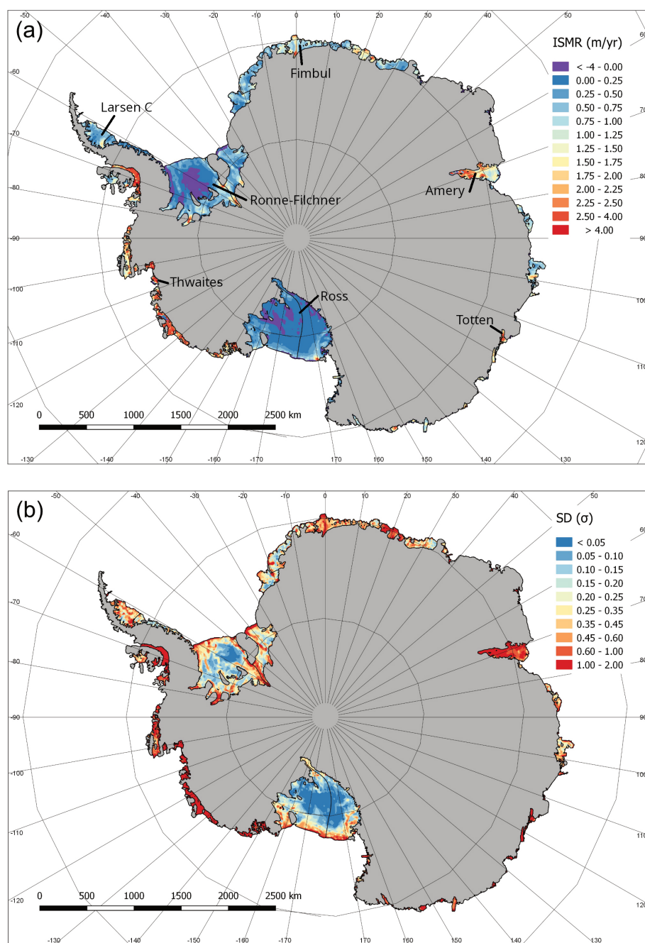
Figure 1. Multi-model mean of ice shelf (a) melt rate (ISMR), and (b) standard deviation (SD) in melt rate.
