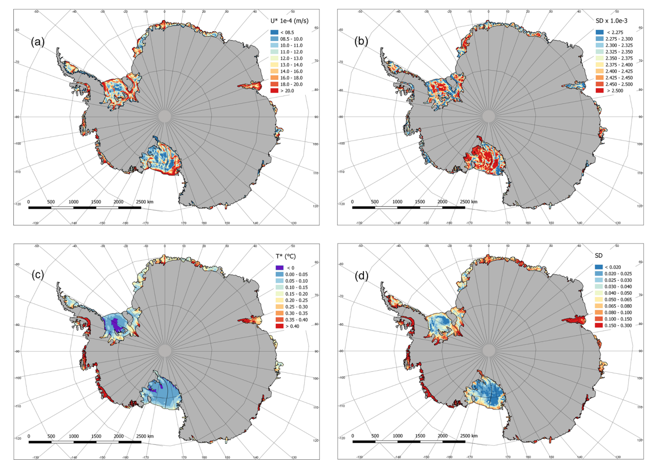
Figure 2. Multi-model mean of (a) friction velocity ( u^* ), (b) standard deviation in u^* , (c) thermal driving ( T^* ), and (d) standard deviation (SD) in thermal driving.
